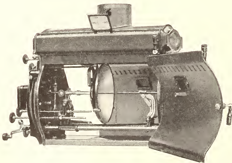
Figure 3.—Interior view of lamphouse.
