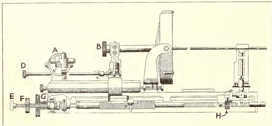
Diagram of parts of Sterling Suprex lamp mechanism. See text.
