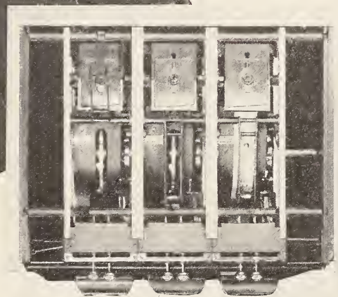
Three Unit NEW 1935 MODEL H ALL PURPOSE REGISTER with top plate removed showing mechanism.
