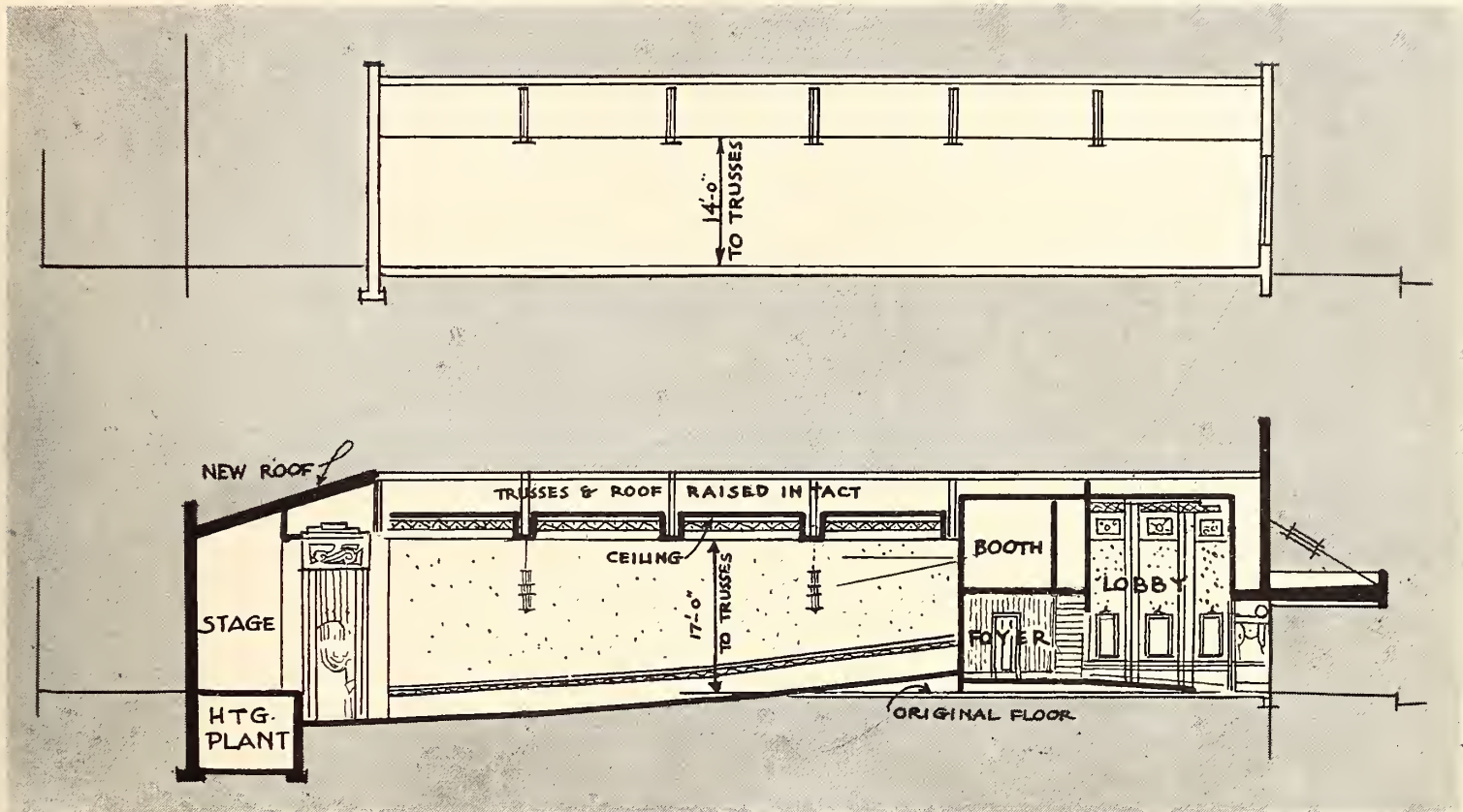
Author's sketches showing in cross section the changes made in the original building (upper sketch) at the ceiling, floor and elsewhere.
