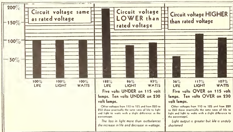
Chart comparing life and illumination efficiency of incandescent lamps at varying voltages.
