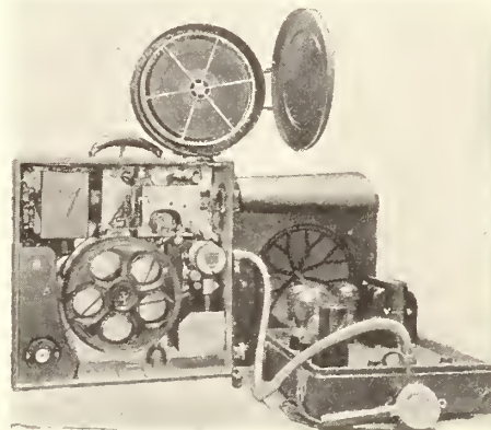
DeVry portable sound projector.
