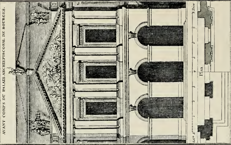
FRONTISPIÈCE OF ARCHBISHOP'S PALACE AT BOURGES. BULLET (see p. 142) (FROM J. F. BLONDEL, "COURS D'ARCHITECTURE," VOL. VIII)
