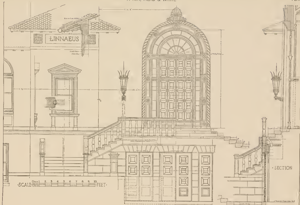
DETAILS OF GARDEN ELEVATION
