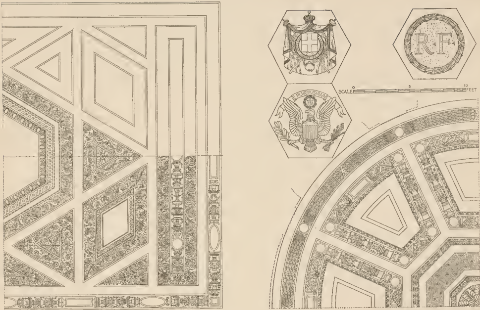
DETAILS OF PLASTER CEILING
