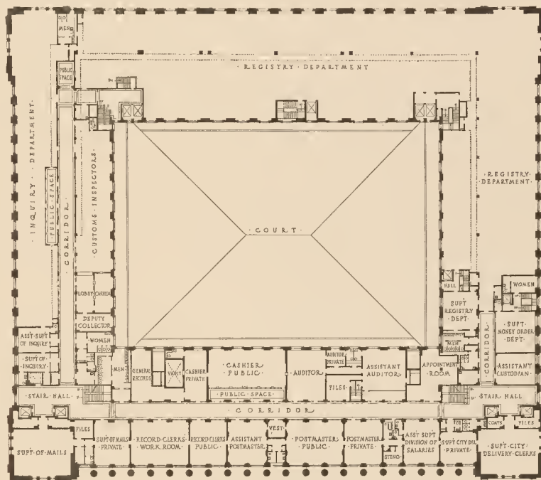
SCALE 0 10 20 30 40 50 60 70 80 90 100 FEET. SECOND FLOOR PLAN
