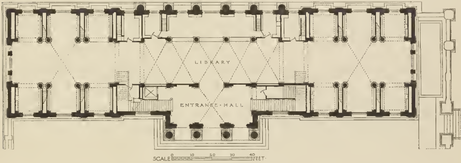
KENT HALL, PLAN OF FIRST FLOOR 1910
