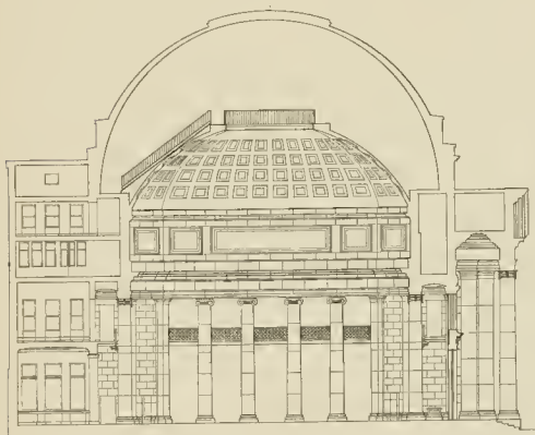
SCALE 0 5 10 15 20 25 FEET SECTION
