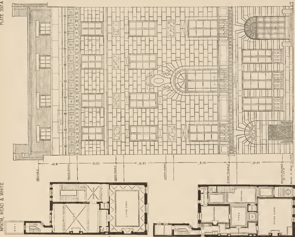
FRONT ELEVATION SCALE 0 5 10 20 FEET
