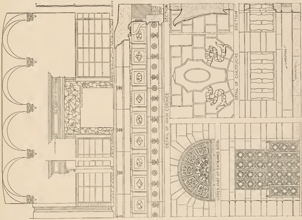
EXTERIOR DETAILS AND DETAIL OF LIVING ROOM SCALE 0 1 2 3 FEET
