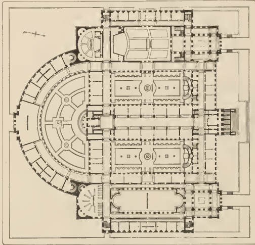
BASEMENT PLAN
