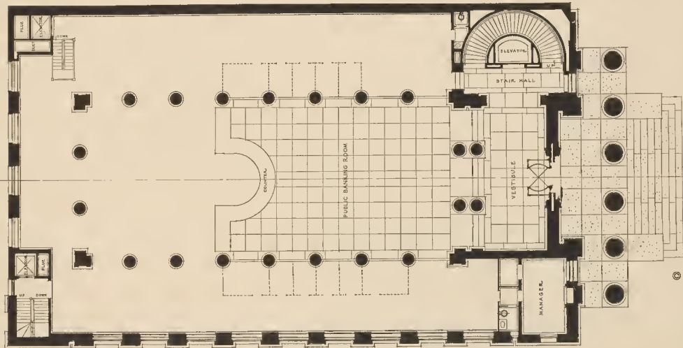
PLAN THE BANK OF MONTREAL, WINNIPEG BRANCH 1911
