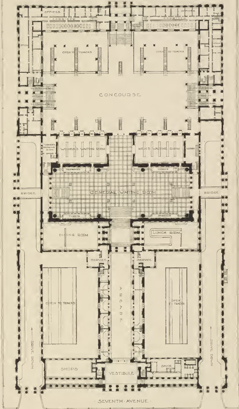
BLOCK PLAN THE PENNSYLVANIA RAILROAD STATION, NEW YORK CITY. 1906 - 1910
