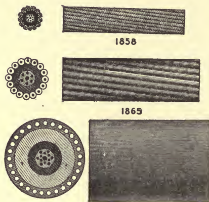
TYPES OF CABLES USED SINCE 1858.
