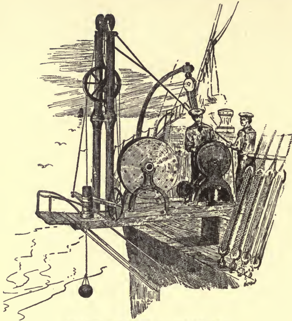
SOUNDING MACHINE ON A CABLE STEAMER.
