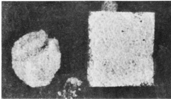
Marble fragment, spot-cleaned by a single, brief pulse of laser energy, reveals its pristine color and texture. The technique is so precise it can be controlled so that only recent encrustations are removed while the natural patina of old stone remains unharmed. Even stone that has been seriously weakened (to a structural strength equivalent to that of a sugar cube, for example) is not further weakened by laser cleaning.
