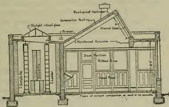
CROSS SECTION
