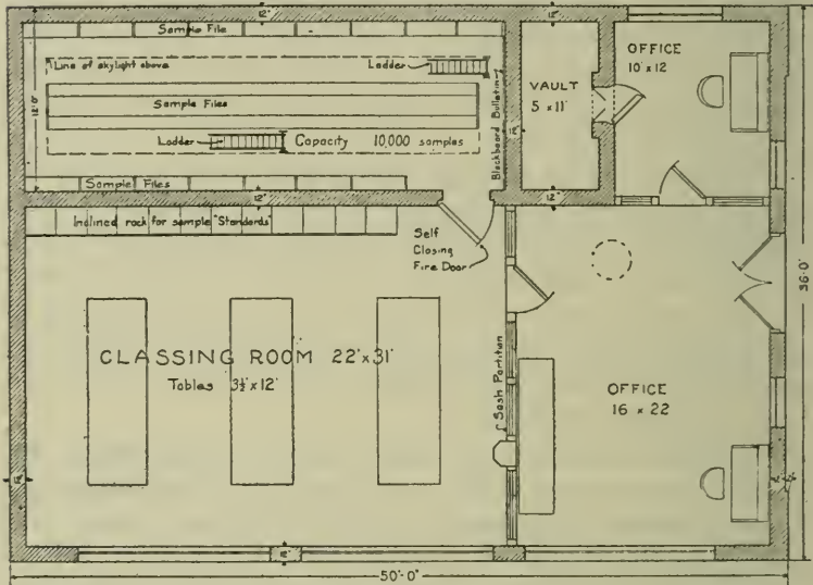
FLOOR PLAN
