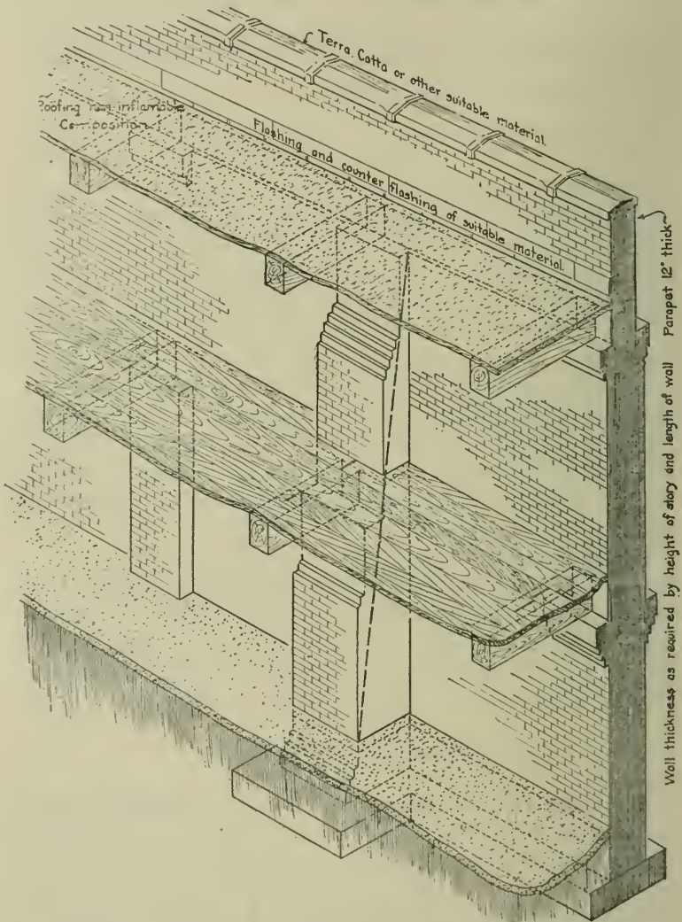
FIG. 27.—Timbers supported by plasters, corbels, or offsets and self-releasing. Note the buttress (in the foreground) used for bracing long walls.
