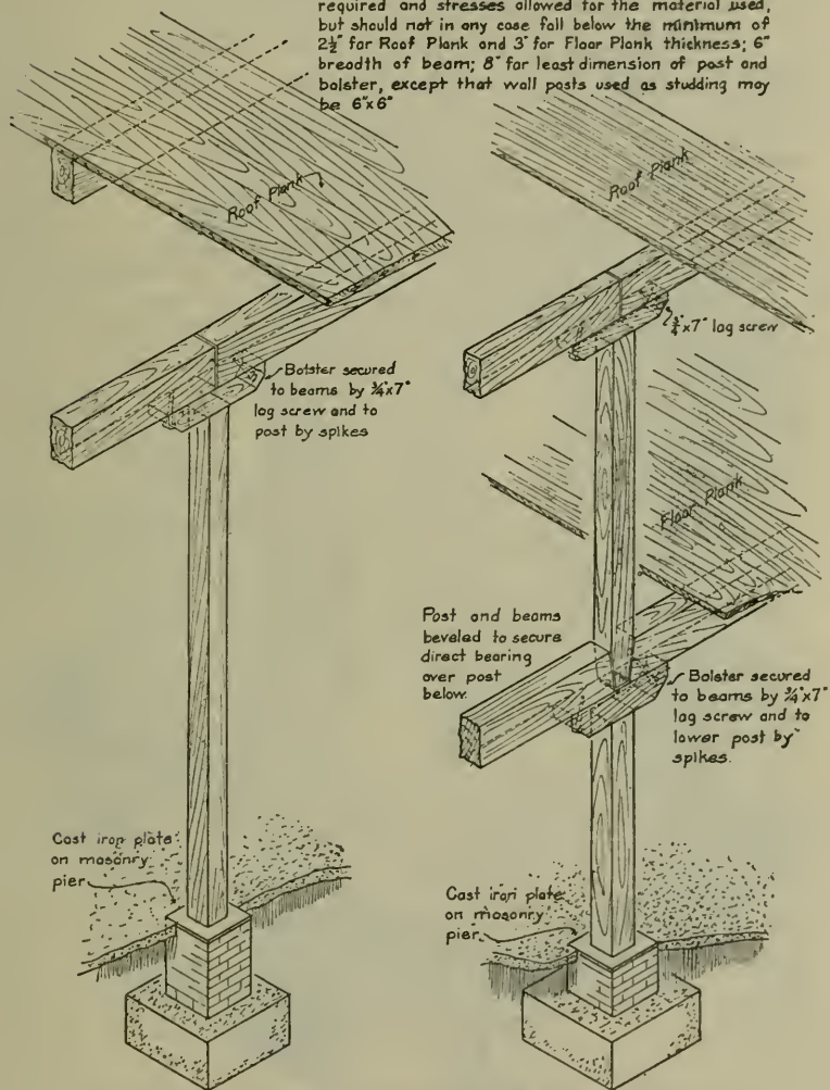
FIG. 28.—An economical method of framing posts and timbers.
