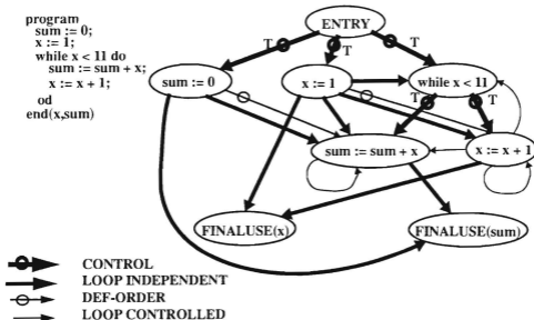
Figure 3.2: Example of a Program Dependence Graph [Ref. 28]
