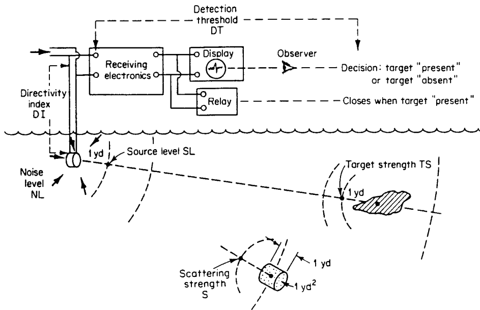
Figure 1: Diagram Showing Sonar Parameters (Urick)
