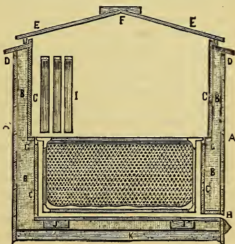
DIAGRAM OF CHAFF HIVE.*
