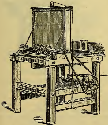
GRAY'S IMPROVED MACHINE FOR MAKING SECTIONS.
