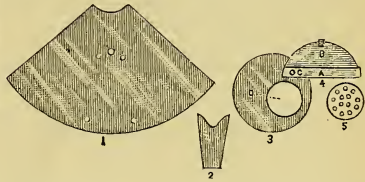
THE TINWORK USED FOR COLD-BLAST SMOKER.
