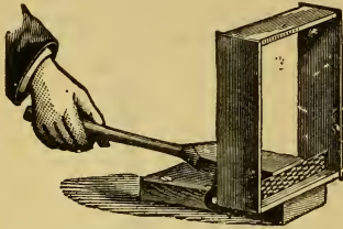
PARKER MACHINE FOR FASTENING STARTERS IN SECTIONS.
