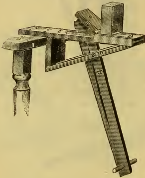
GRAY'S MACHINE FOR FASTENING STARTERS IN SECTIONS.
