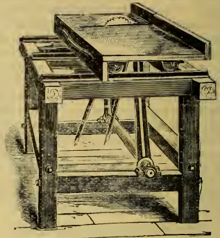
A SAW-TABLE FOR CUTTING OFF STUFF.
