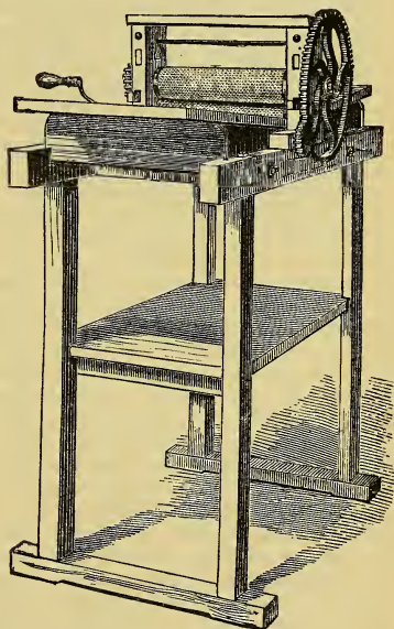
ORIGINAL FOUNDATION-MACHINE WITH 12-IN. ROLLS.
