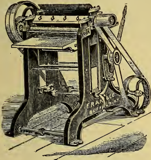
18-INCH GEM PLANER.
