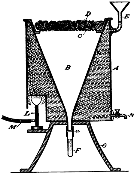
FIG. 86. — THE BERLESE COLLECTING TRAP: A , EXTERIOR RECEPTACLE CONTAINING WATER; B , INTERIOR FUNNEL; C , VESSEL HAVING THE BOTTOM OF METALLIC NETWORK; D , SUBSTANCE FOR EXAMINATION; E , FUNNEL FOR INTRODUCING THE WATER; F , SMALL GLASS TUBE CONTAINING ALCOHOL, WHERE THE INSECTS ARE COLLECTED, THIS BEING CONNECTED TO THE APEX OF THE FUNNEL BY A SHORT TUBE ( a ) OF INDIA RUBBER; G , FEET SUPPORTING THE APPARATUS; L , LAMP FOR HEATING; M , INDIA RUBBER TUBE FOR CARRYING OFF THE GAS; N , FAUCET FOR DISCHARGE.
