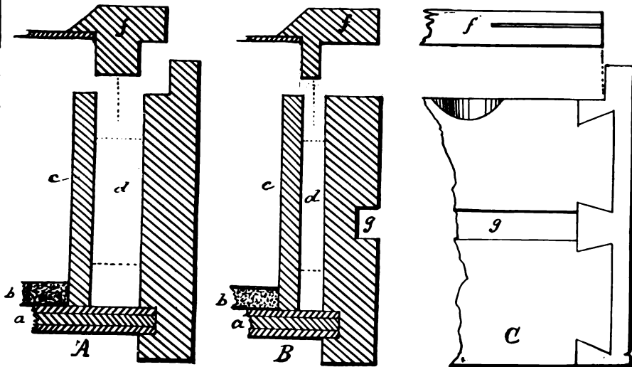
FIG. 166.—CONSTRUCTION OF THE INSECT CABINET DRAWER OF THE U. S. NATIONAL MUSEUM: A, CROSS-SECTION OF FRONT; B, SAME OF SIDE; C, VIEW OF FRONT END OF SIDE, TWO-THIRDS NATURAL SIZE. a, BOTTOM; b, CORK LINING; c, INSIDE STRIP FORMING NAPHTHALENE POISON CHAMBER; d, NAPHTHALENE POISON CHAMBER; f, TOP; g, GROOVE.
