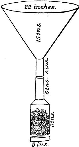
FIG. 87.—THE GILLETTE TRAP LIGHT.
