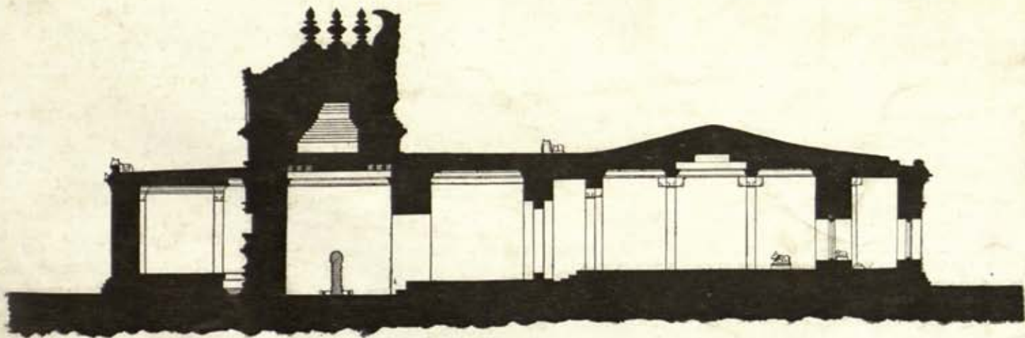
(b) SECTION. A-B
