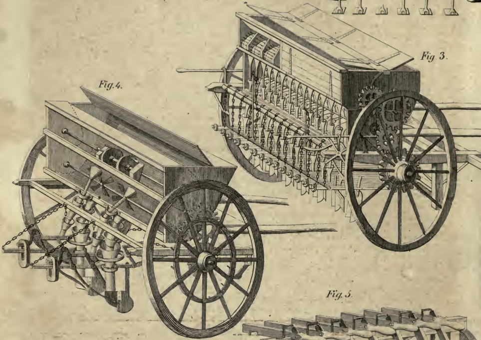
Drill Hopper for Bone Dust
