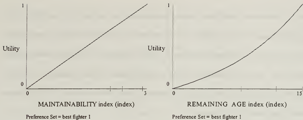
Figure 11. Forms of Single Utility Functions Used in LDW Modernization Model
