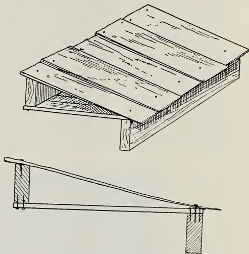
BLAISDELL'S SHADE BOARD AND HIVE-COVER.
