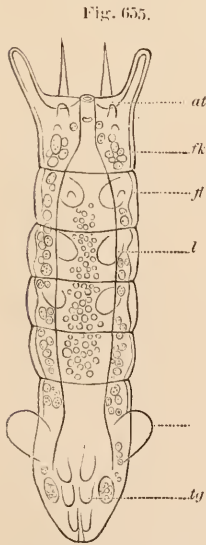
Third larva of Polyneina .
