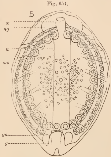
Second larva of Platyaster .
