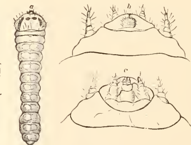
Larva of Callidium angustum .
