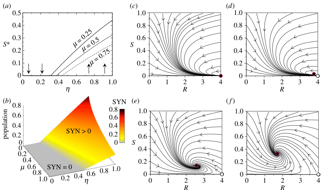
Figure 9. Bifurcations and dynamics of the function-and-die TM with competing microbes. In (a) we display the stationary population of the synthetic strain ( S^* ) against the parameter \eta that weights the efficiency of the resource–microbe interaction. Here we fix \alpha = \sigma = \rho_w = 1 and \delta = 0.25 , using different values of the reversion parameter \mu . We specifically use \mu = 0.25 (thick line), \mu = 0.5 (thin line) and \mu = 0.75 (dashed line). The vertical arrows indicate the stability of the fixed point P_0^* . (b) Survival and extinction phases in the parameter space (\mu, \eta) computed numerically, using the same parameter values of (a). Several phase portraits are displayed setting \mu = 0.25 and (c) \eta = 0.3 < \eta_c = 0.3125 , (d) \eta = 0.34 > \eta_c , (e) \eta = 0.5 and (f) \eta = 0.8 . The internal stable fixed point (black circle highlighted in red) is the fixed point P_2^* . The fixed point P_1^* is not biologically meaningful in the range analysed, since S_1^* > 1 (see electronic supplementary material, Fig. S4). Unstable equilibria are indicated with white circles.
