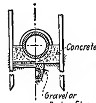
5. Soft Foundation.
