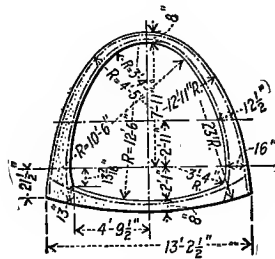
4. Semi-Elliptical Section, Louisville, Ky., Eng. News, Vol. 62, p. 416.
