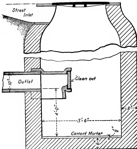
FIG. 34.—CATCH-BASIN.
