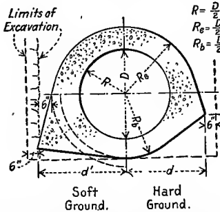
3. Circular Concrete Section in Soft and Hard Ground, Eng. Record, Vol. 59, p. 570,
