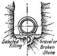
4. Trench in Rock.
