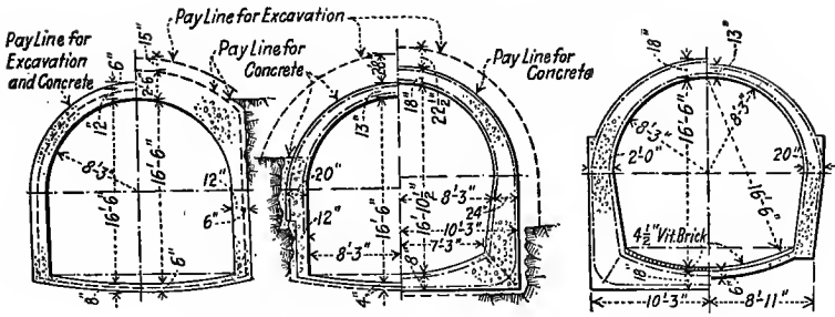
1. Tunnel Sections.
