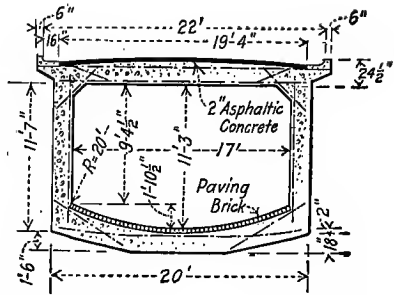
2. Rectangular Section, Omaha, Nebraska, Eng. Contracting, Vol. 46, p. 49.
