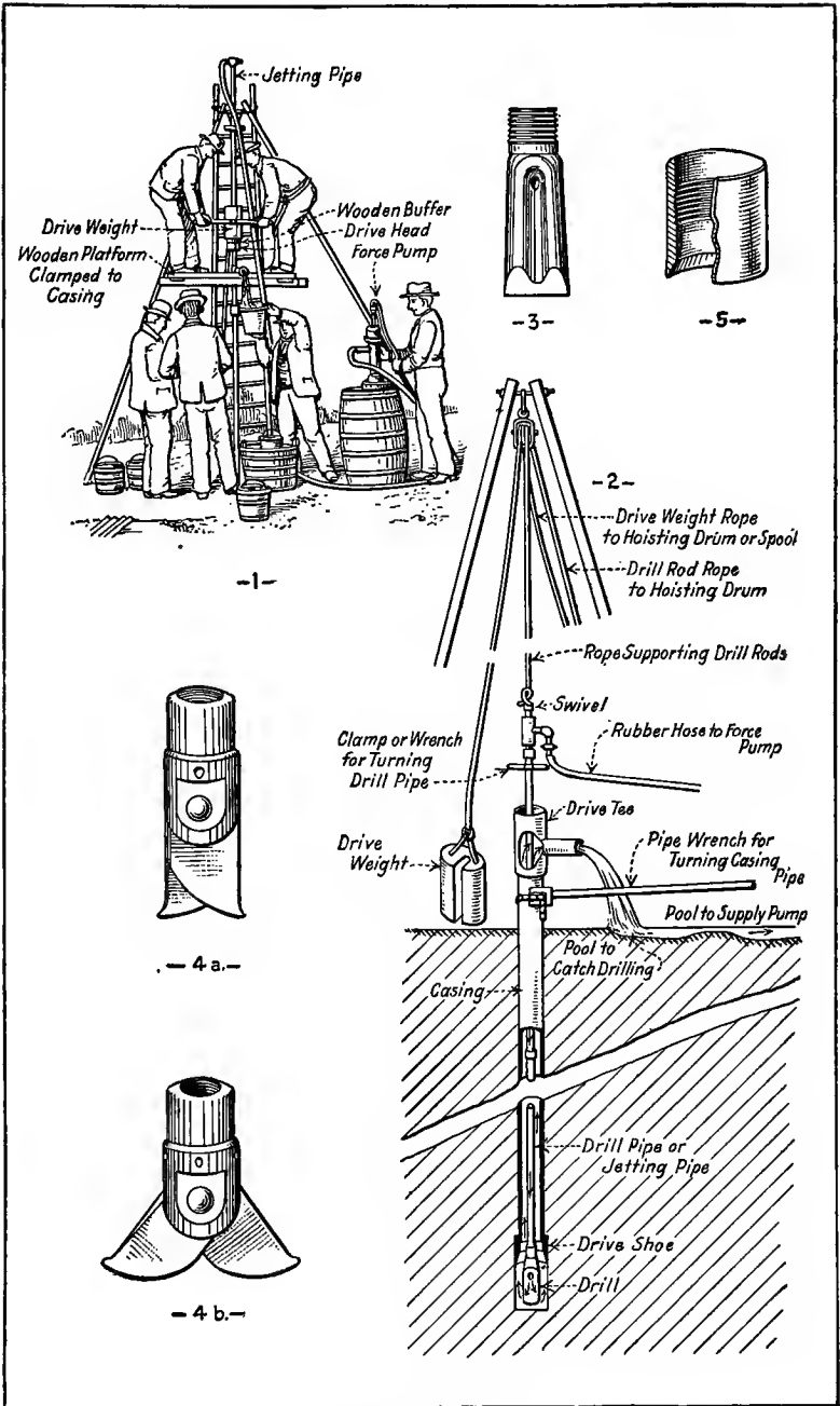
FIG. 7.—Jetting Outfit.
