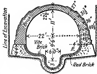
7. Brick and Concrete Sewer showing cunette.
