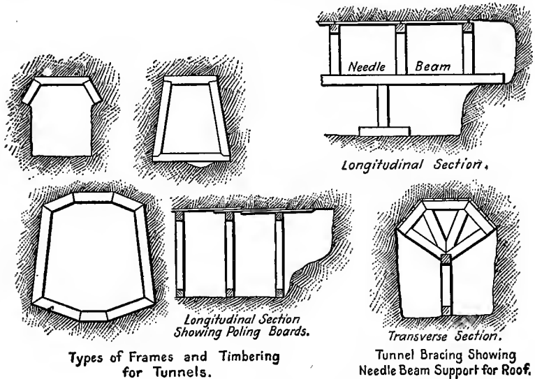
FIG. 116.—Types of Frames and Timbering for Tunnels.
