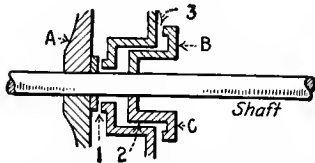
FIG. 57.—Piston Type of Thrust Balancing Device.
