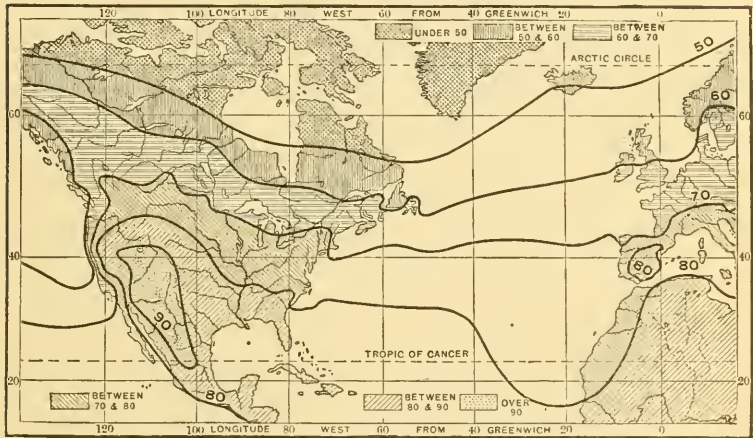
Lines of equal temperature, August
