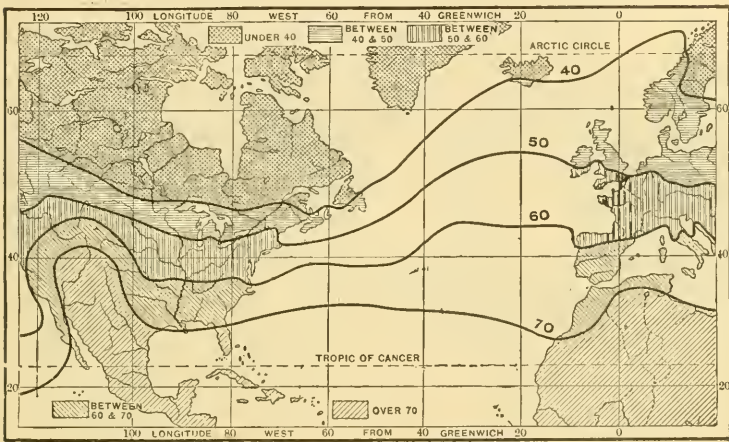
Lines of equal temperature, annual
