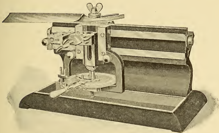
FIG. 3.—Large laboratory microtome (Bausch & Lomb).
