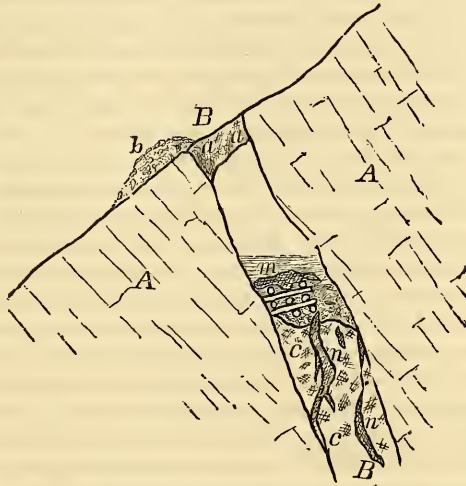
MINNESOTA MINE. Section across the Vein, looking from the easterly quarter. N. 30° W.—B B. Mineral vein dipping north.—A A. Wall rock of compact trap.—a a. Left standing a part of the original surface support to the hanging wall.—m. Mass of copper sustained by timbers.—b. Ancient burrow or spoil bank.—c c. Vein matter embracing masses of copper n n.
