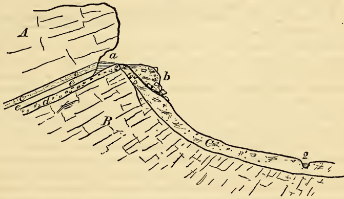
WATERBURY MINE, artificial cavern.—A. Crystalline or greenstone trap, dipping N. 28^{\circ} .—B. Amygdaloid trap.—C. Talus of the bluff and drift.—a. Ancient rock excavation.—b. Rubbish thrown out of a.—d. Conglomerate bed.—c. Jointed chloritic bed.—e. Inclined shaft of Waterbury Company.—2. Little Montreal River or creek.
