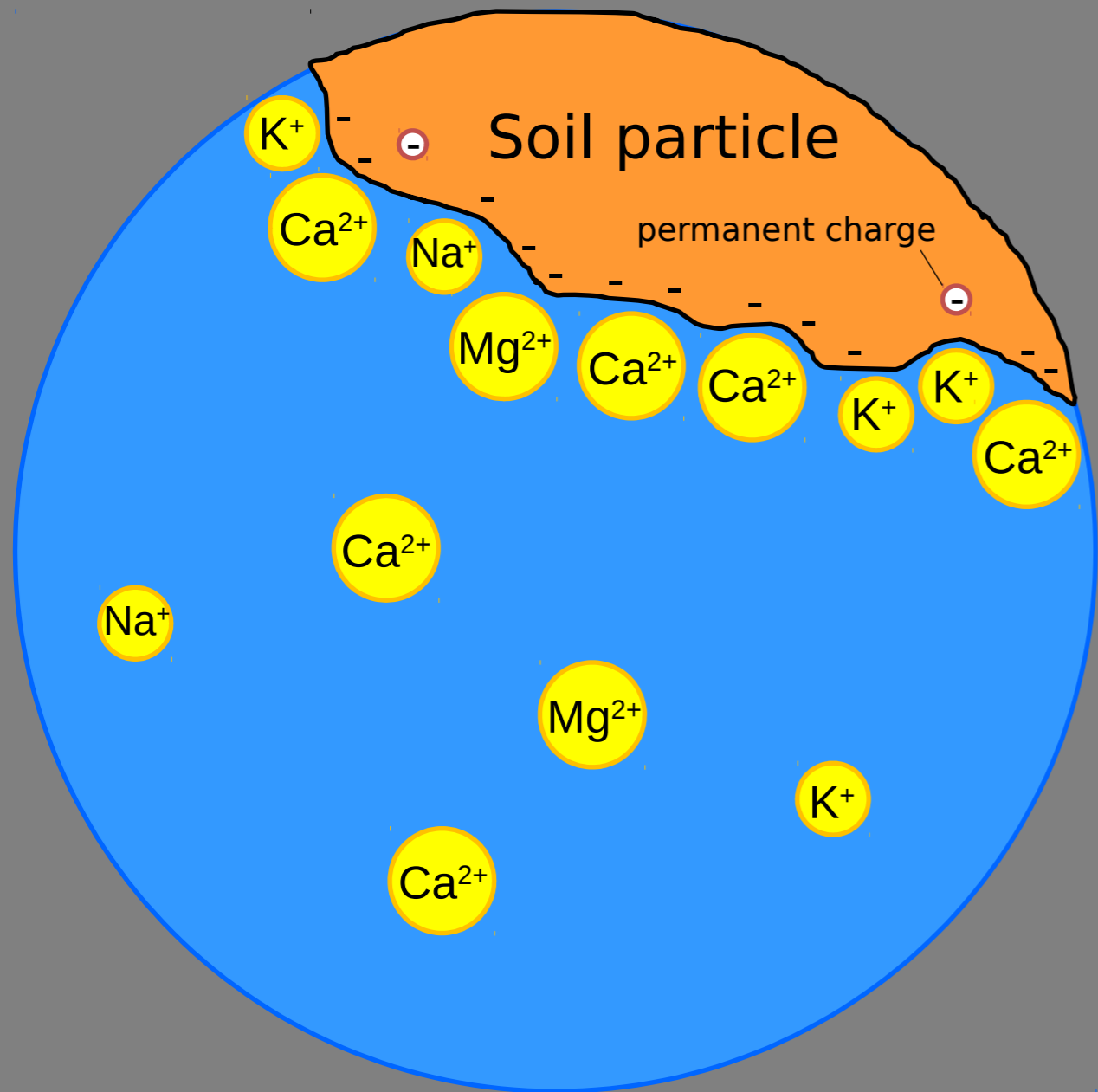
Higher pH
