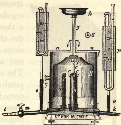
FIG. 19. MOITESSIER'S GAS-PRESSURE REGULATOR.
