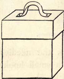
FIG. 9. BOX FOR GLASS PLATES.
