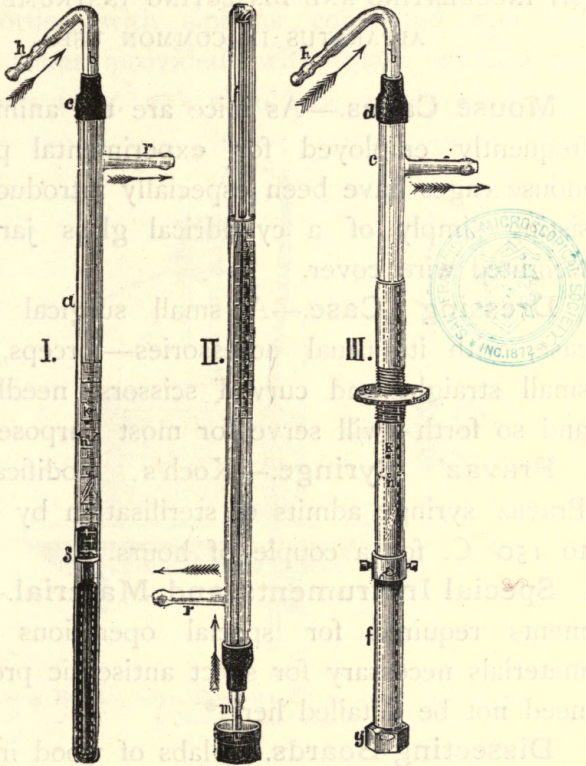
FIG. 23.—MEYER'S THERMO-REGULATOR.
