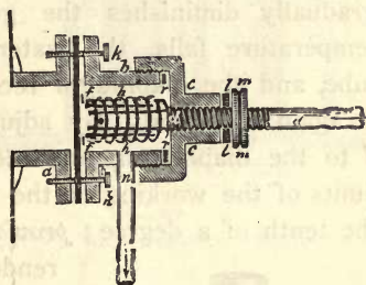
FIG. 17.—SCHLOSING'S MEMBRANE REGULATOR.
