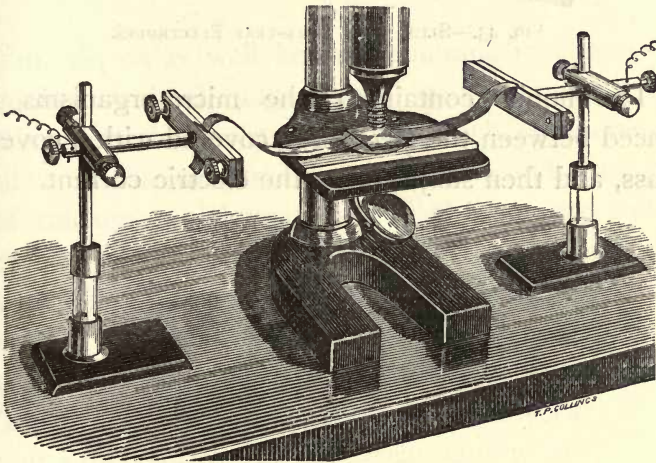
FIG. 42.—APPARATUS ARRANGED FOR TRANSMITTING ELECTRICITY.
