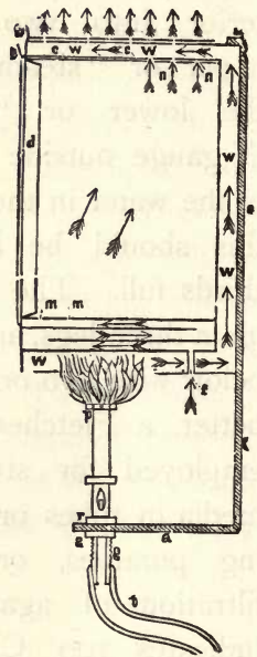
FIG. 3.—SECTION OF HOT-AIR STERILISER.
