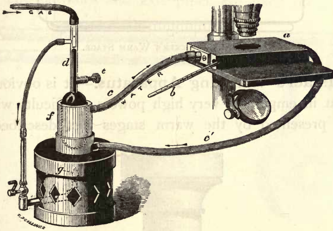
FIG. 33.—SCHÄFER'S WARM STAGE.
