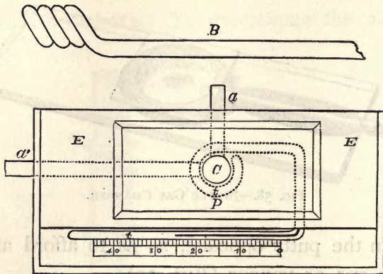
FIG. 40.—STRICKER'S COMBINED GAS CHAMBER AND WARM STAGE.
