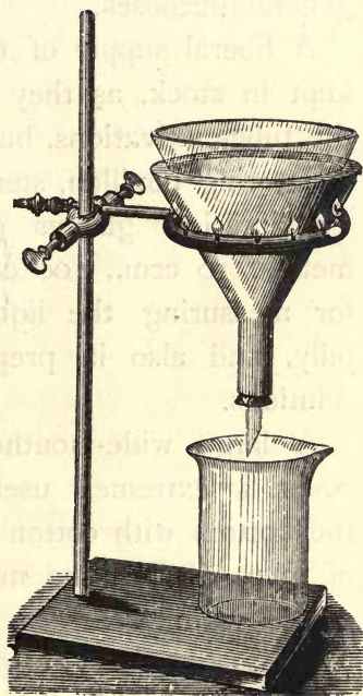
FIG. 4. HOT-WATER FILTERING APPARATUS WITH RING BURNER.
