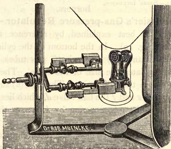
FIG. 20.—Koch's SAFETY BURNER.
