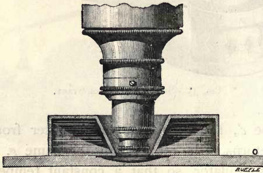
FIG. 35.—SECTION OF ISRAEL'S WARMING APPARATUS AND DROP-CULTURE SLIDE.
