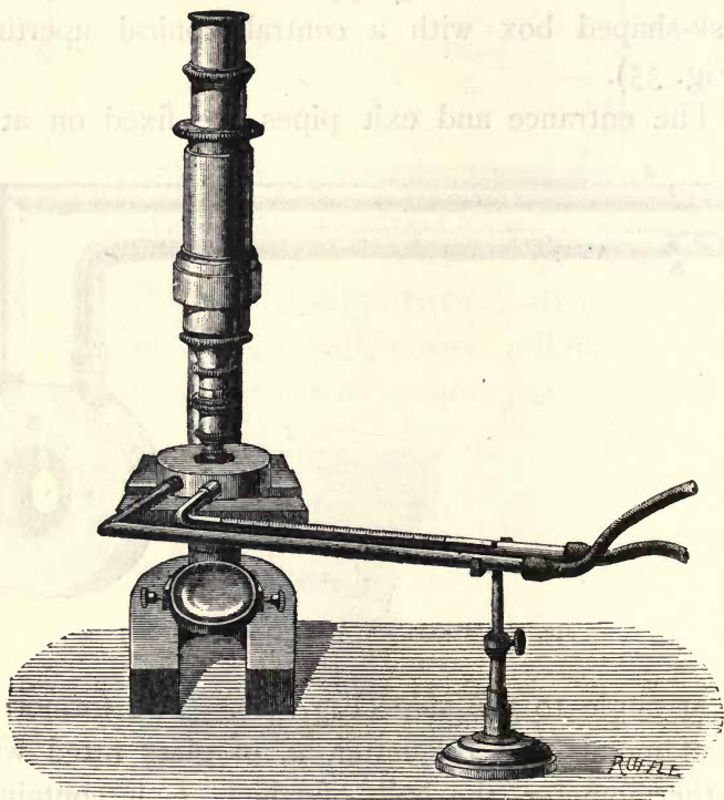
FIG. 37.—ISRAEL'S WARMING APPARATUS IN OPERATION.
