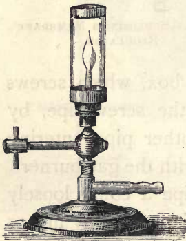
FIG. 18. GAS-BURNER PROTECTED WITH MICA CYLINDER.
