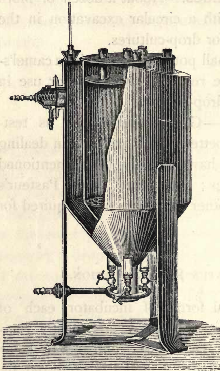
FIG. 16.—D'ARSONVAL'S INCUBATOR.
