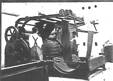
Raising Machine
