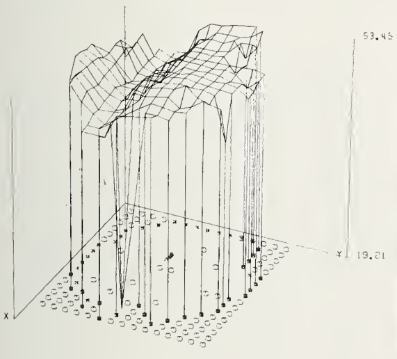
Figure 19. "Three-dimensional" plot of sheet resistance over wafer.
