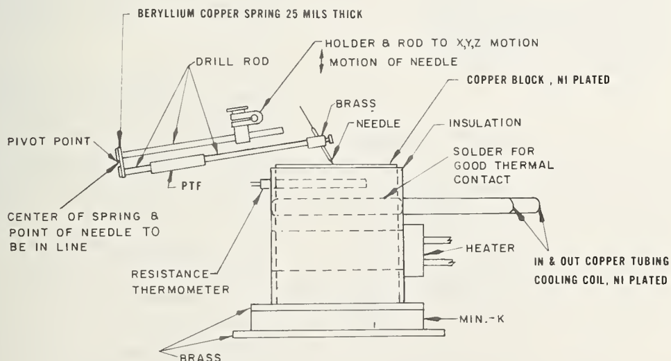
Figure 9. Probe system for making electrical contact to wafers. The wafer holder is designed to allow no more than a 2^{\circ}\text{C} difference between the device and the base, where the temperature is measured. The "MIN-K" specification for the base refers to any low thermal conductivity material that is an electrical insulator. PTF refers to the material polytetrafluoroethylene.
