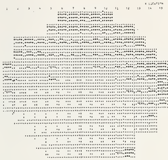
Figure 18. Map of threshold voltage where the magnitude of threshold voltage is indicated by the darkness of the position characters.
