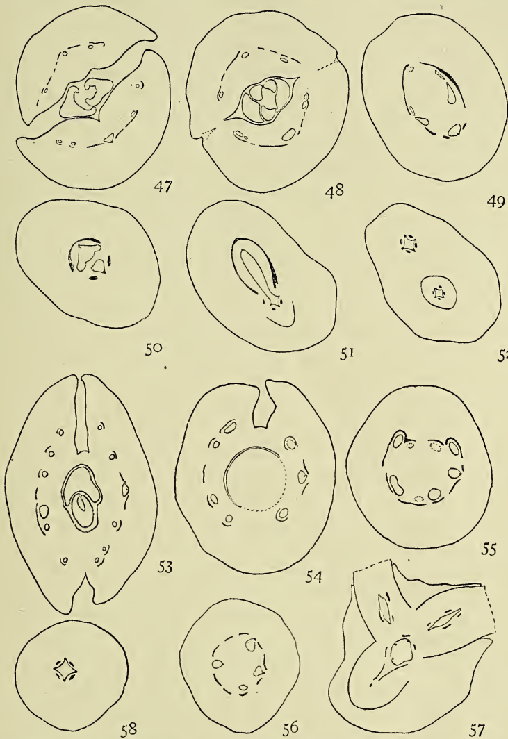
FIGS. 47-58. Figs. 47-52 show the transition phenomena in a seedling (Figs. 6 a , 6 b ) in which the cotyledons are markedly unequal. Figs. 53-58 show the transition in a seedling (Fig. 7) in which cotyledonary inequality and syncotyls are combined.
