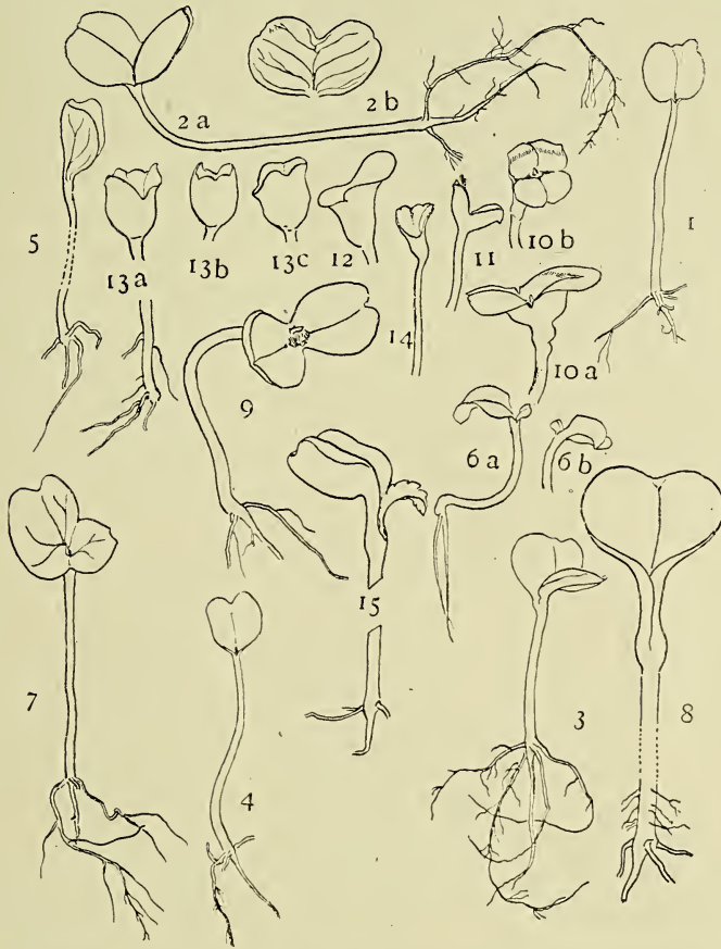
FIGS. 1-15. Fig. 1. 'Seedling A.' A syncotyl combining tetrarchy at the base of the hypocotyl with extremely intimate syncotyl. Figs. 2 a, 2 b. 'Seedling B.' A syncotyl in which the hypocotyl is diarch; Fig. 2 b shows the venation of the compound lamina. Figs. 3, 4. Syncotyls showing tetrarchy. Fig. 5. A syncotyl showing a triarch hypocotyl; the tap-root was pentarch. Figs. 6 a, 6 b. Seedling with markedly unequal cotyledons. Fig. 7. A syncotyl with unequal cotyledons. Fig. 8. Large 'Type 2' seedling in which the epicotyl has not developed. Figs. 9, 10 a, 10 b. Salver-shaped amphisyncotyls, 'Seedlings C and D' respectively. Figs. 11-14. Goblet-shaped amphisyncotyls. Fig. 15. 'Seedling H.'
