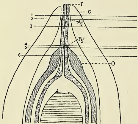
TEXT-FIG. 1. Diagrammatic view of section of young ovule of Gnemon , 3 mm. long, in which closure of micropyle is just beginning. c , outer covering; o , middle covering; 1 is the inner covering terminating in the freely projecting micropylar tube. Af , Bf , are the beginnings of the projecting upward and downward flanges of the micropylar tube. 1-6 represent the levels of Photos 1-6, Pl. I.
