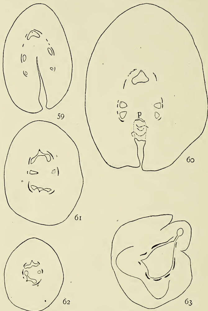
FIGS. 59-63. Transition in a 'Type 2' seedling (Fig. 8). Fig. 60 shows the effect of partial roofing-in of the plumule on the side of the base of the petiole. The dotted lines . . . . indicate irregular lines of crushed cells; p . = the pore-like communication with the plumular bud.
