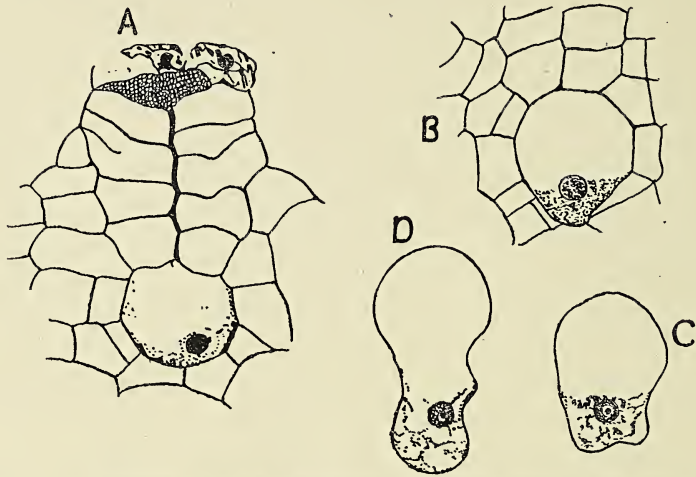
TEXT-FIG. 4 A. Recently fertilized archegonium containing unicellular embryo. \times 270 . B-D. Older unicellular embryos. \times 270 .
