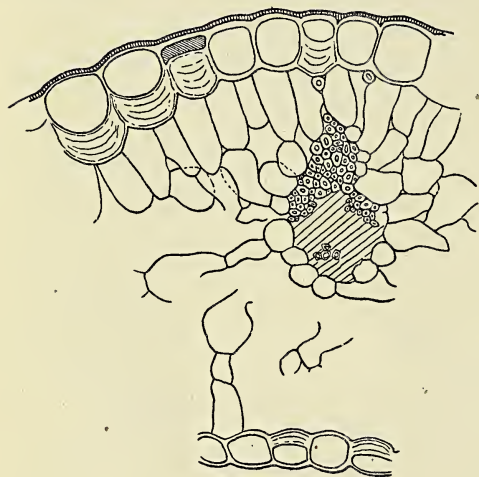
Fig. 12. Portion of section of juvenile leaf of P. filiformis , showing sunk stomata in upper concave epidermis.
