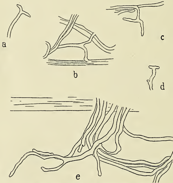
FIG. 9. a-e. Branching hypodermal fibres.
