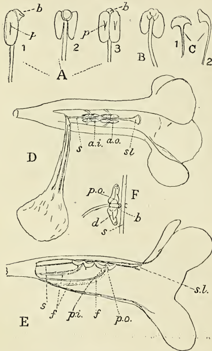
FIG. 2. A. Anther-lobes of longer stamen: 1, side view; 2, back view; 3, front view. \times 2 . B. Back view of shorter stamen. \times 2 . C. Young stigma: 1, front view; 2, side view. D. Diagrammatic view of flower from below (with a slit in the side). E. Diagrammatic longitudinal section of flower. F. Diagram of anther showing the pad touching the style. \times 1\frac{1}{2} . p. process; p.o. outer process; p.i. inner process; b. 'buffer' or pad; a.i. inner anther; a.o. outer anther; f. filament; s. style; s.l. stigmatic lobe; d. slit in anther lobe.
