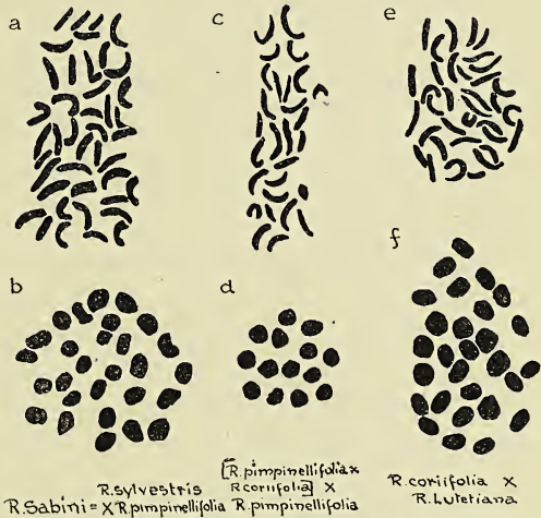
TEXT-FIG. 2. Somatic and heterotype metaphases in hybrids. × 3,000.
