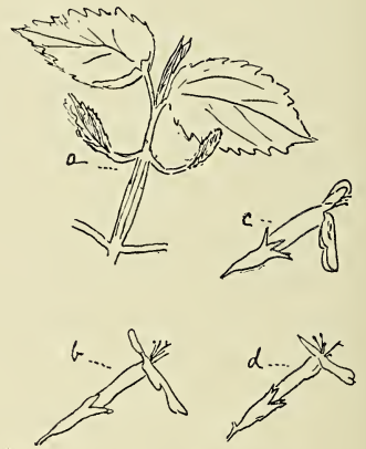
FIG. 2. (See Table II.) a , two shoots partly fused to main stem. For description see text and table. [Downley, near High Wycombe, Bucks., 1917.]
