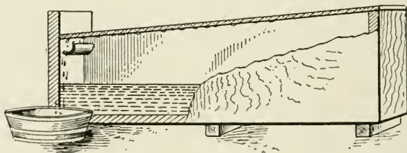
Fig. 162—A simple apparatus for distilling fresh water from sea water
