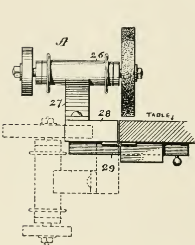
Fig. 50—Hinged mounting of the tool grinder
