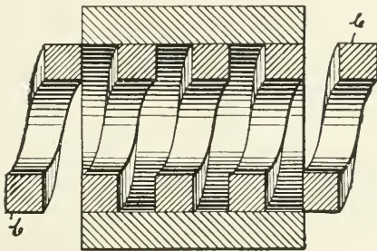
Fig. 83—Section showing thread in nut
