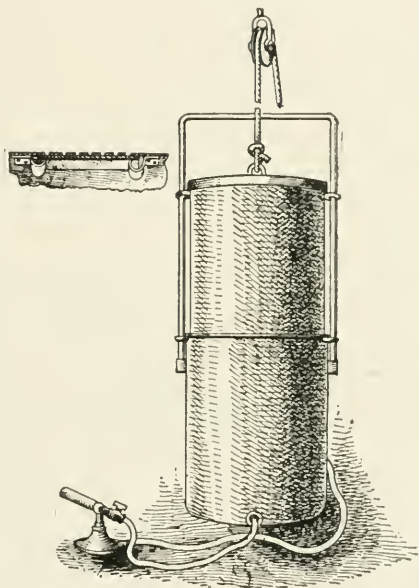
Fig. 132—Continuous blast apparatus
