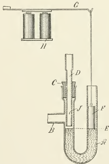
Fig. 163—Electrically-controlled gas regulator
