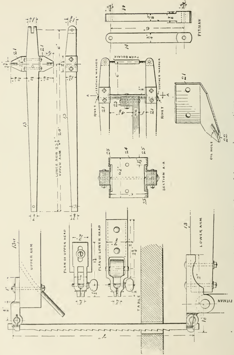
Fig. 49—The saw-frame fulcrum and connections
