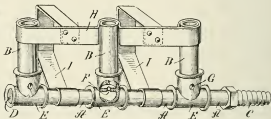
Fig. 286—A general view of the fire lighter
