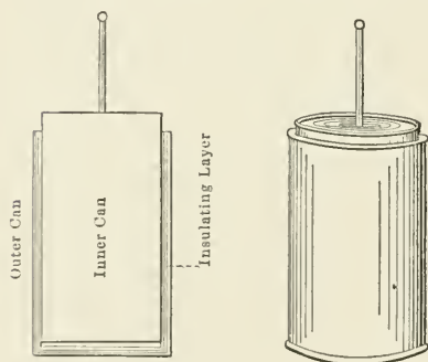
Fig. 195—An unbreakable Leyden jar
