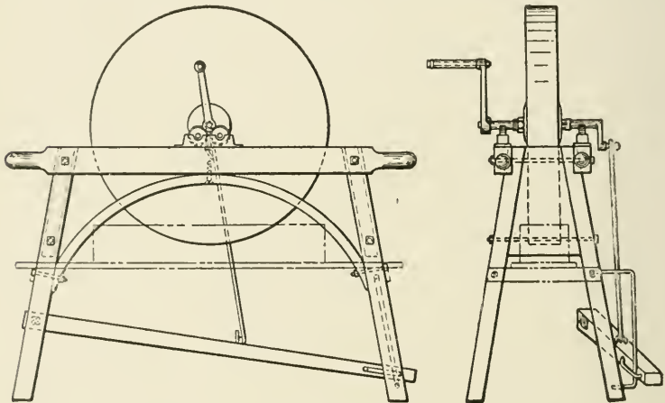
Fig. 27—Frame construction for grindstones
