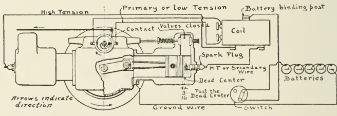
Fig. 323—Wiring diagram for engine
