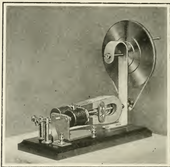
Fig. 209—A magneto machine of simple construction
