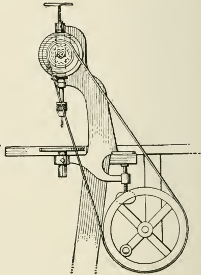
Fig. 51—The drill-press
