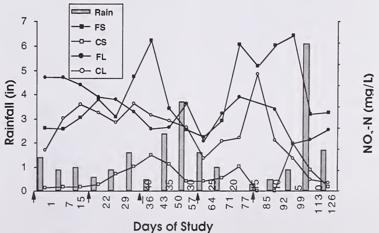
Figure 3. Nitrate-nitrogen concentrations and rainfall/irrigation amounts for State 2 between 5/21-9/24/92. Nitrogen fertilizer was added every 3 weeks at 56 kg/ha (50 lbs/ac) as 34-0-0 or 21-0-0. Nitrate-nitrogen concentrations: FS = fertilized - 15 cm (6 in); CS = unfertilized - 15 cm (6 in); FL = fertilized - 1 m (3 ft); CL = unfertilized - 1 m (3 ft).
