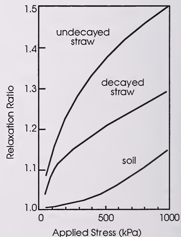
Figure 8. Relaxation ratio (elasticity) of soil compared to undecayed and decayed wheat straw (after Guerif, 1979).
