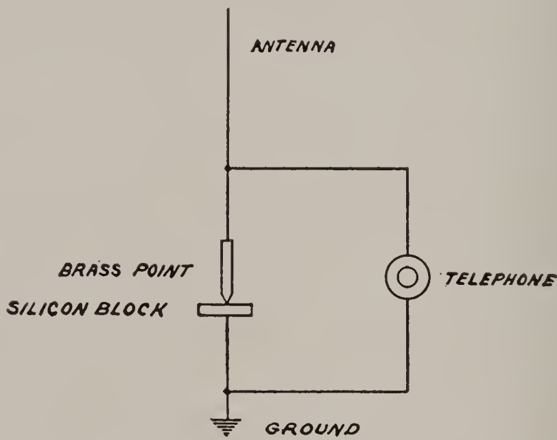
FIG. 17.—CONNECTIONS OF SILICON DETECTOR.
