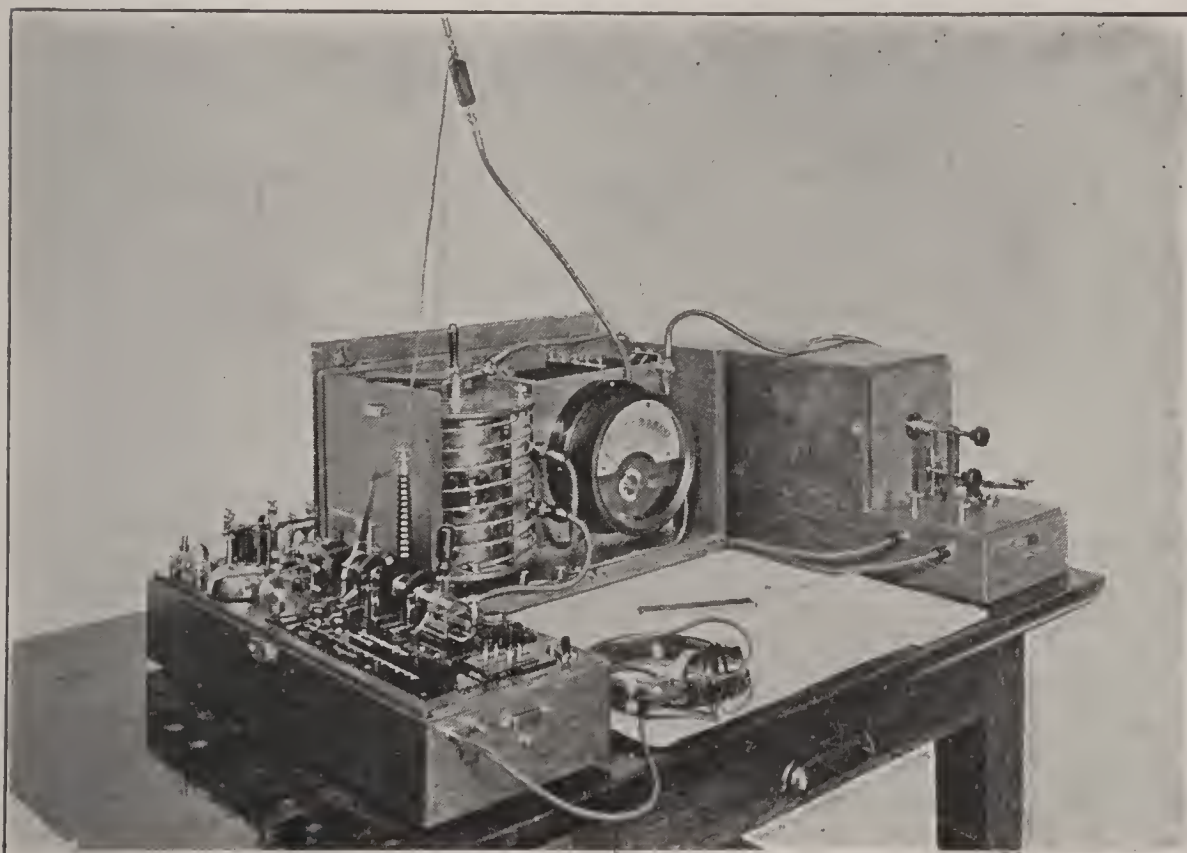
FIG. 25.—COMPLETE PORTABLE OUTFIT.
