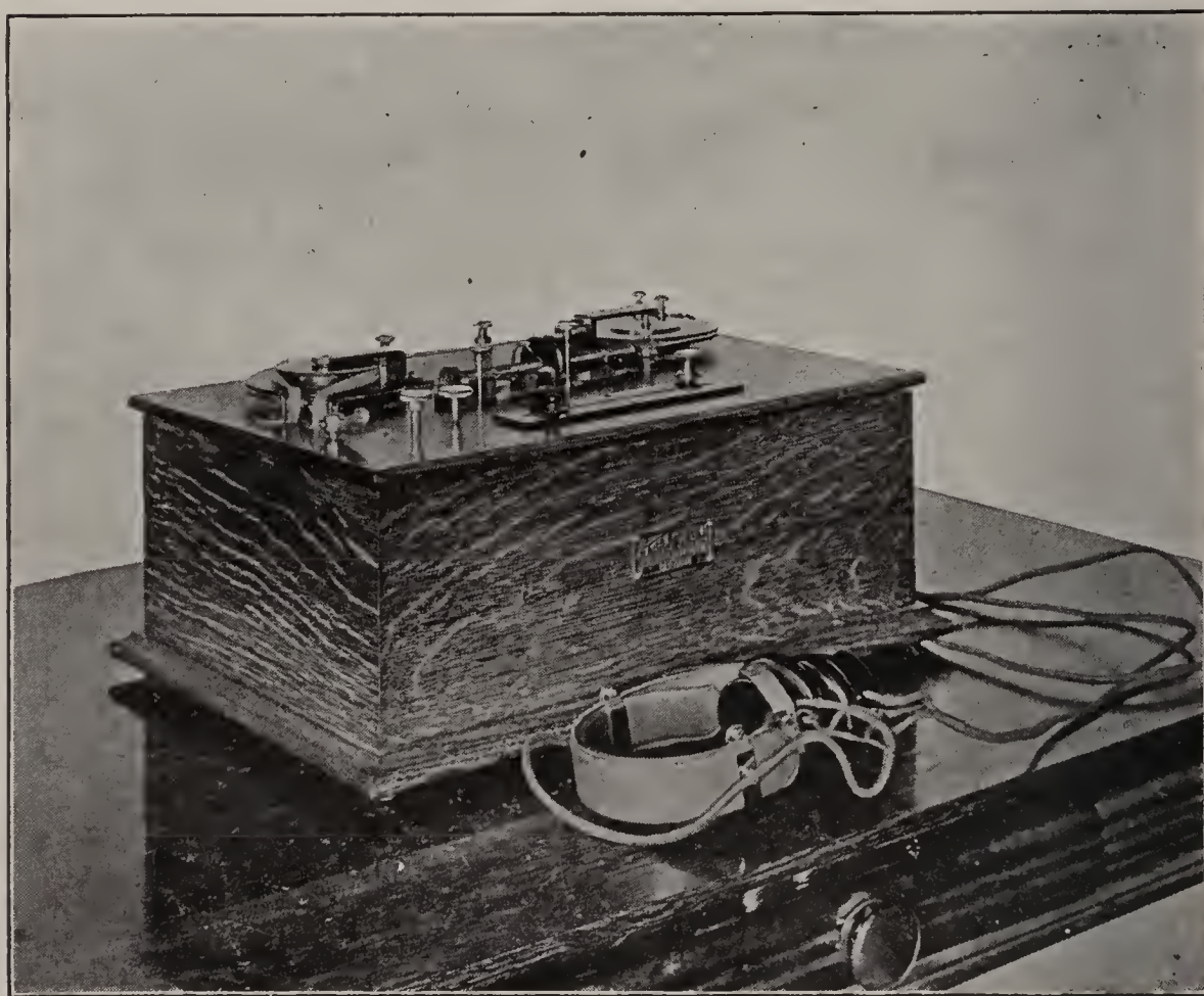
FIG. 15.—MAGNETIC DETECTOR.
