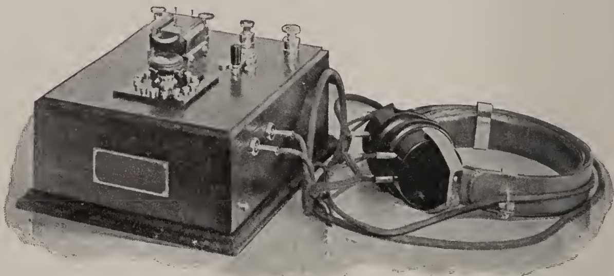
FIG. 11.—MICROPHONE WITH TELEPHONE RECEIVERS CONNECTED.
