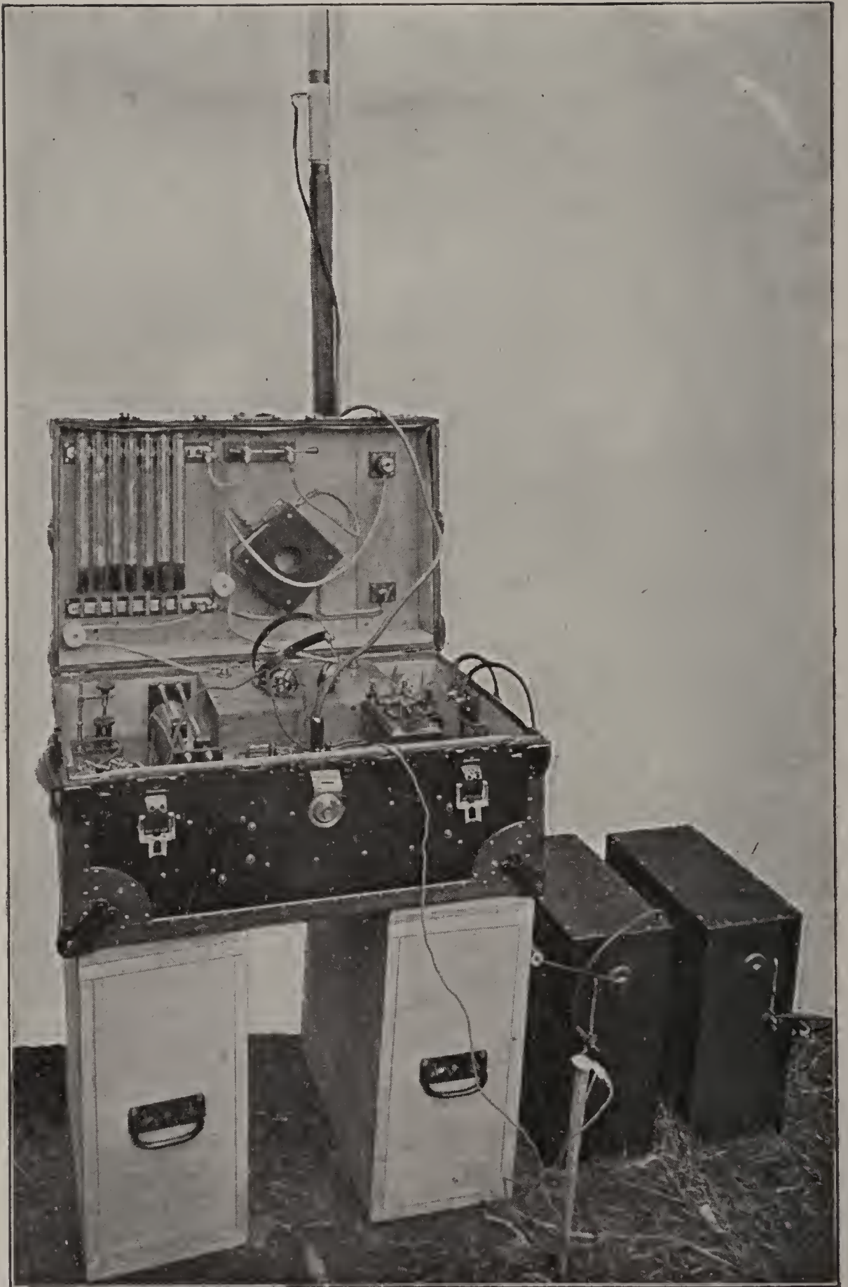
FIG. 24.—PORTABLE SIGNAL CORPS U. S. A. OUTFIT "READY FOR BUSINESS."
