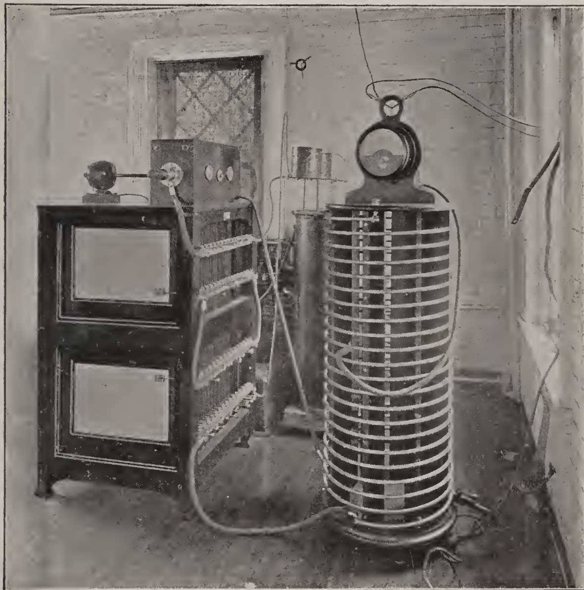
FIG. 8. — HIGH-POWER OUTFIT, WITH ROTATING SPARK-GAP MOUNTED ON LEYDEN-JAR BATTERY FRAME, AND HOT-WIRE CURRENT METER MOUNTED ON INDUCTANCE FRAME. —Navy Yard, Washington, D. C.
