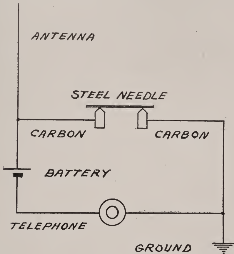
FIG. 12.—MICROPHONE CONNECTIONS.
