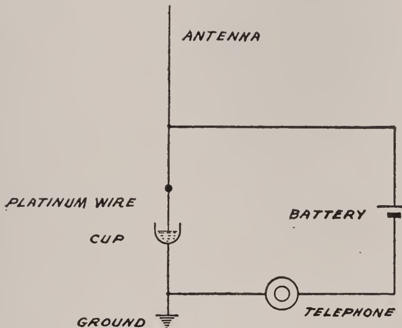
FIG. 14.—CONNECTIONS OF ELECTROLYTIC DETECTOR.
