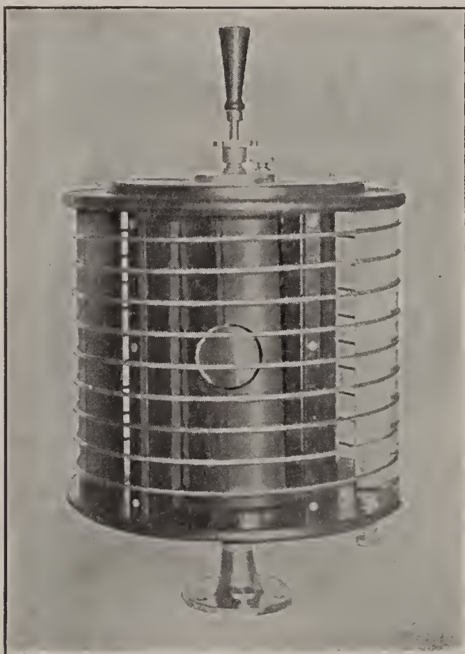
FIG. 6.—SPARK-GAP WITH MUFFLER, SURROUNDED BY INDUCTANCE.
