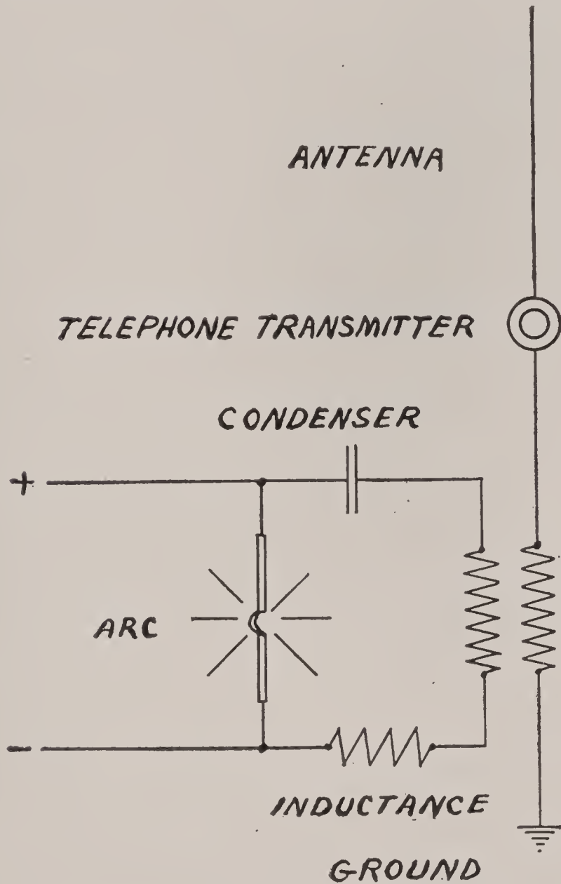
FIG. 27.—WIRELESS TELEPHONE TRANSMITTER CONNECTIONS.
