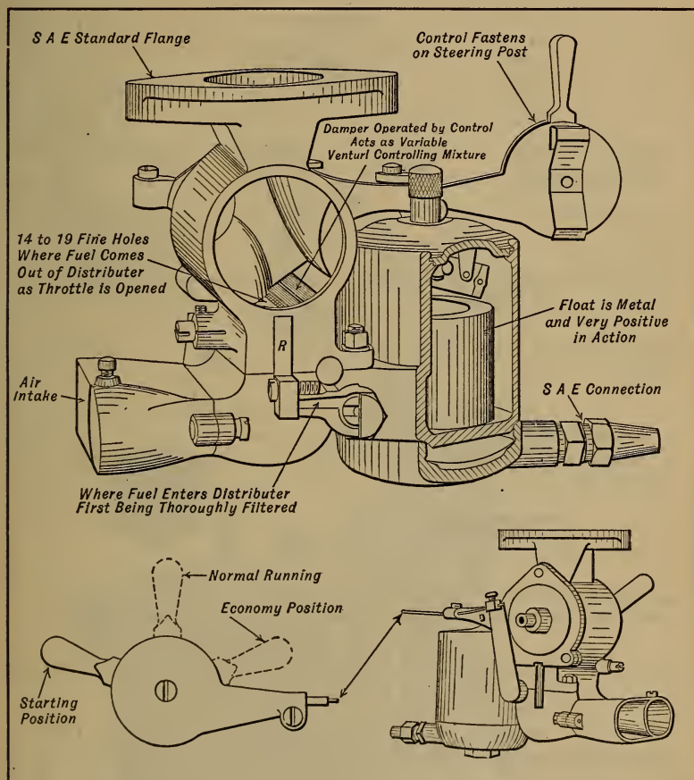
Fig. 49.—The Master Carburetor.
