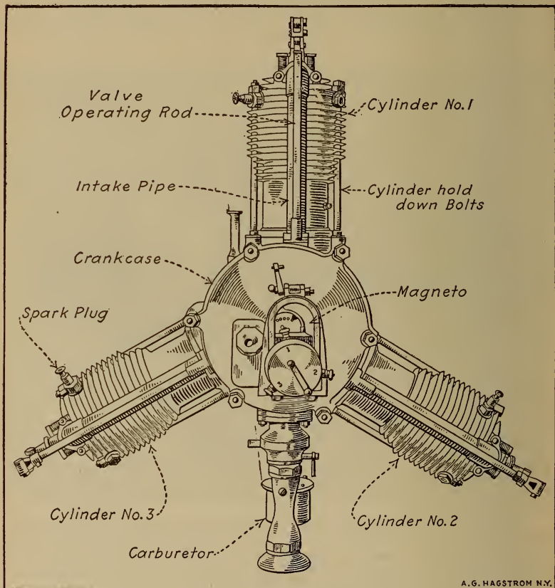
Fig. 193.—Three-Cylinder Anzani Air-Cooled Y-Form Engine.
