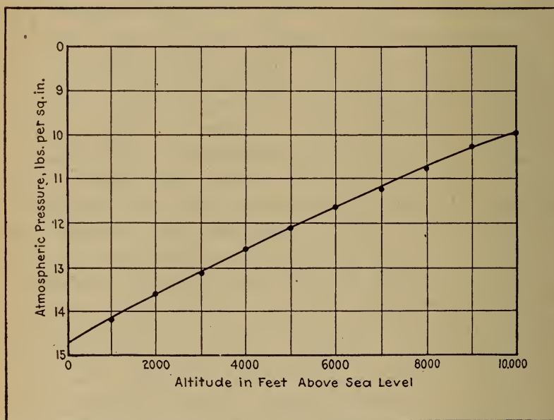
Fig. 56.—Chart Showing Diminution of Air Pressure as Altitude Increases.
