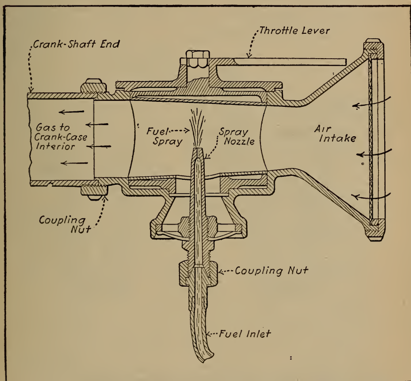
Fig. 206.—Simple Carburetor Used On Early Gnome Engines Attached to Fixed Crank-Shaft End.
