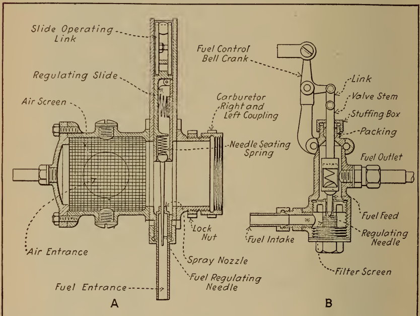
Fig. 221.—The Le Rhone Carburetor at A and Fuel Supply Regulating Device at B.
