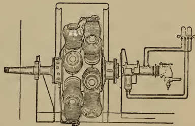
Fourteen or Eighteen Cylinder Revolving Air Cooled Aviation Engine Speed 1200 R.P.M. 2 Pounds per Horsepower
