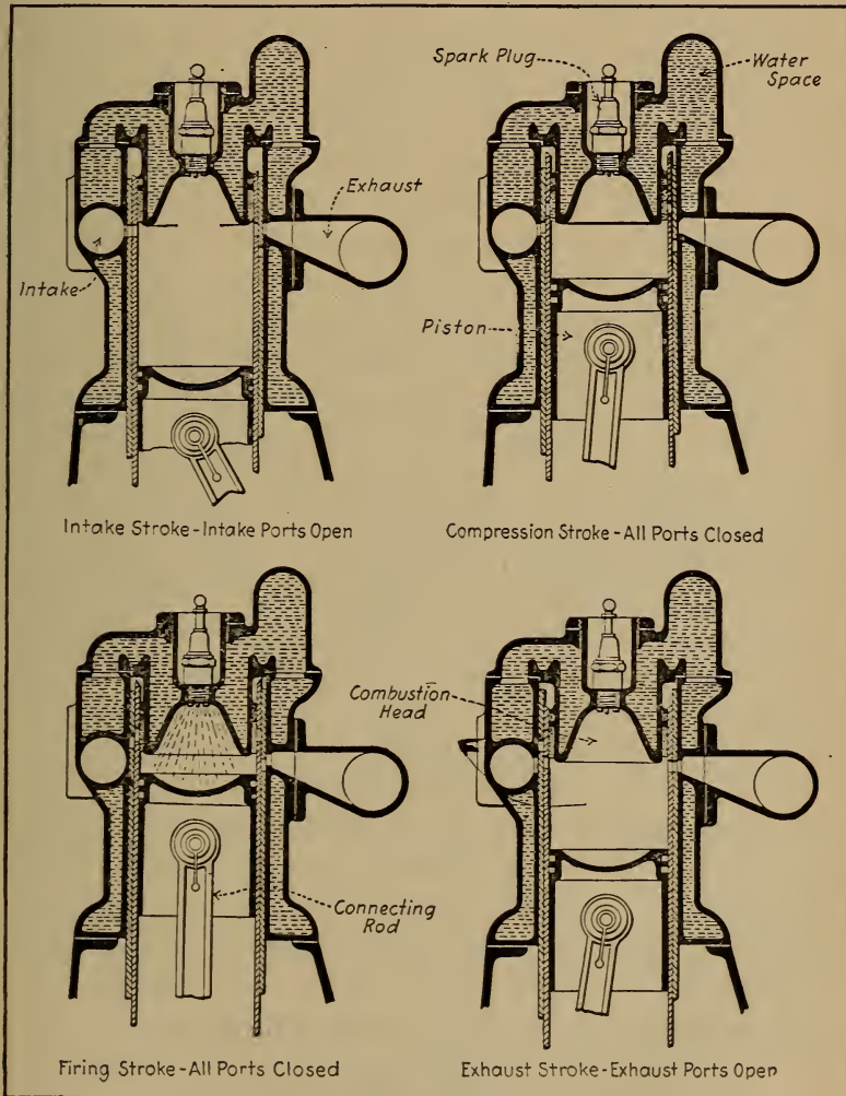
Fig. 106.—Diagrams Showing Knight Sleeve Valve Action.
