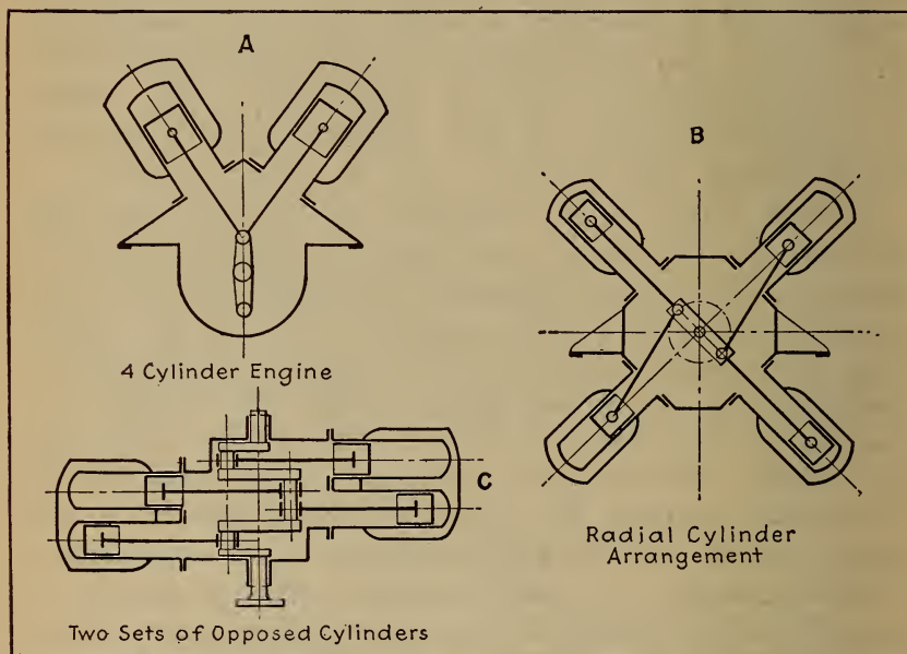
Fig. 24.—Showing Three Possible Though Unconventional Arrangements of Four-Cylinder Engines.
