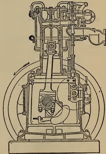
Stationary Gas Engine Four Cycle - Two Cylinder 300 Pounds per Horsepower
