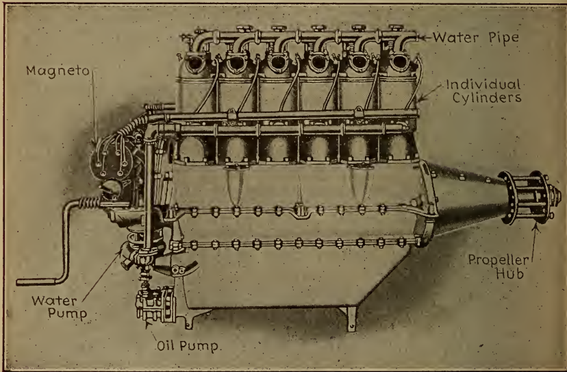
Fig. 236.—The Six-Cylinder Aeromarine Engine.
