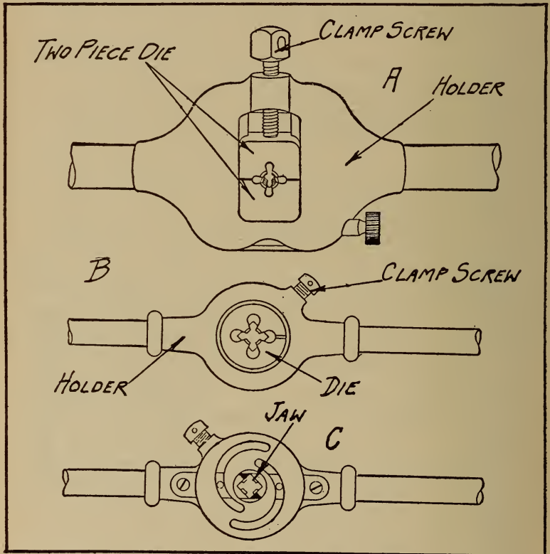
Fig. 172.—Showing Holder Designs for One- and Two-Piece Thread Cutting Dies.
