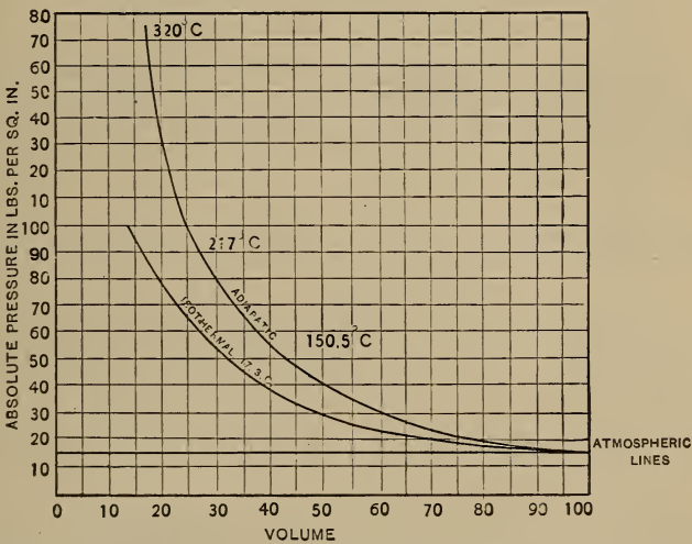
Fig. 11.—Diagram Isothermal and Adiabatic Lines.
