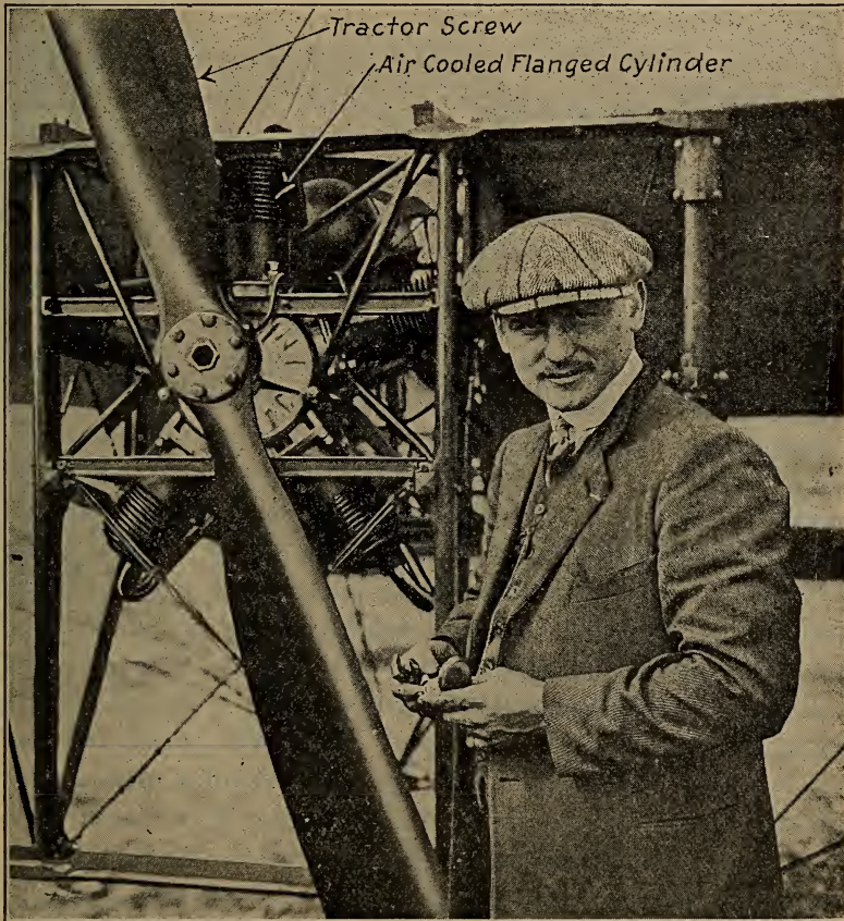
Fig. 85.—Anzani Testing His Five-Cylinder Air Cooled Aviation Motor Installed in Bleriot Monoplane. Note Exposure of Flanged Cylinders to Propeller Slip Stream.
