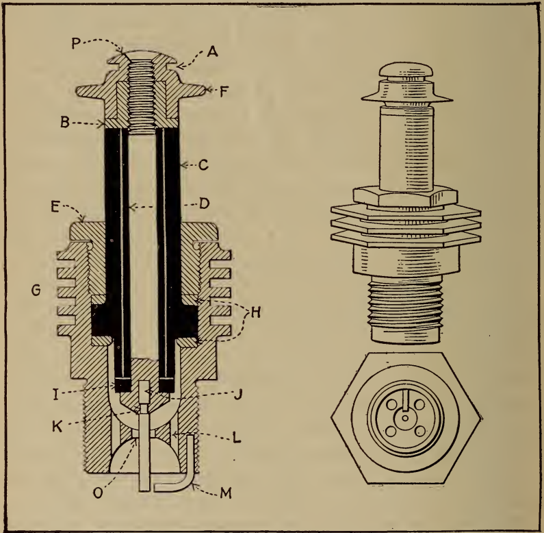
Fig. 74.—Special Mica Plug for Aviation Engines.
