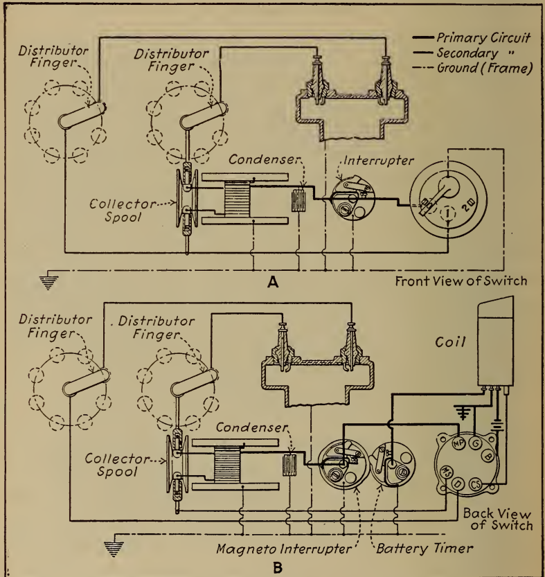
Fig. 64.—Wiring Diagrams of Berling Magneto Ignition Systems.
