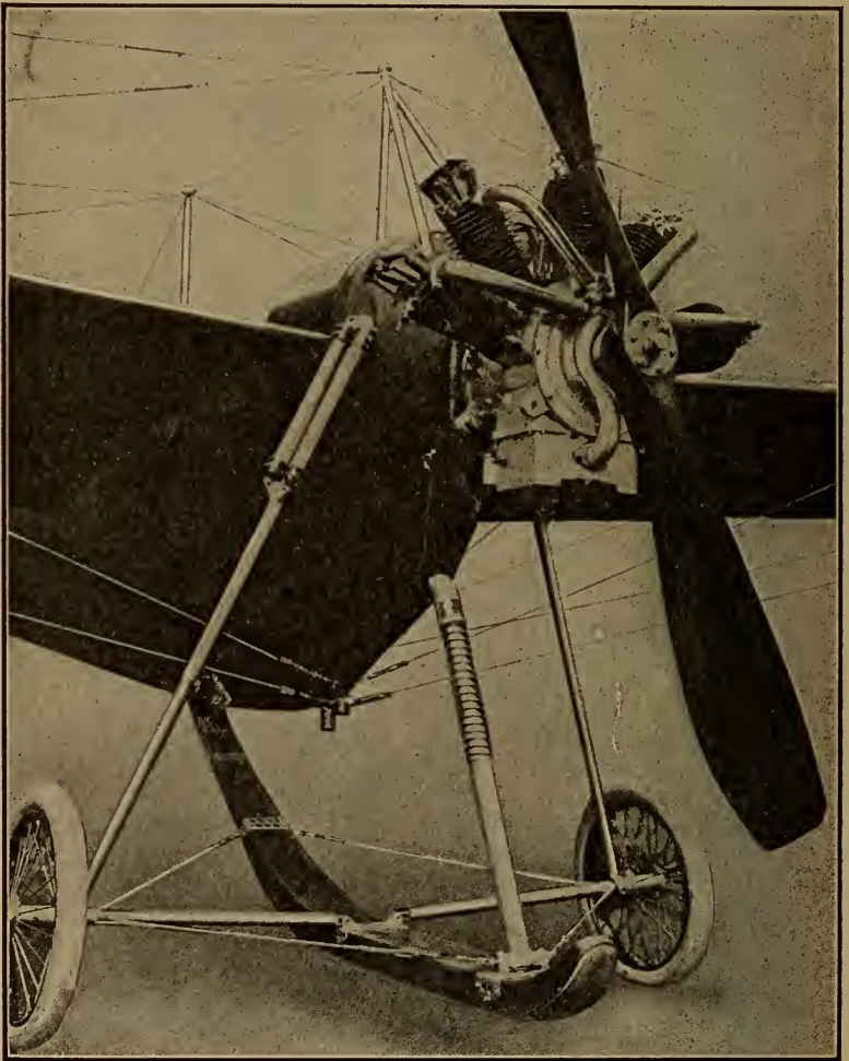
Fig. 197.—Application of R. E. P. Five-Cylinder Fan-Shape Air-Cooled Motor to Early Monoplane.
