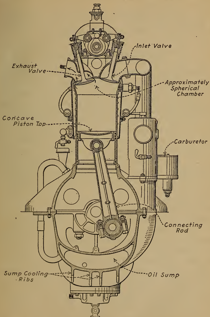
Fig. 20.—Mercedes Aviation Engine Cylinder Section Showing Approximately Spherical Combustion Chamber and Concave Piston Top.
