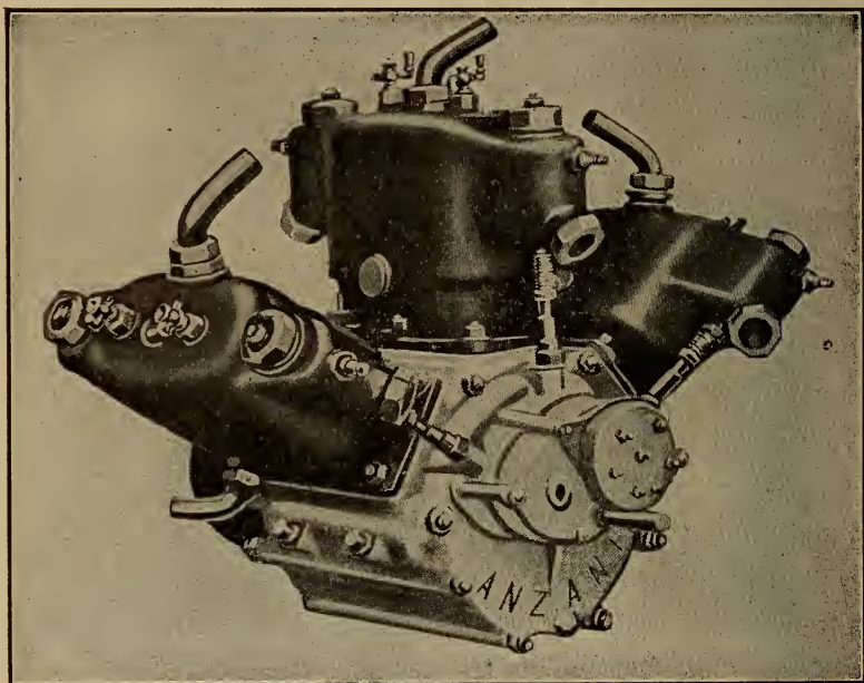
Fig. 191.—The Anzani Six-Cylinder Water-Cooled Aviation Engine.
