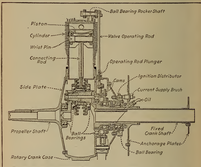
Fig. 217.—Side Sectional View of Le Rhone Aviation Engine.
