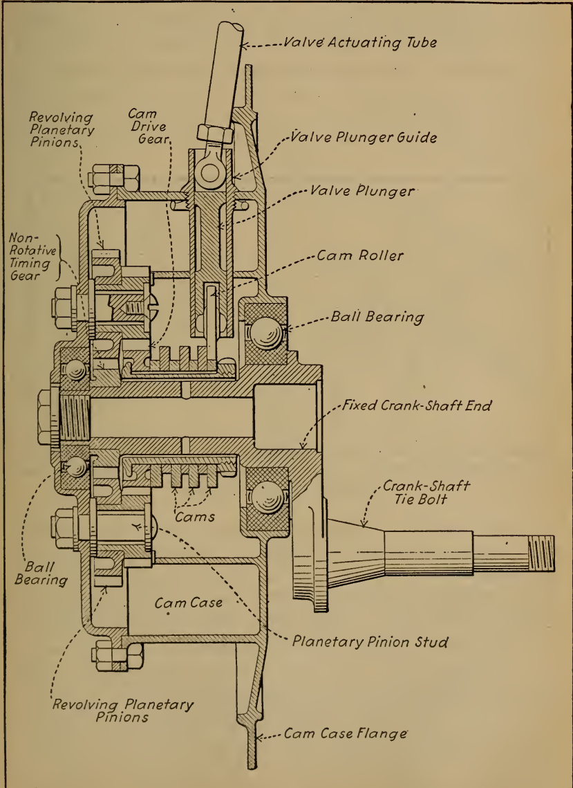
Fig. 204.—Cam and Cam-Gear Case of the Gnome Seven-Cylinder Revolving Engine.
