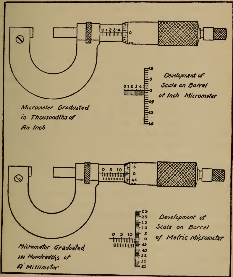
Fig. 178.—Standard Forms of Micrometer Caliper for External Measurements.
