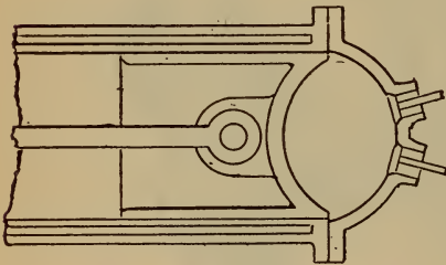
Fig. 18.—Spherical Combustion Chamber.
