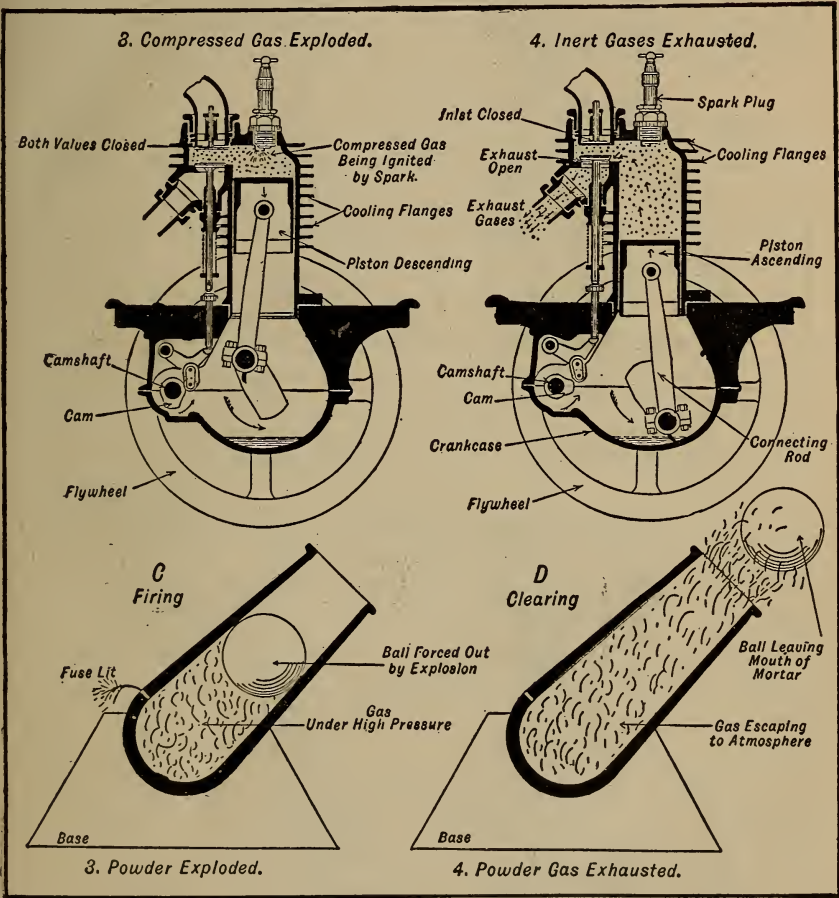
Fig. 6.—Outlining Second Two Strokes of Piston in Four-Cycle Engine.
