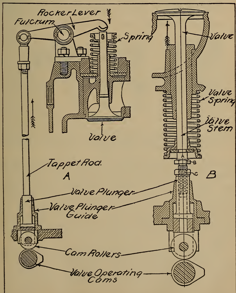
Fig. 95.—Conventional Methods of Operating Internal Combustion Motor Valves.
