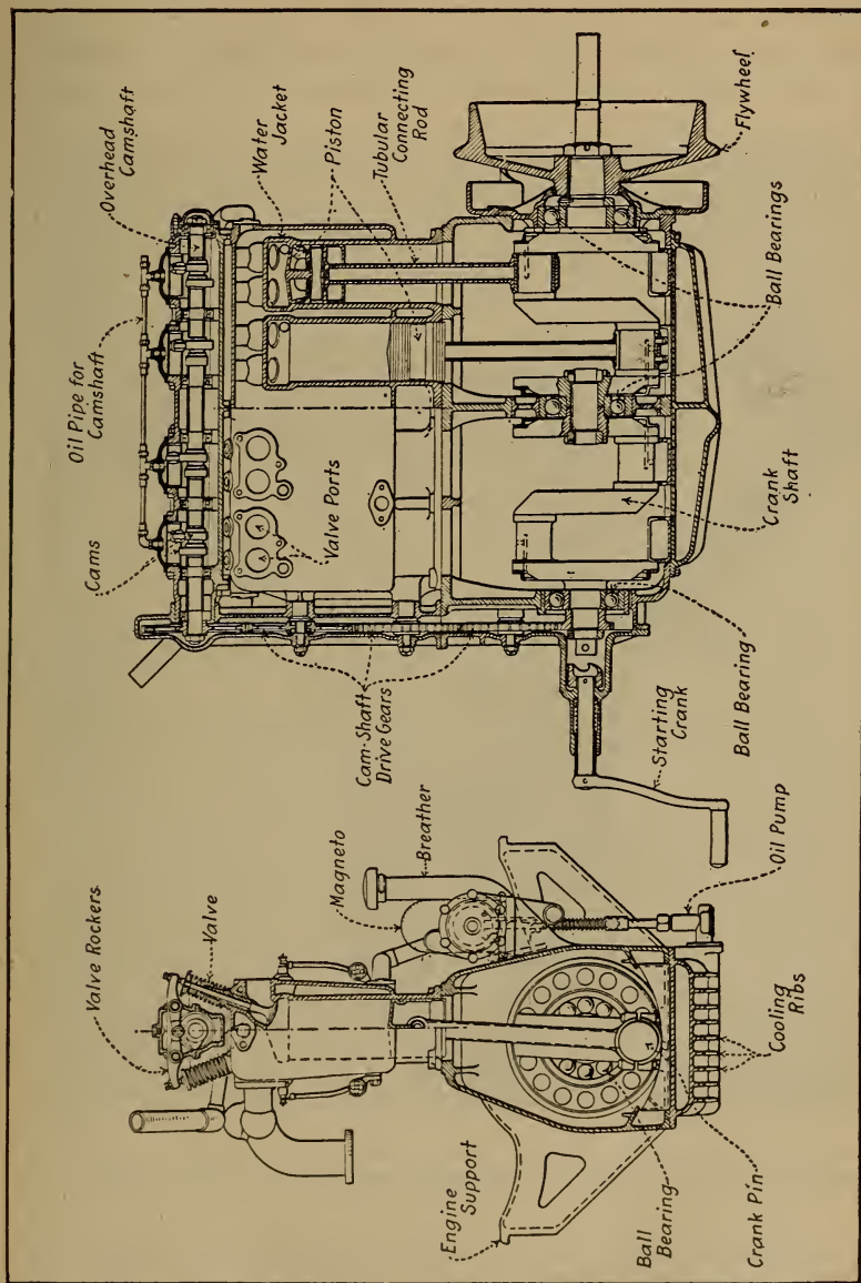
Fig. 114.—Sectional Views of Sixteen-Valve Four-Cylinder Automobile Racing Engine That May Have Possibilities for Aviation Service.
