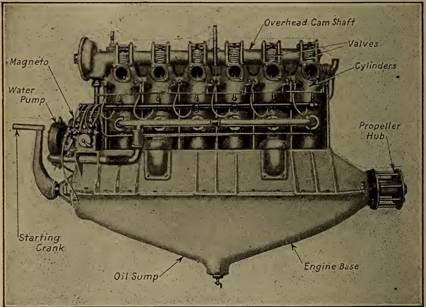
Fig. 35.—The Hall-Scott Six-Cylinder Aviation Engine.
