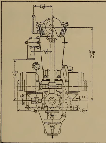
Fig. 238.—Dimensioned End Elevation of Wisconsin Six Motor.
