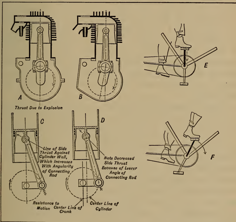
Fig. 91.—Diagrams Demonstrating Advantages of Offset Crank-Shaft Construction.
