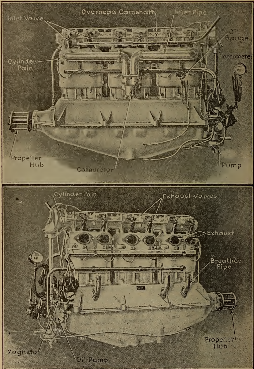
Fig. 237.—The Wisconsin Aviation Engine, at Top, as Viewed from Carburetor Side. Below, the Exhaust Side.
