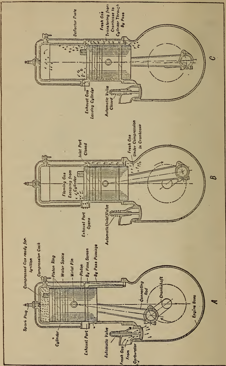
Fig. 8.—Showing Two-port, Two-cycle Engine Operation.
