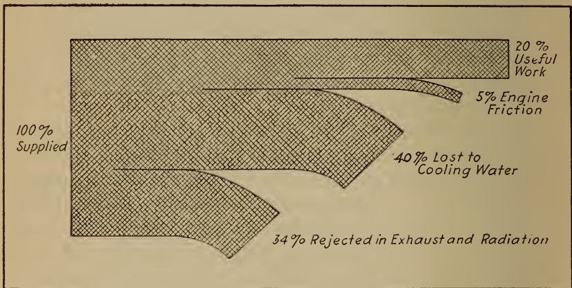
Fig. 12.—Graphic Diagram Showing Approximate Utilization of Fuel Burned in Internal-Combustion Engine.
