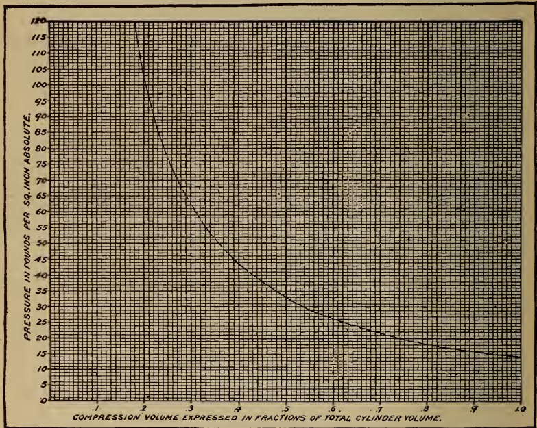
Fig. 16.—Chart Showing Relation Between Compression Volume and Pressure.
