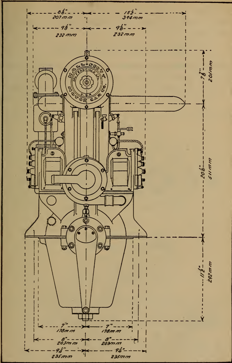
Fig. 148.—End Elevation of Hall-Scott A-7 Four-Cylinder Motor, with Installation Dimensions.
