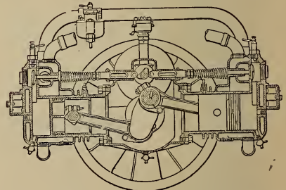
Two Cylinder Four Cycle Tractor Engine 75 Pounds per Horsepower 800 to 1000 R.P.M.
