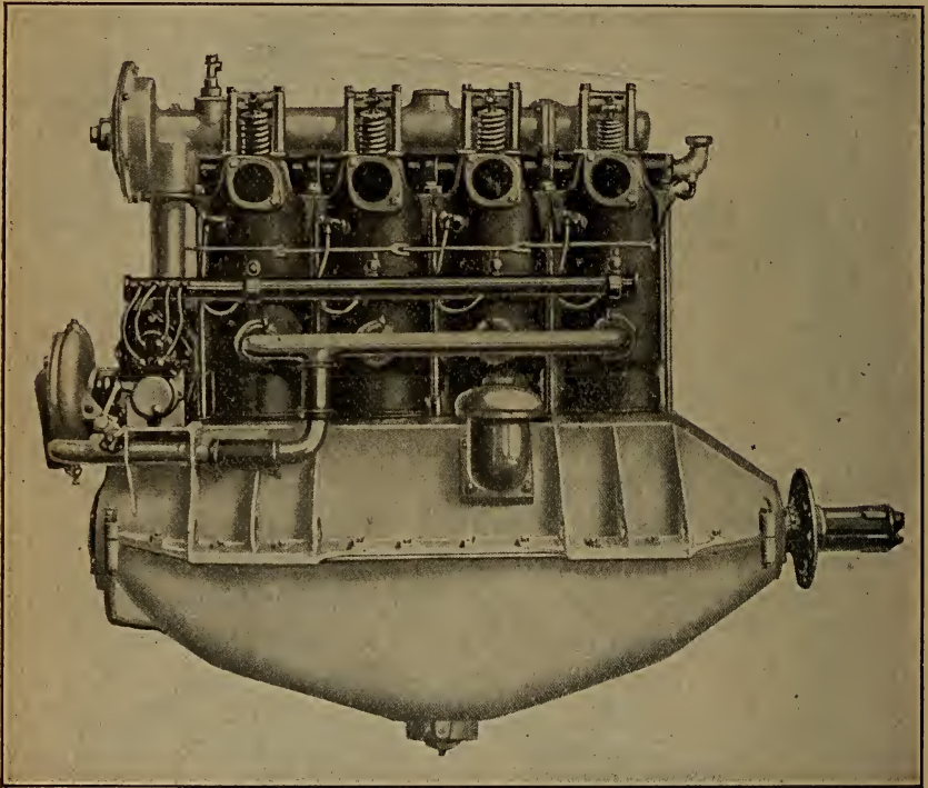
Fig. 33.—The Hall-Scott Four-Cylinder 100 Horse-Power Aviation Motor.
