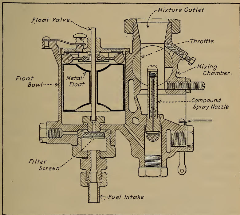
Fig. 46.—The Claudel Carburetor
