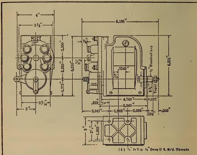
Fig. 67.—Installation Dimensions of Dixie Model 60 Magneto.
