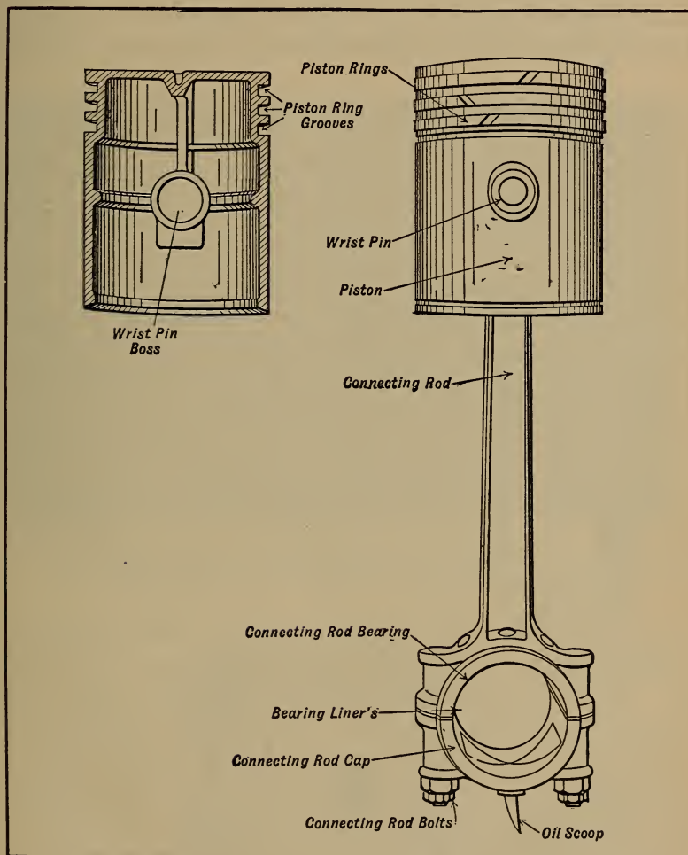
Fig. 118.—Typical Piston and Connecting Rod Assembly.
