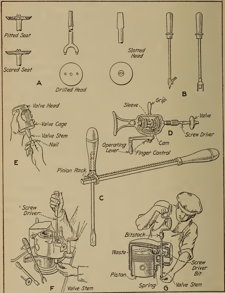
Fig. 184.—Tools and Processes Utilized in Valve Grinding.
