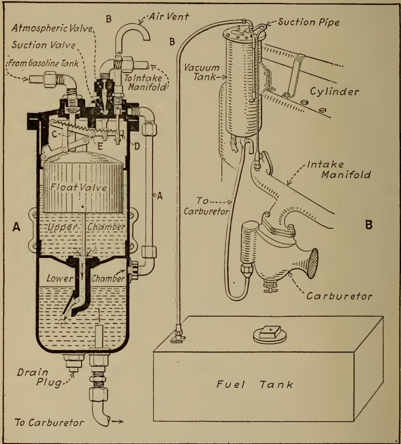
Fig. 42.—The Stewart Vacuum Fuel Feed Tank.
