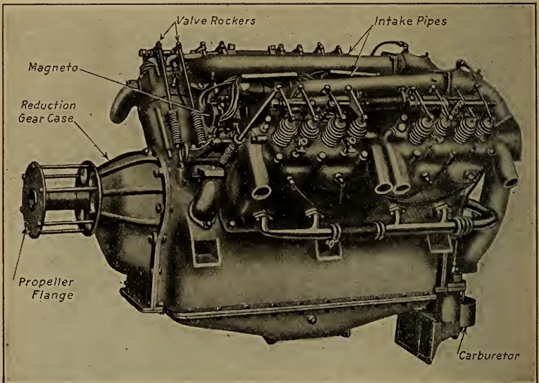
Fig. 37.—The Sturtevant Eight-Cylinder, High Speed Aviation Motor.
