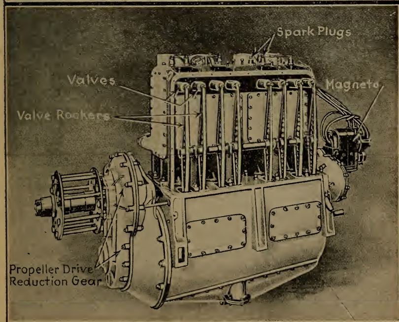
Fig. 34.—Two Views of the Duesenberg Sixteen Valve Four-Cylinder Aviation Motor.
