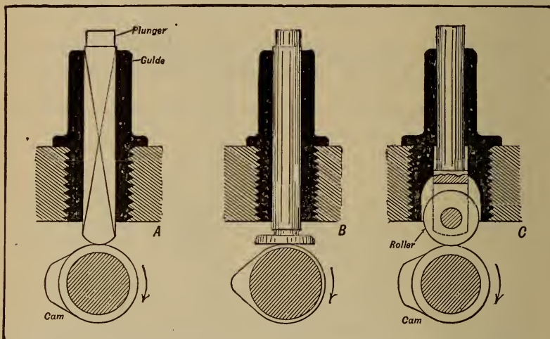
Fig. 102.—Showing Principal Types of Cam Followers which Have Received General Application.
