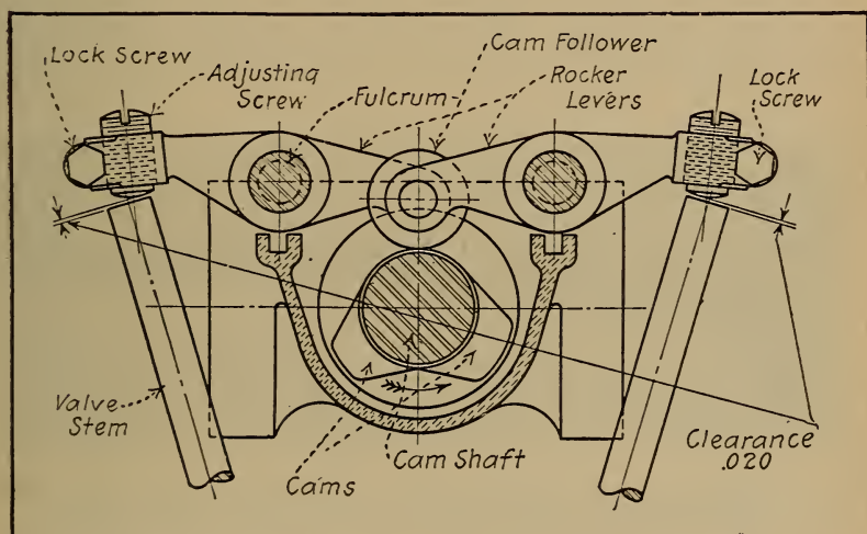
Fig. 103.—Diagram Showing Proper Clearance to Allow Between Adjusting Screw and Valve Stems in Hall-Scott Aviation Engines.
