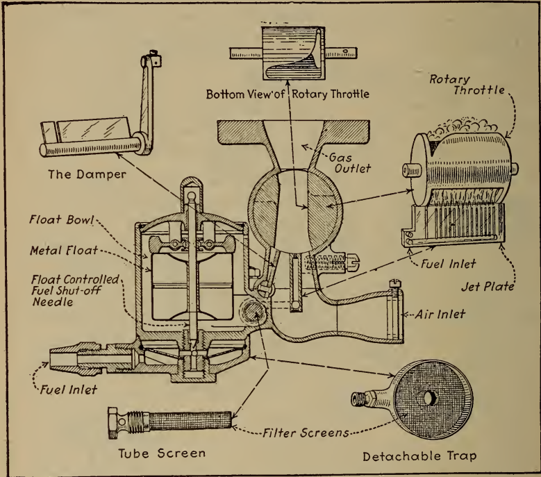
Fig. 50.—Sectional View of Master Carburetor Showing Parts.
