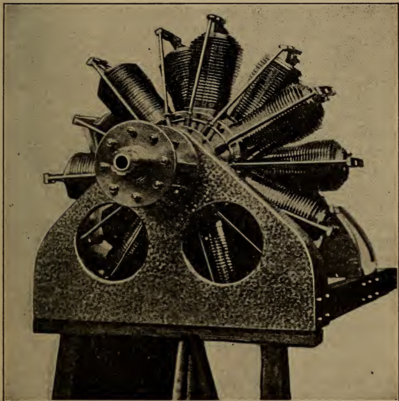
Fig. 40.—The Gnome Fourteen-Cylinder Revolving Motor.
