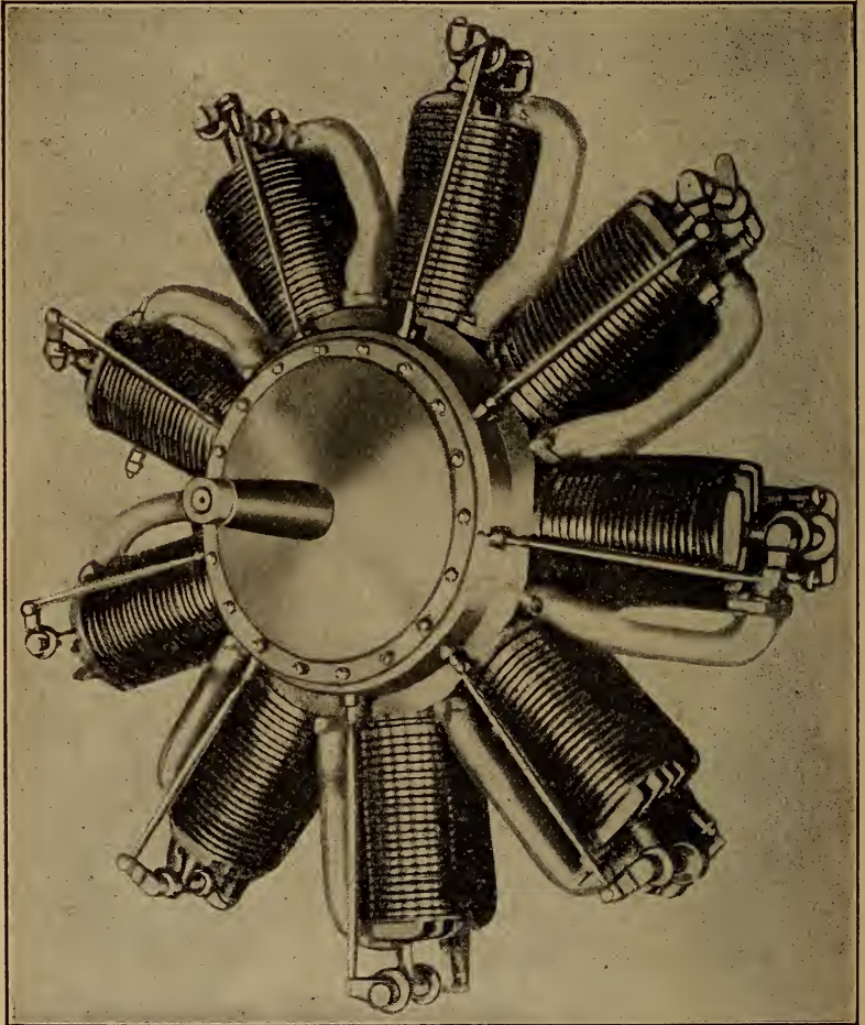
Fig. 215.—Nine-Cylinder Revolving Le Rhone Type Aviation Engine.
