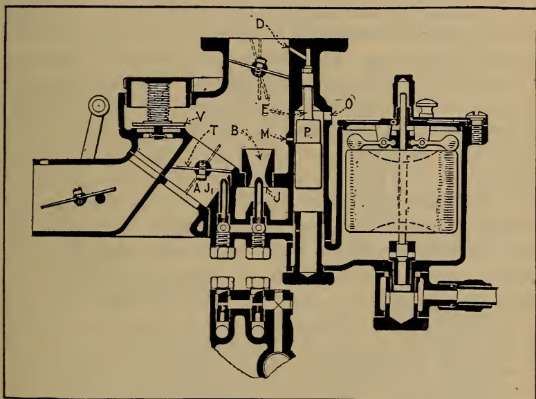
Fig. 48.—The Ball and Ball Two-Stage Carburetor.
