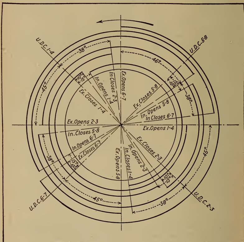
Fig. 110.—Timing Diagram of Typical Eight-Cylinder V Engine.
