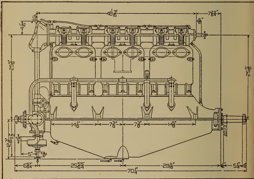
Fig. 239.—Dimensioned Side Elevation of Wisconsin Six Motor.
