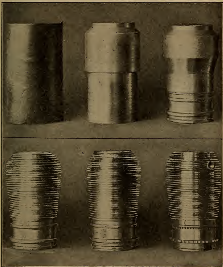
Fig. 211.—How a Gnome Cylinder is Reduced from Solid Chunk of Steel Weighing 97 Pounds to Finished Cylinder Weighing 5\frac{1}{2} Pounds.
