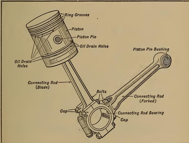
Fig. 129.—Double Connecting Rod Assembly For Use On Single Crank-Pin of Vee Engine.
