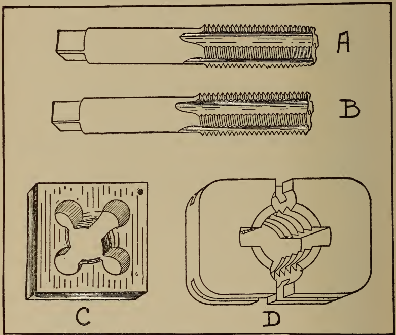
Fig. 171.—Tools for Thread Cutting.
