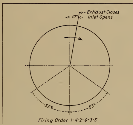
Fig. 241.—Timing Diagram, Wisconsin Aviation Engine.
