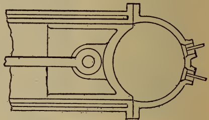
Fig. 19.—Enlarged Combustion Chamber.
