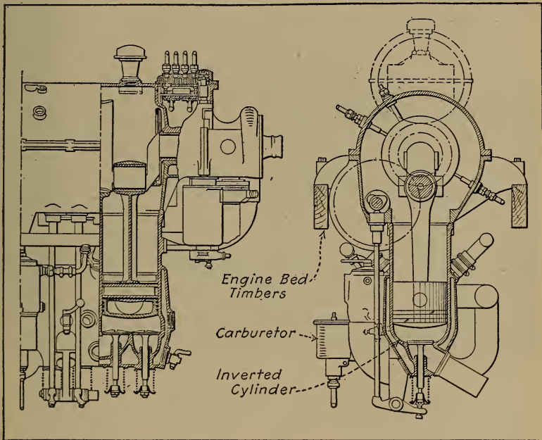
Fig. 144.—Unconventional Mounting of German Inverted Cylinder Motor.
