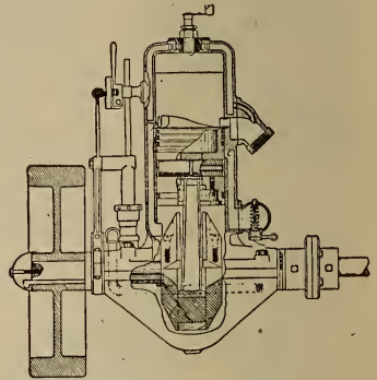
Two-Cycle Marine Engine 50-100 Pounds per Horsepower 600 to 800 R.P.M.
