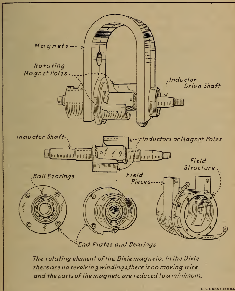
Fig. 68.—The Rotating Elements of the Dixie Magneto.
