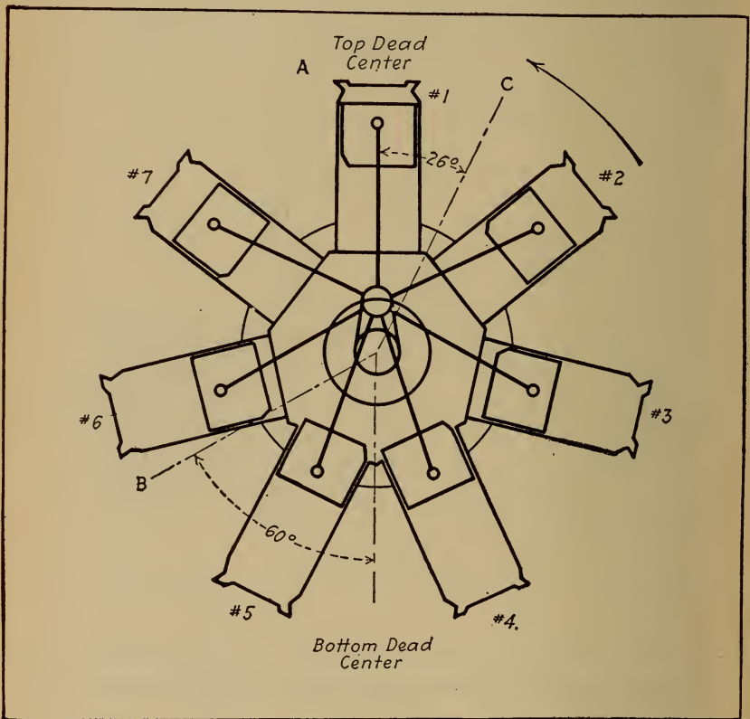
Fig. 223.—Diagram Showing Positions of Piston in Le Rhone Rotary Cylinder Motor.
