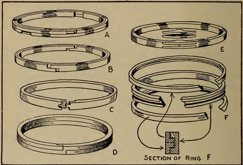
Fig. 125.—Leak-Proof and Other Compound Piston Rings.
