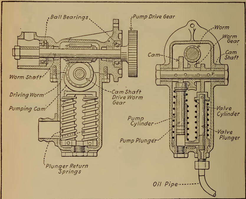
Fig. 207.—Sectional Views of the Gnome Oil Pump.
