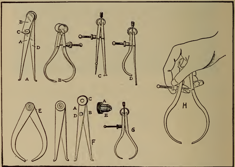
Fig. 174.—Common Forms of Inside and Outside Calipers.
