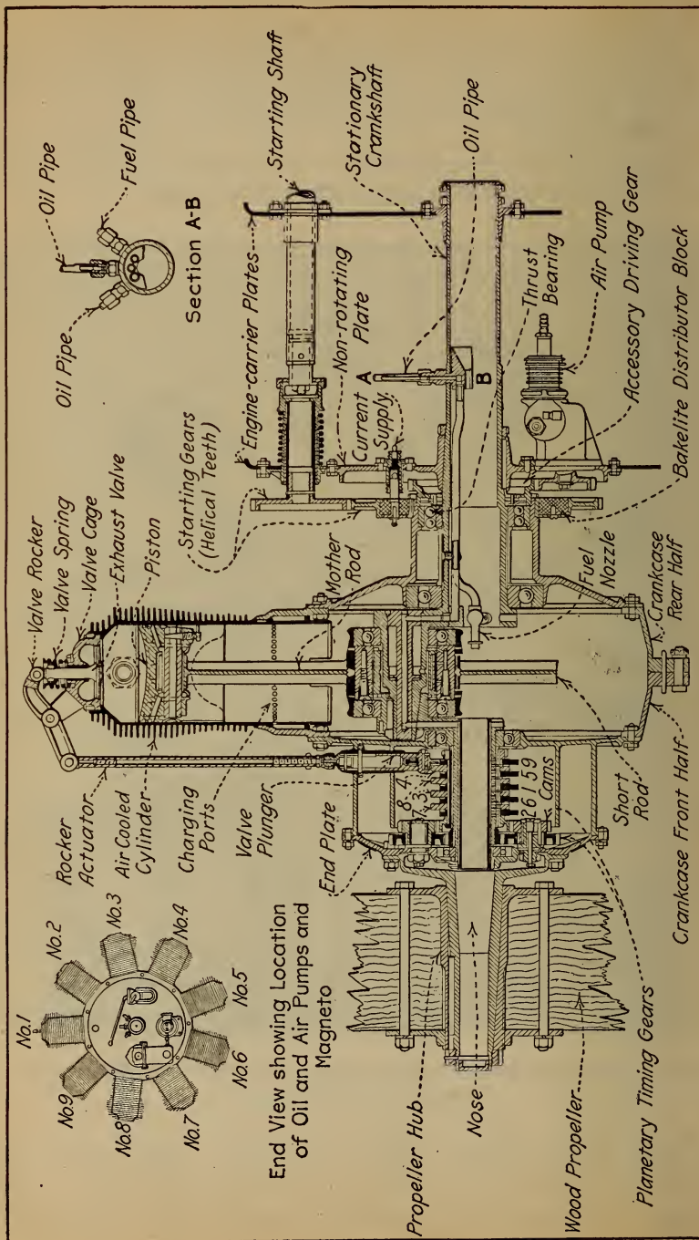
Fig. 210.—Sectional View Showing Construction of General Vehicle Co. 'Monosoupape,' Gnome Engine.
