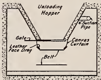
SECTION OF UNLOADING PIT
