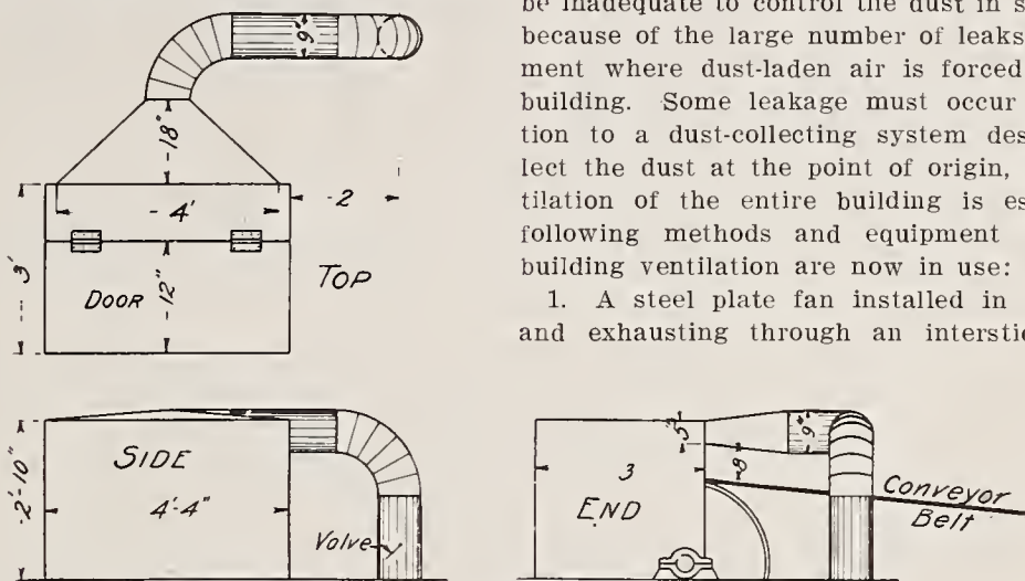
FIG. 8. DETAIL OF HOOD OVER WORKING FLOOR END OF CONVEYOR BELTS
