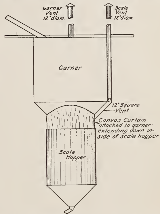
FIG. 5. ARRANGEMENT OF SCALE AND GARNER VENTS
