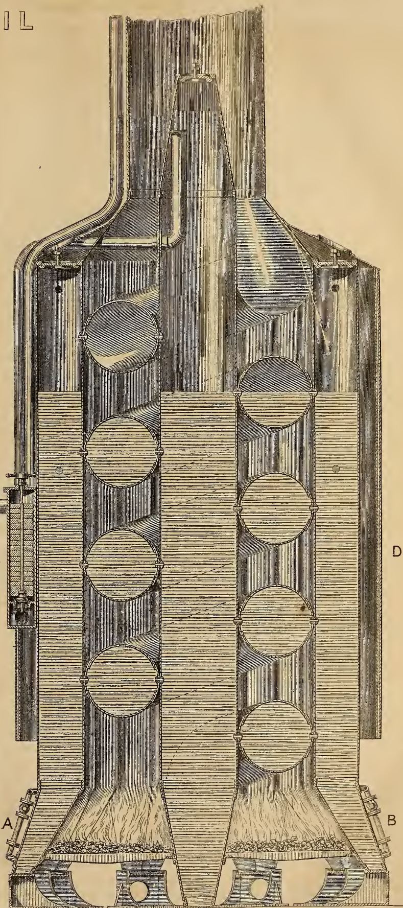
FIG. 2. SECTION
