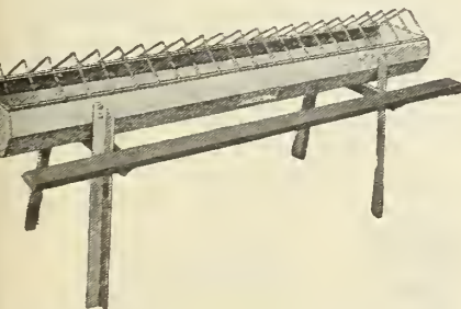
No. 25A—5 feet long. Trough 9 inches wide, 4 7/8 inches deep, holds 40 pounds or 4 1/2 pecks dry laying mash. Serves 60 hens. Three in carton K.D. Weight 53 lbs. Second class freight L.C.L.
