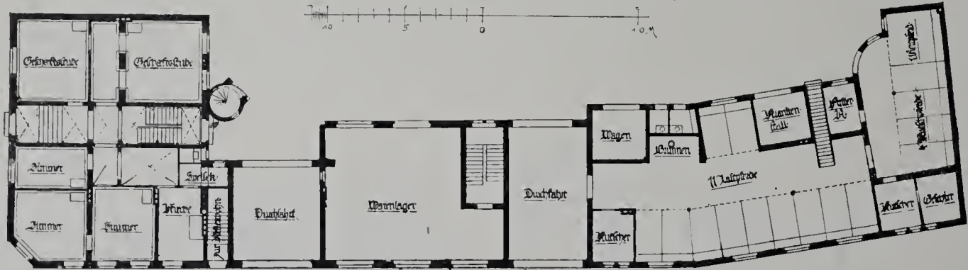
Erdgeschoss.
