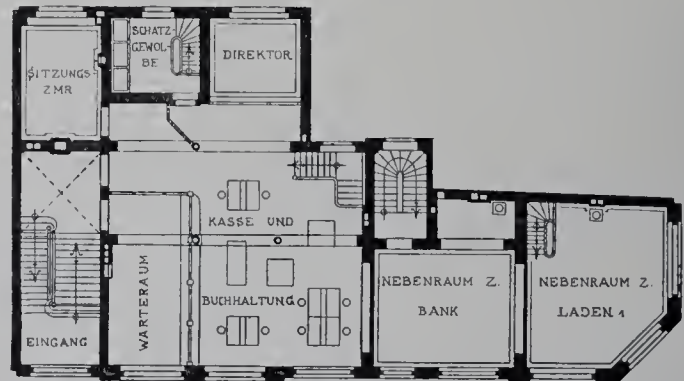
Erdgeschoss.
