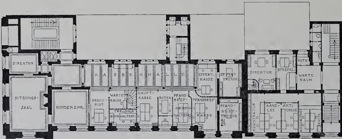
Erdgeschoss.
