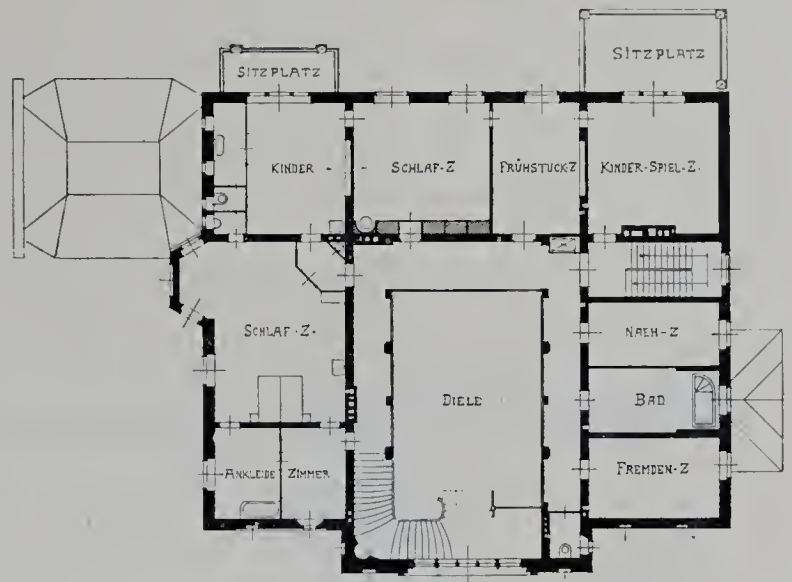
—I. STOCK—
