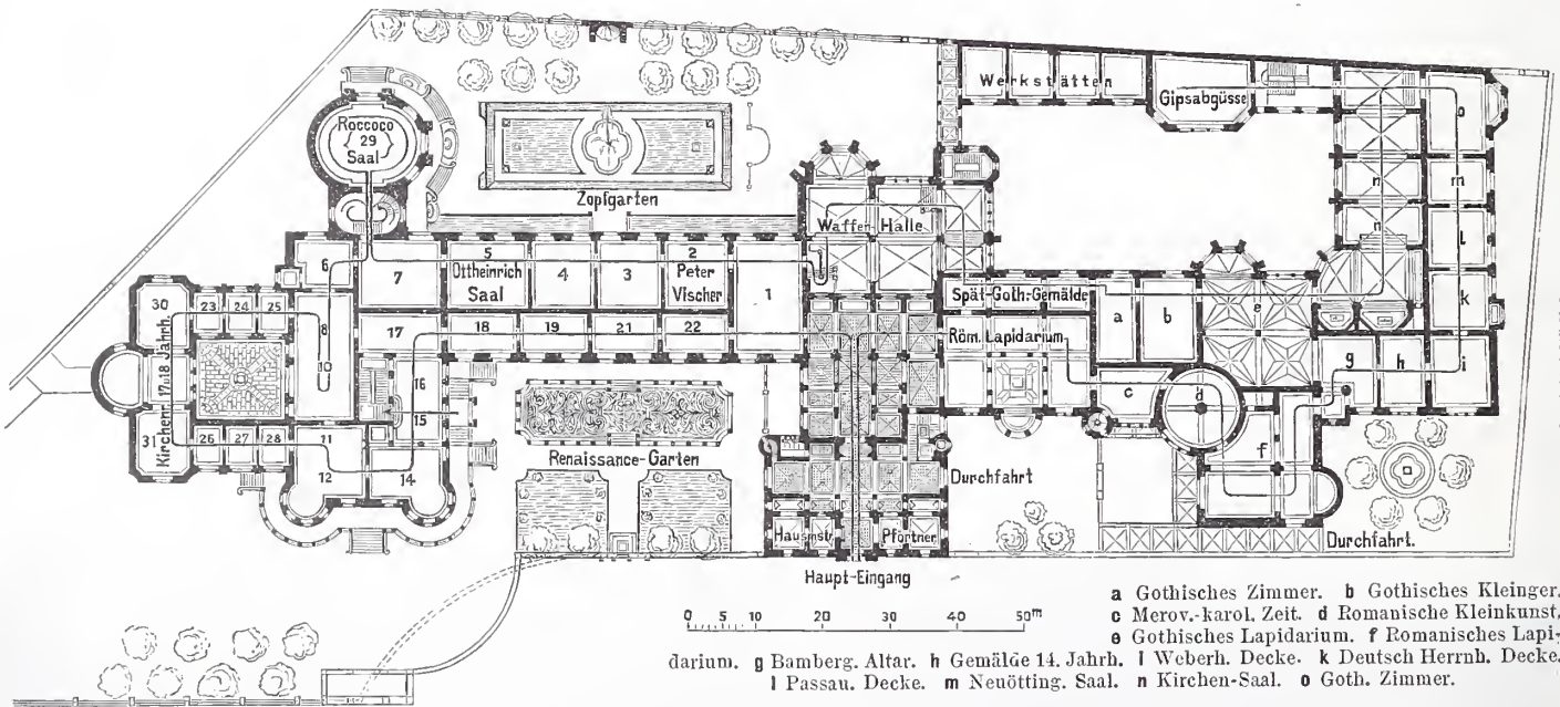
Erdgeschoss.
