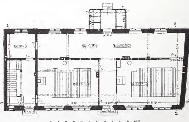
Abb. 4. Erdgeschofs.
