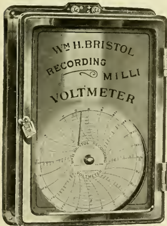
Figure 1—Recording Milli-Voltmeter.
