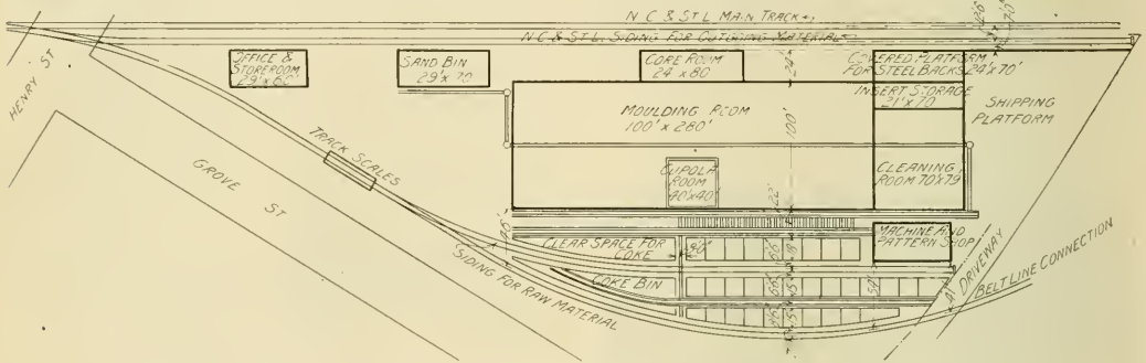
Foundry of the American Brake Shoe & Foundry Company at Chattanooga, Tenn.—General Plan.
