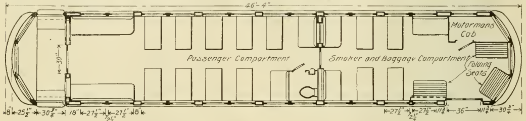
Choctaw Railway Cars—Floor Plan and Seating Arrangement.
