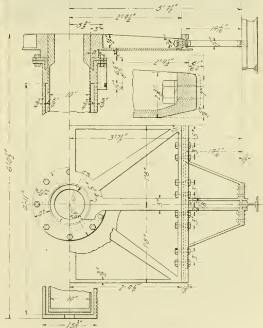
York Shops—Details of Hydraulic Pit Hoist.
