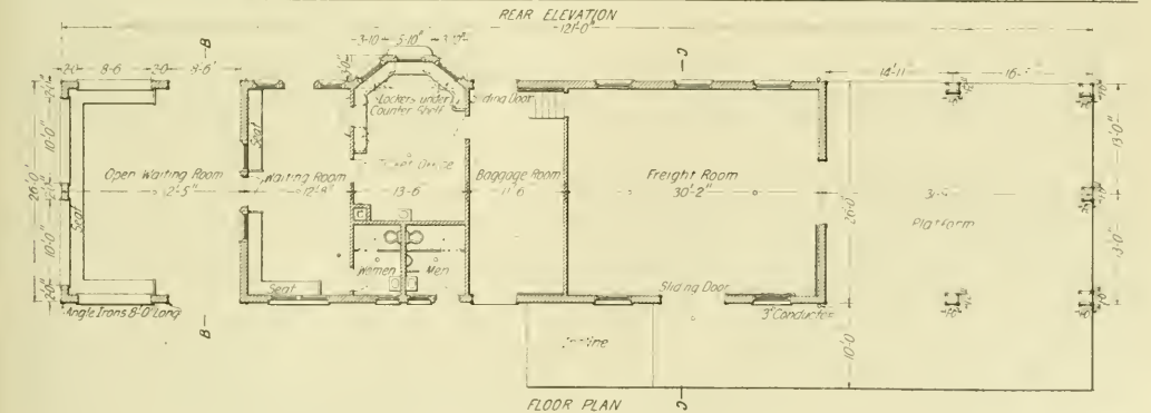
Pacific Electric Railway—Floor Plan, Elevation and Section of Monrovia Station.
