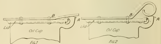
Oil Cup Lid—Showing Original Flat Spring and Improved Spring with Long Bend.
