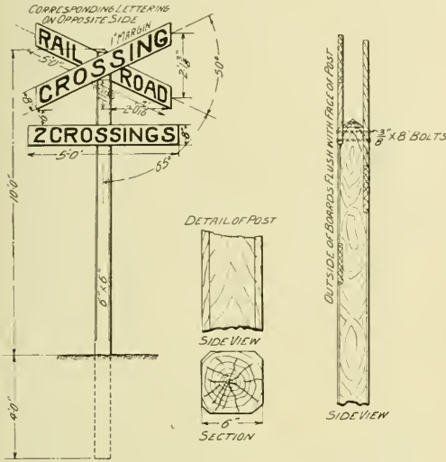
Indiana Union Traction Company—Sign Post for Highway Crossing Two Railways.
