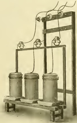
Electrolytic Arresters.
