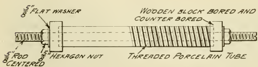
Allegheny Shop Practice—Scheme for Winding Heater Coils.
