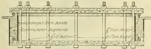
Repairing Commutators—Figure 2.
