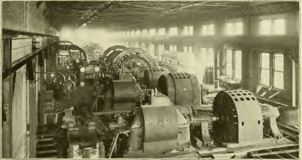
Westinghouse Double-Flow Turbines—Interior of Brunot Island Station of the Pittsburg Railways Company, Showing Turbines During Erection.
