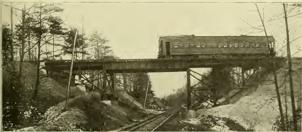
Washington Baltimore & Annapolis—Double-Track Steel Viaduct over Steam Road.
