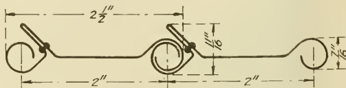
Erwood's Reversible Rolling Door—Section Showing Two Slats.
