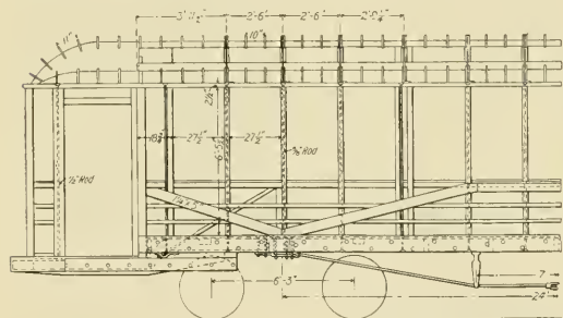
Aurora Elgin & Chicago Cars—Side and Floor Framing.
