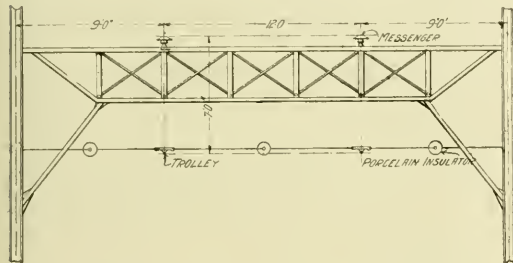
Syracuse Lake Shore & Northern Railroad—Plan of Steady Attachment at Catenary Bridges.
