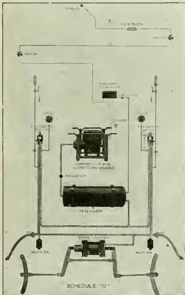
Diagram of National Straight Air Brake Equipment
