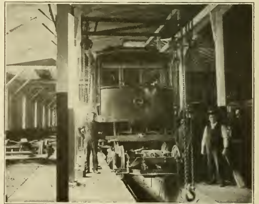
Tampa Shops—Hoist and Chain Blocks for Handling Car Bodies.
