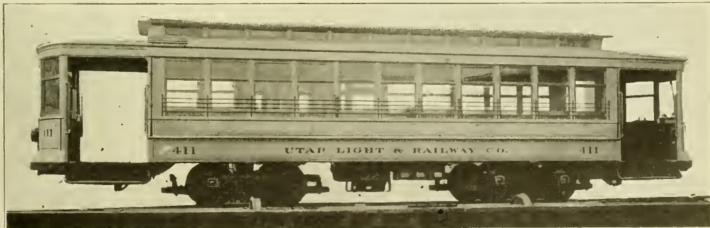
Semi-Convertible Cars for Salt Lake City—Side View.
