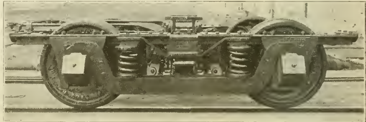
Waterloo Cedar Falls & Northern—Truck for Combination Car.
