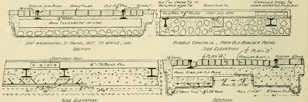
Substructures for Tracks in Streets—Sections Above Showing Rails, Wood and Carnegie Steel; Sections Below Showing Beam Construction with Kahn Reinforcement Under Joint and Drainage.
