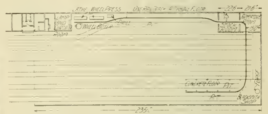
Tampa Shops—Plan Showing Location of Overhead Runway for Trolley Hoist.
