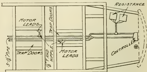
Allegheny Shop Practice—Arrangement of Conduits for Motor Wiring.
