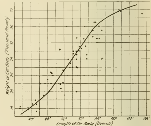
Typical Traction Cars—Curve 3. Relation of Length to Weight.
