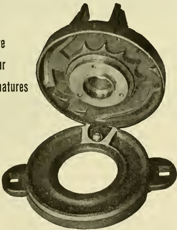
Regulator open
