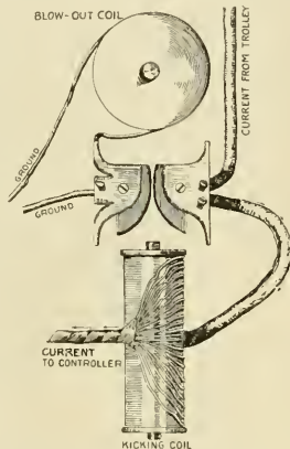
Sketch of the Clark Lightning Arrester.
