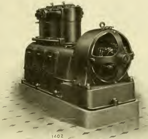
150 Cubic Foot "3VS" Type Air Compressor with Direct Current Motor
