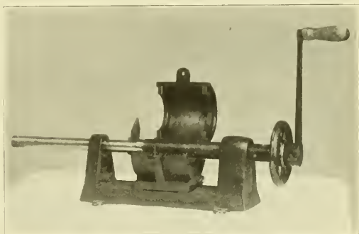
Hand-Driven Lathe for Boring Armature Boxes.
