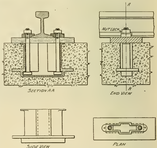
Beilharz Housing for Embedded Bolts.
