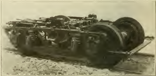
New Elevated Cars for Brooklyn Rapid Transit Company— Side View of Motor Truck.
