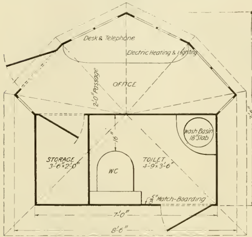
Chicago City Railway—Floor Plan of Terminal Booth.
