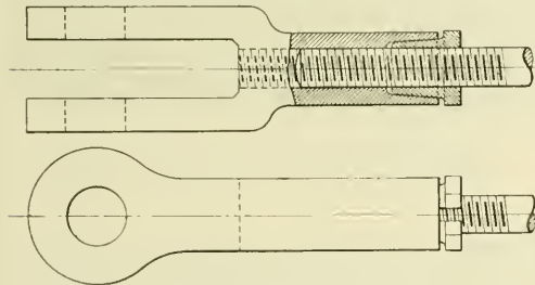
The Hillman Locked Clevis.
