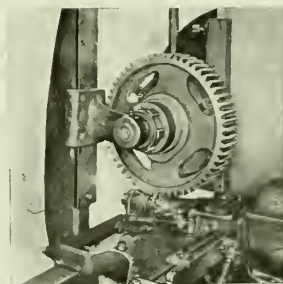
Gear Mounted in Gear Cutting Machine. Roughing and Finishing Cutter Operating Simultaneously.
