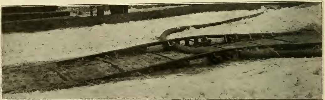
Philadelphia Rapid Transit Hose Bridge—View When in Service.
