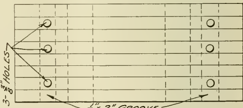
Allegheny Shop Practice—Details of Double Thickness Trap Doors.
