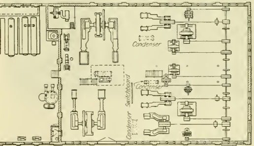
Jacksonville Power Station—Plan After Remodeling.
