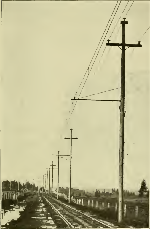
Oregon Electric Railway—Overhead Construction on Tangent.
