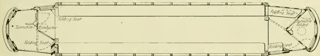
Pay-As-You-Enter Car—Platform Arrangement for Double-End Operation.
