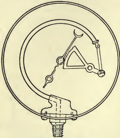
FIG. 233—STEAM GAUGE
