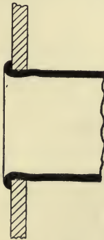
FIG. 240—FLUE EXPANDED WITH PROSSER EXPANDER
