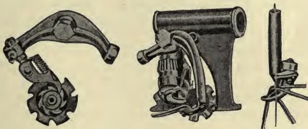
FIG. 113—A TWINE DISK. A KNOTTER COMPLETE—A KNOTTER HOOK
