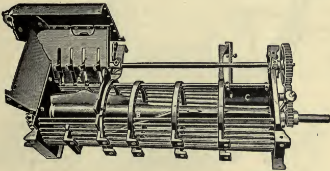
FIG. 173—SHELLING MECHANISM OF CYLINDER SHELLER
