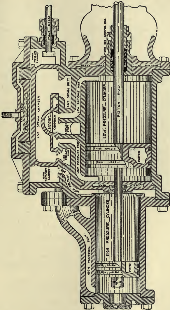
FIG. 277—CYLINDERS OF WOOLF TANDEM-COMPOUND ENGINE
