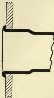
FIG. 241—FLUE EXPANDED WITH DUDGEON EXPANDER
