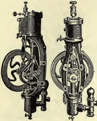
FIG. 228—INDEPENDENT PLUNGER PUMP
