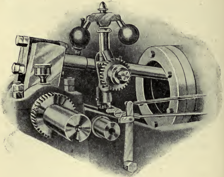
FIG. 300—BALL GOVERNOR
