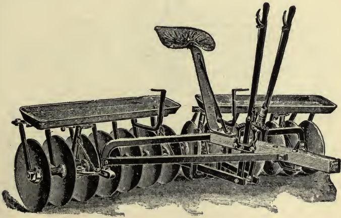
FIG. 55—A TWO-LEVER DISK HARROW. SCRAPPERS OPERATED BY THE FEET
