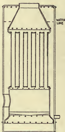
FIG. 213—VERTICAL BOILER WITH SUBMERGED FLUES
