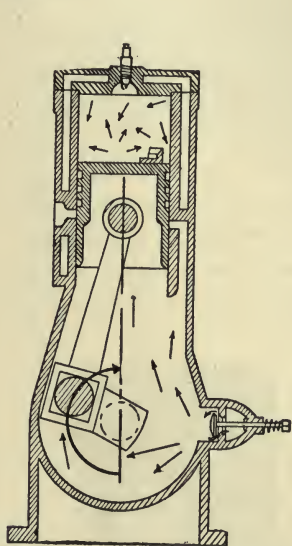
FIG. 287—SUCTION, COMPRESSION AND IGNITION STROKE OF TWO-CYCLE ENGINE
