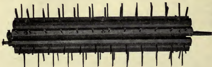
FIG. 150—A MANURE SPREADER BEATER
