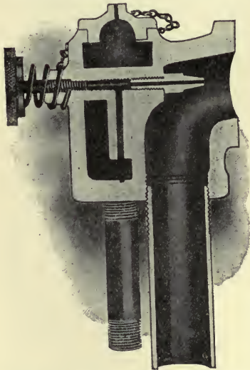
FIG. 303—CONSTANT-LEVEL CARBURETOR
