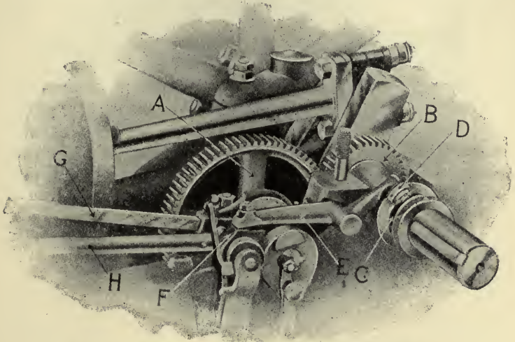
FIG. 297—MECHANISM FOR HIT-OR-MISS GOVERNOR
