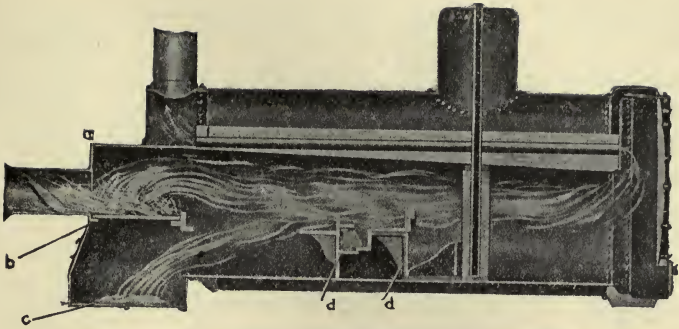
FIG. 223.—STRAW BURNER RETURN-FLUE BOILER
