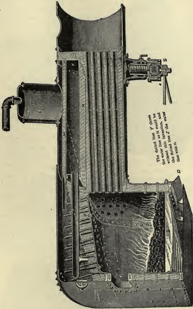
FIG. 220—BOILER WITH REAR END OF CROWN SHEET LOWER THAN FRONT END
