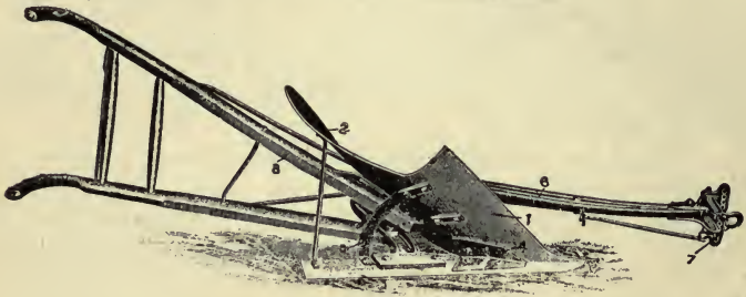
FIG. 34—AN UNDER VIEW OF THE MODERN STEEL PLOW, SHOWING ITS CONSTRUCTION
