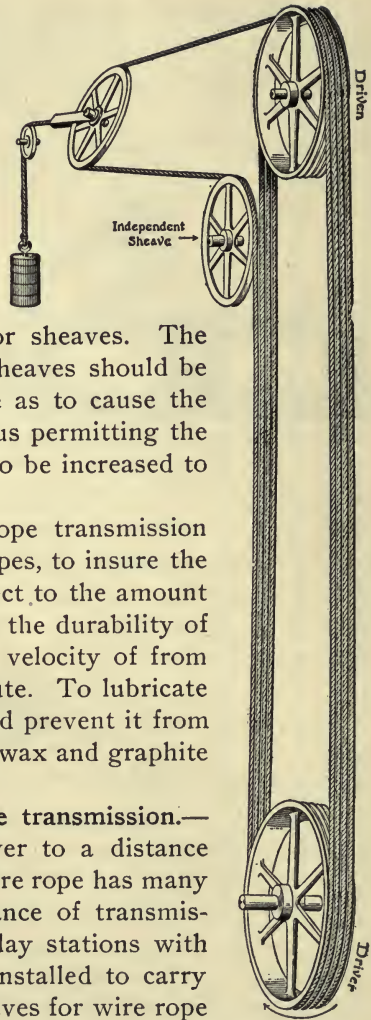
FIG. 20—TRANSMISSION OF POWER BY ROPES
