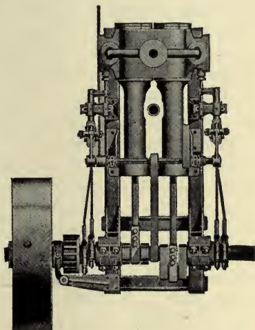
FIG. 276—DOUBLE-CYLINDER ENGINE
