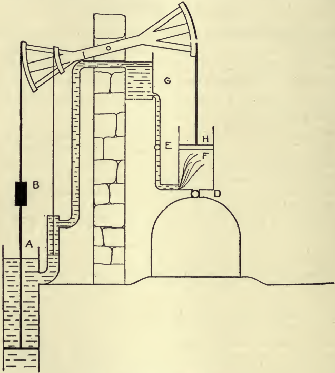
FIG. 242—NEWCOMEN'S ENGINE
