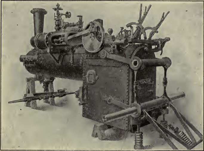
FIG. 323—REAR-MOUNTED ENGINE WITH RADIUS AND CROSS LINKS
