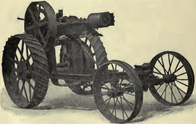
FIG. 326—FRAME-MOUNTED ENGINE
