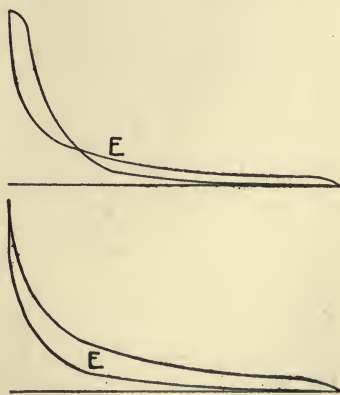
FIG. 314—TOO EARLY IGNITION
