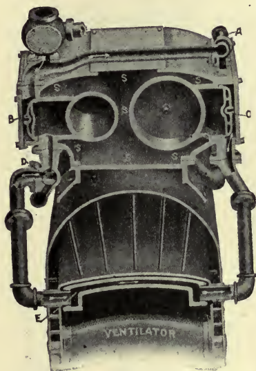
FIG. 278—CROSS-COMPOUND ENGINE
