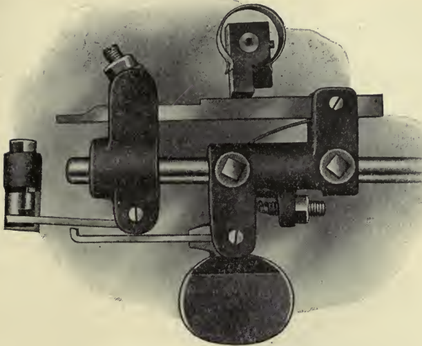
FIG. 301—PENDULUM GOVERNOR
