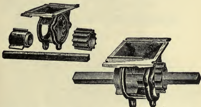
FIG. 78—A FORCE-FEED DEVICE. THE FEED IS VARIED BY EXPOSING MORE OR LESS OF THE FLUTED FEED SHELL
