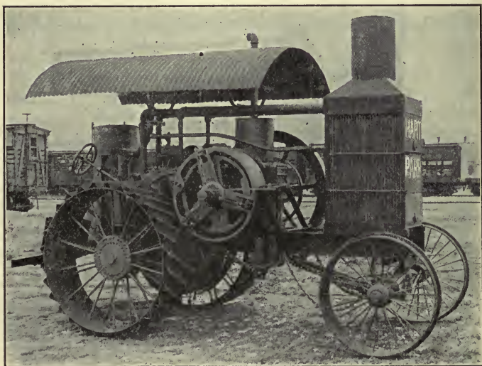
FIG. 338—TRACTION ENGINE WHICH REVERSES IN THE CLUTCH
