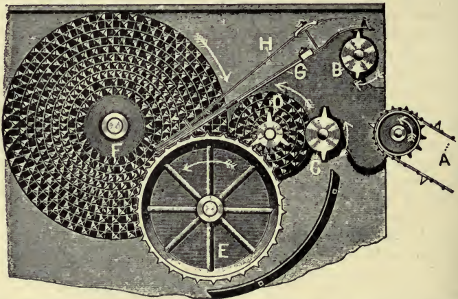
FIG. 172—SHELLING MECHANISM OF THE PICKER OR SPRING SHELLER. A , FEED CHAIN; B , C , BEATERS; D , F , PICKER WHEELS; E , BEVEL RUNNER; G , RAG IRON; H , SPRING
