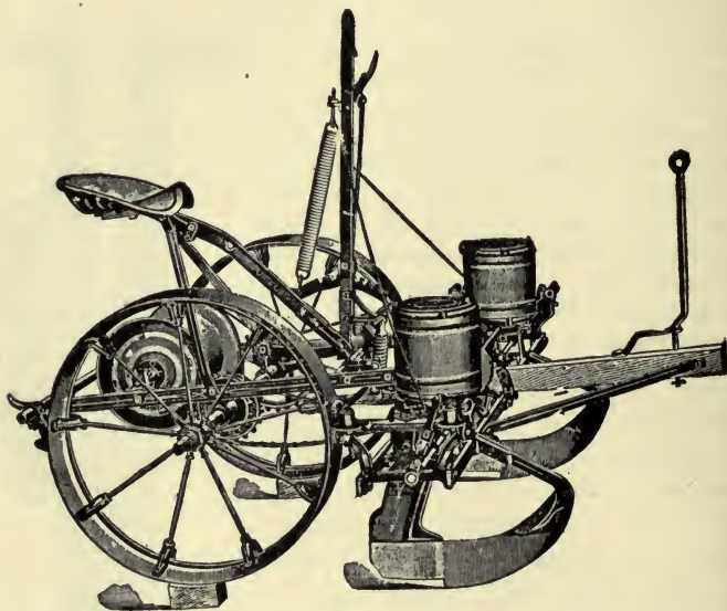
FIG. 89—A MODERN CORN PLANTER WITH LONG CURVED FURROW OPENERS, VERTICAL CHECK HEAD, AND OPEN WHEELS
