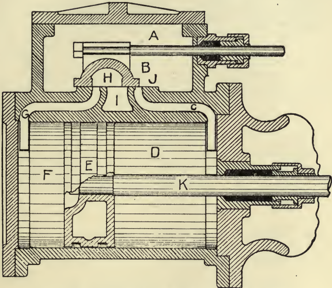
FIG. 243—CYLINDER AND VALVE OF STEAM ENGINE
