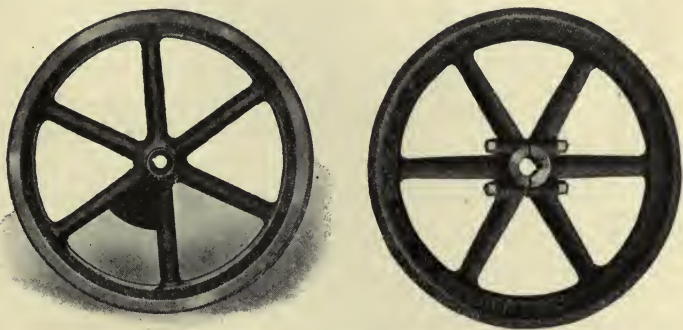
FIG. 295—FLYWHEELS
