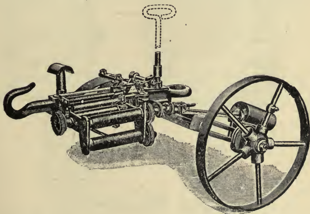
FIG. 11—A GERMAN RECORDING DYNAMOMETER WHICH HAS THE REEL DRIVEN BY A WHEEL TRAVELING ON GROUND
