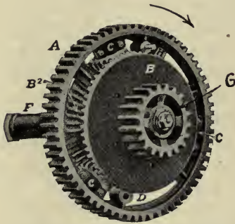
FIG. 335—COMPENSATING GEARS
