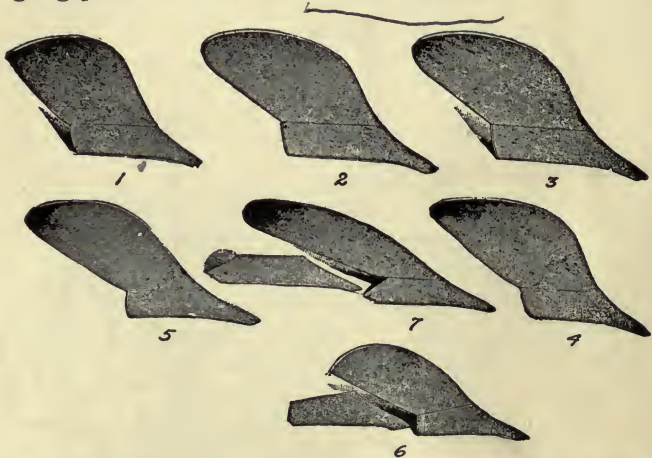
FIG. 40—TYPES OF PLOW BOTTOMS. NO. 1 IS THE STUBBLE OR OLD GROUND BOTTOM. NO. 7 IS THE BREAKER BOTTOM FOR TOUGH NATIVE SODS. NOS. 2, 3, 4, 5, AND 6 ARE INTERMEDIATE TYPES FOR GENERAL PURPOSE PLOWS
