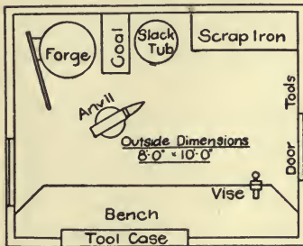
FIG. 375—ARRANGEMENT OF A SMALL SHOP
