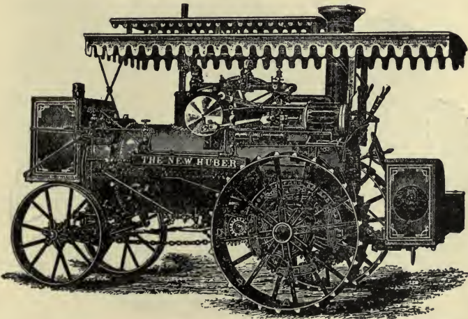
FIG. 324—UNDER-MOUNTED ENGINE
