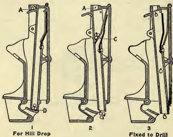
FIG. 93—A TRIPLE VALVE MECHANISM SHOWING HOW THE CORN IS RELEASED AT THE HEEL OF THE FURROW OPENER
