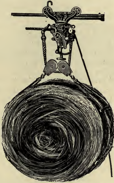
FIG. 142—A LIGHTER SLING CARRIER LOADED WITH A SLING LOAD OF HAY
