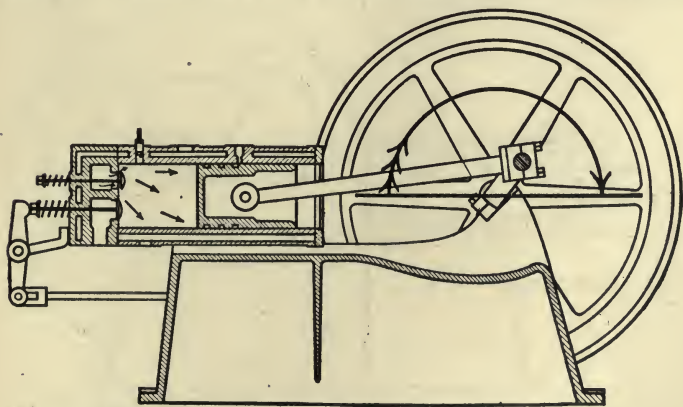
FIG. 281—SUCTION STROKE OF FOUR-CYCLE ENGINE
