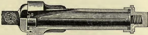
FIG. 185—A LONG-DISTANCE BUGGY AXLE. NOTE THE PROVISION MADE TO EXCLUDE DUST AND DIRT
