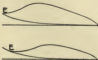
FIG. 313—TOO LATE IGNITION
