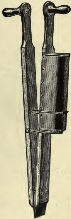
FIG. 88—A HAND CORN PLANTER. THE CORN IS DRAWN FROM UNDER THE SEED BOX BY A SLIDE UPON CLOSING AND OPENING THE HANDLES
