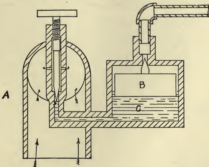
FIG. 305—PRINCIPLE OF THE FLOAT-FEED CARBURETOR
