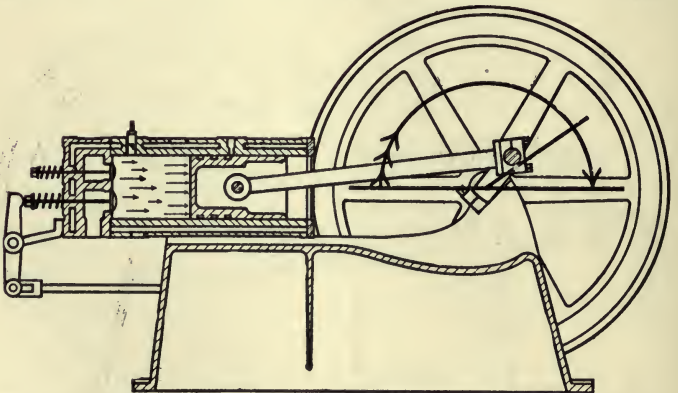
FIG. 283—EXPANSION AND RELEASE STROKE OF FOUR-CYCLE ENGINE
