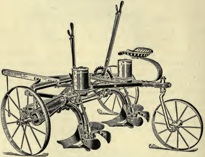
FIG. 101—A TWO-ROW LISTER
