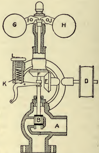
FIG. 272—SECTIONAL VIEW OF THROTTLING GOVERNOR
