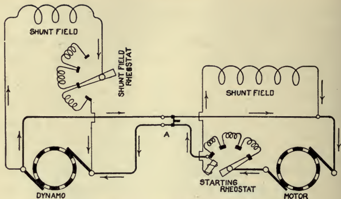
FIG. 368—WIRING SYSTEM FOR DYNAMO AND MOTOR
