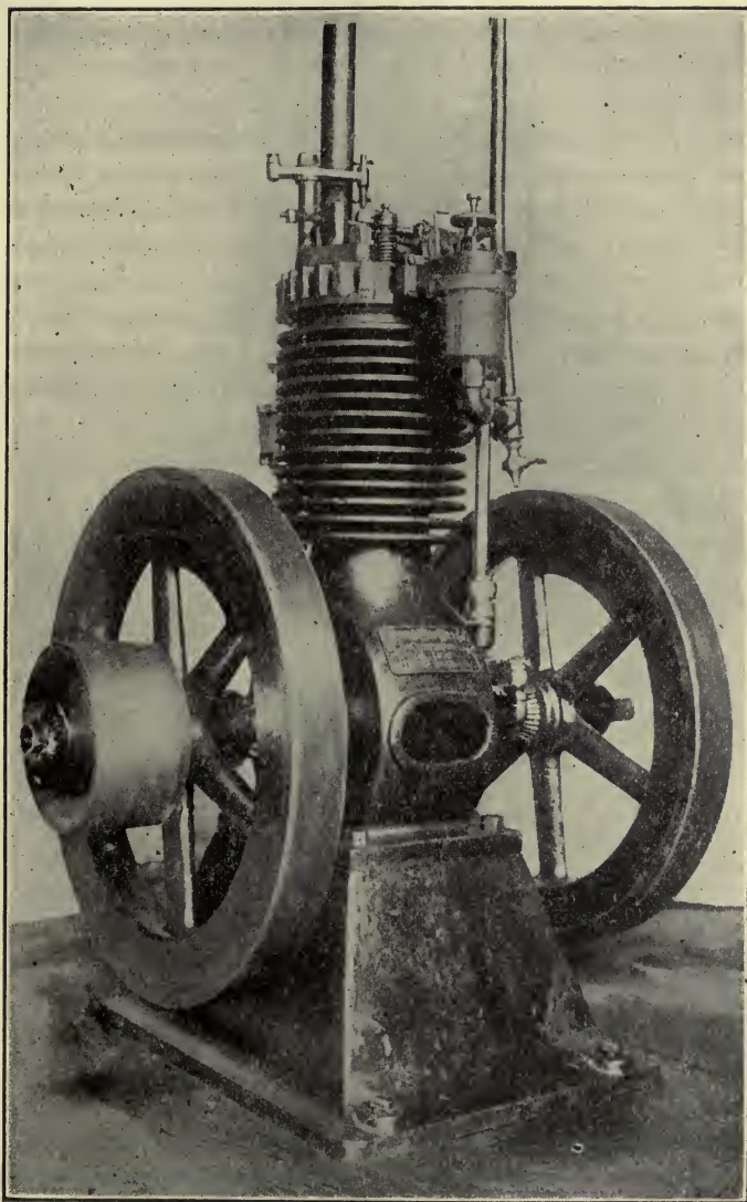
FIG. 310—AIR-COOLED ENGINE
