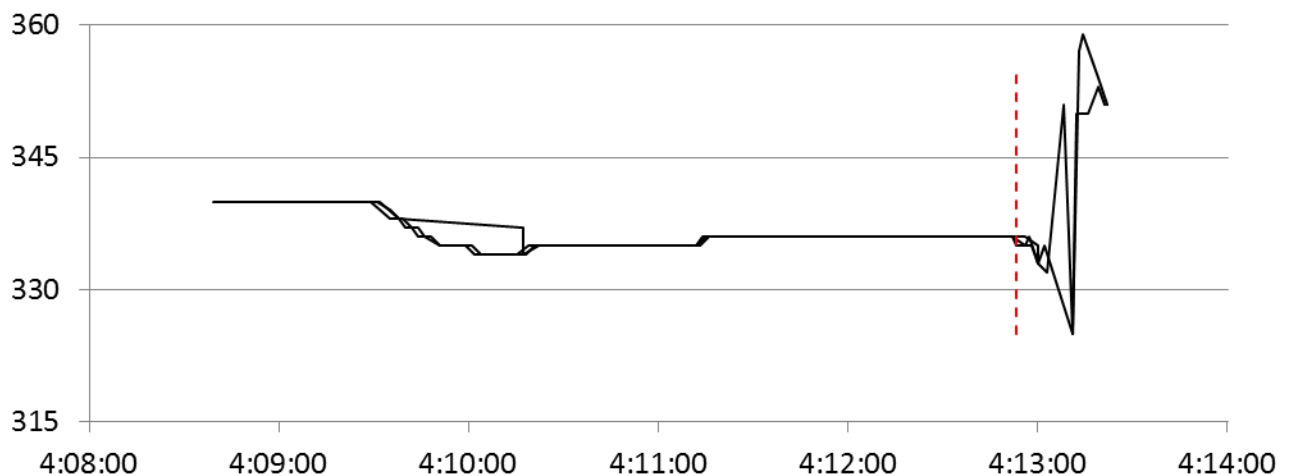
Three Radars Tracking Flight KGL9268 Heading
