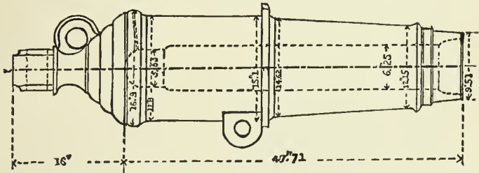
32-Pound Carronade, 1779.—Weight, 17 cwt.
