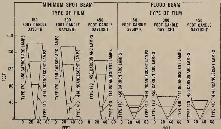
FIGURE 2. Scale diagram showing projection distance, beam spread and beam diameter for equivalent photographic effect at center of beam.
