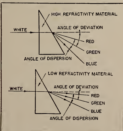
FIG. 18. Refraction and dispersion.
