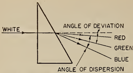
Showing action of white light entering material of low refractive index.
