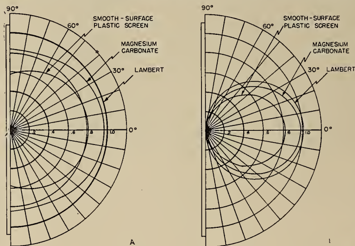
FIGURE 4 Brightness and intensity patterns for a "perfect" screen and the smooth surface plastic screen. On the brightness diagram, A, the radial scale gives foot-Lamberts per foot-candle; on the intensity diagram, B, radial scale gives candles per \pi square feet of screen area per foot-candle of illumination.
