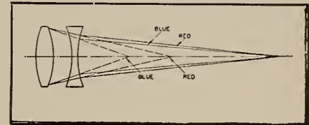
FIG. 21. Longitudinal achromatization.
