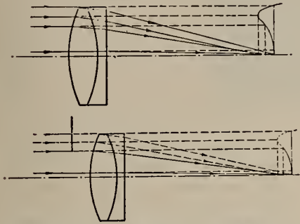
CORRECTION OF SPHERICAL ABERRATION. Top to bottom: Figs. 6 and 7.
