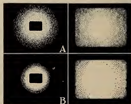
FIG. 3. The aperture "spot" and resulting screen illumination produced by A a spherical mirror, and B an ordinary elliptical mirror. The light-scattering effect of spherical aberration is seen in A ; and the effect of non-uniform brilliancy distribution in the H-I crater in B .
