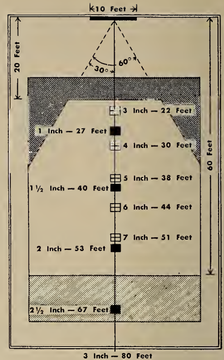
Da-Lite screen viewing chart, Open, ruled squares relate to the positioning of a 35-mm slide projector, with various lenses; solid black squares relate to a 16-mm motion picture projector, with various lenses. Unshaded portion denotes, of course, preferred viewing area.
