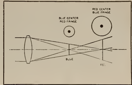
FIG. 20. Longitudinal chromatic aberration.
