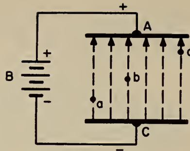
FIG. 10. Electrons placed in electrostatic field between two charged plates and acted upon by force of the field.
