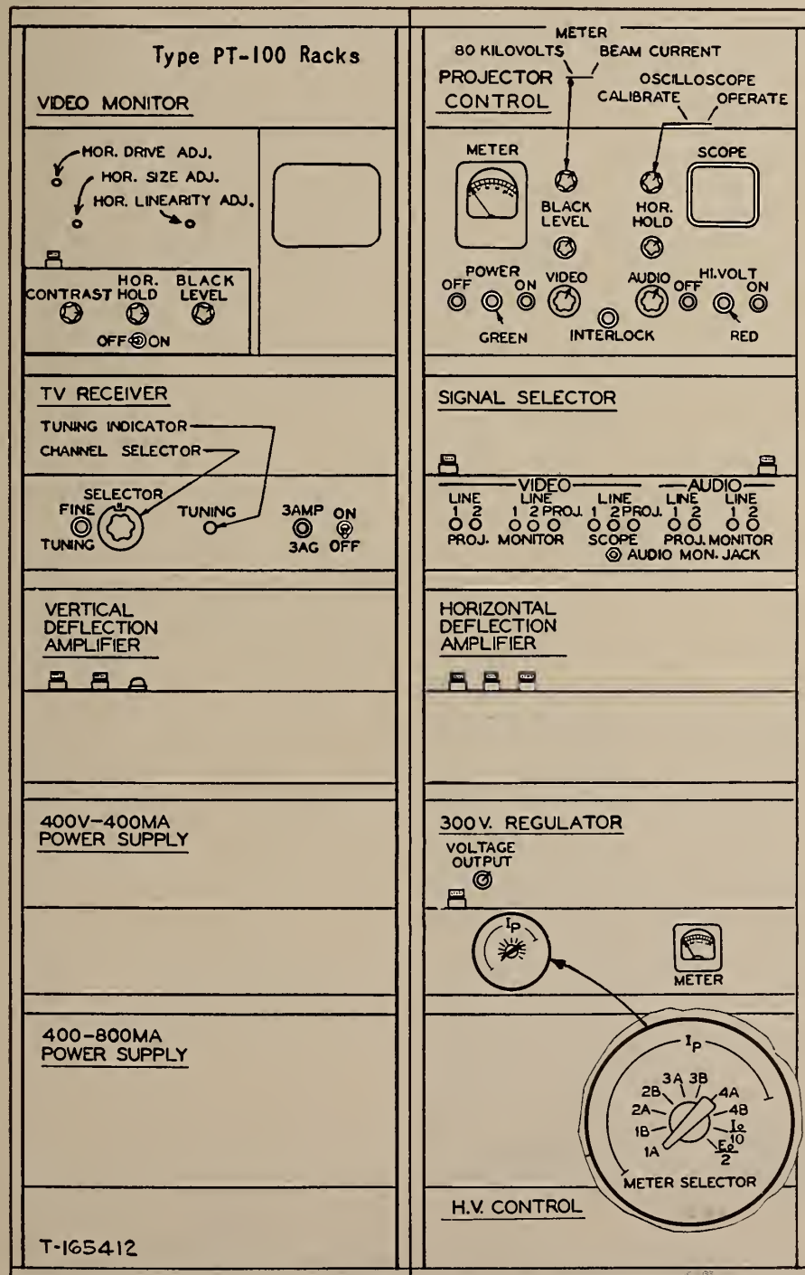
Figure 1 - Operating Controls on Theatre Television Projector
