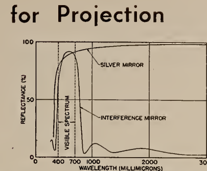
The spectral reflectance of a multi-layer interference film compared with that of the conventional silver film.
