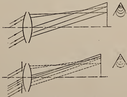
ILLUSTRATING COMA Top to bottom: Figs. 8 and 9.
