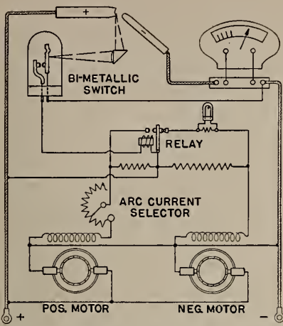
FIG. 3. Simplified arc control circuit diagram.
