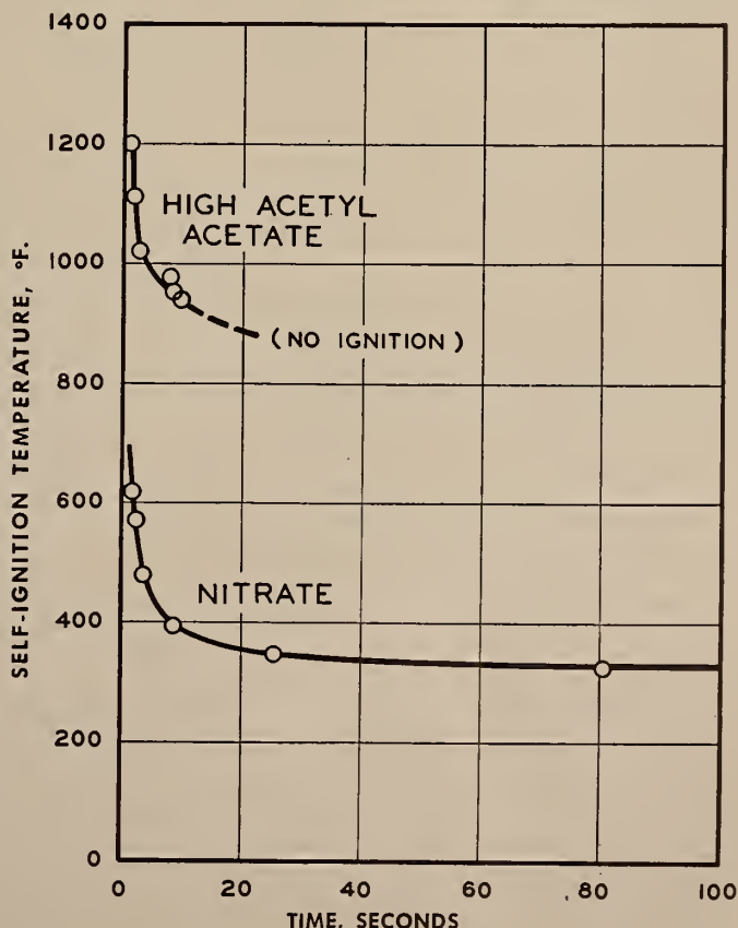
FIGURE 1 Self-ignition temperature in air of Eastman nitrate and high acetyl acetate (safety) motion picture positive film support. American Standards Assoc. test method.
