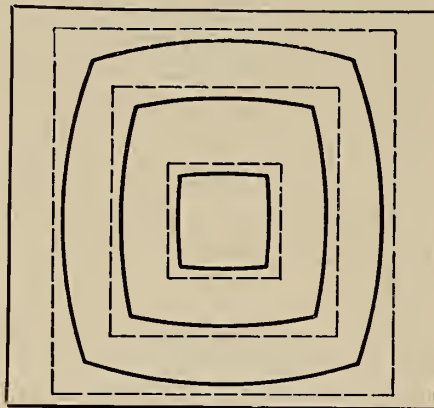
FIG. 15. 'Barrel' distortion.
