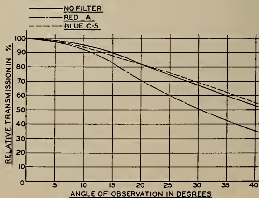
FIGURE 2 Typical brightness fall-off curves— goniophotometer measurements.
