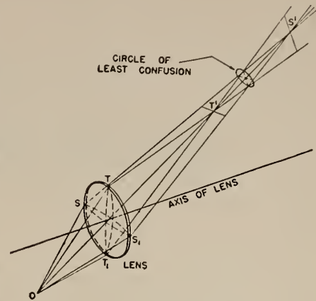
FIG. 10. Astigmatism.
