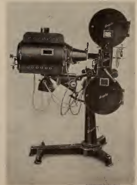
Old standby thru the years—the Regular Simplex (1910). Note old framing lever. The light source shown here is the first McAuley reflector lamp.
