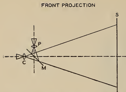
FIG. 3. Schematic drawing of a set-up for front projection.
