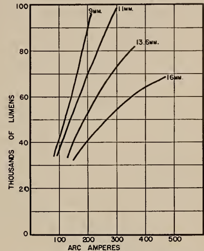
FIG. 4. Relation between screen light and arc current at an optical speed of F:2.0.
