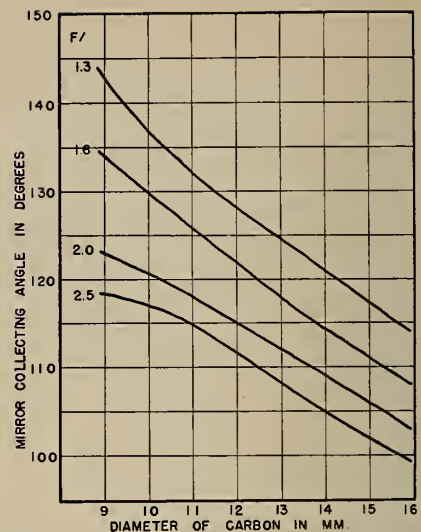
FIG. 7. Collecting angle giving maximum screen light.
