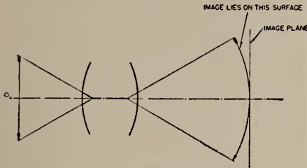
FIG. 12. Field curvature.
