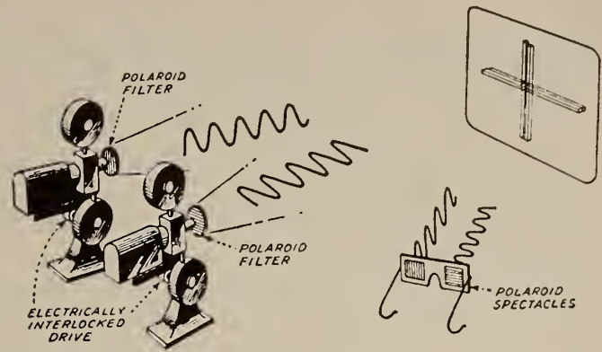
FIGURE 2 Diagram of a double projector installation using Polaroid filters on the projectors, plus viewing spectacles and projector interlock.
