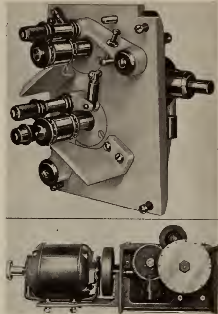
Top: entire upper and lower sprocket assembly in gear box removed as a unit from operating side. Pad roller assembly is held in place by a new compression-type coil spring lock.
