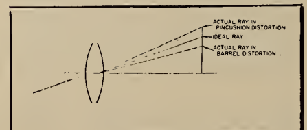
FIG. 16. Distortion.
