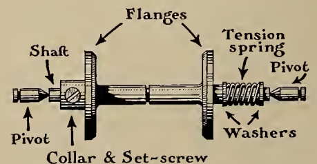
FIG. 3. A standard guide-roller assembly. Note the set-screw by means of which the roller may be adjusted laterally.
