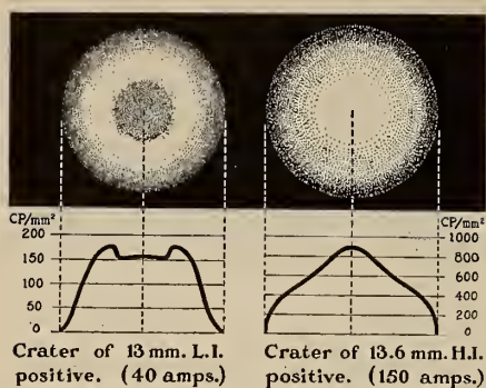
FIG. 2. Brilliancy distribution in low- and high-intensity arc craters.
