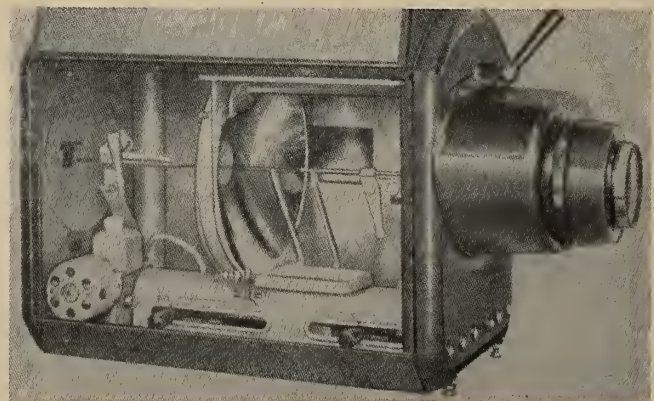
Fig. 5. The Zeiss Ikosol honeycomb-condenser lamp. Note lightness and simplicity of this lamp.
