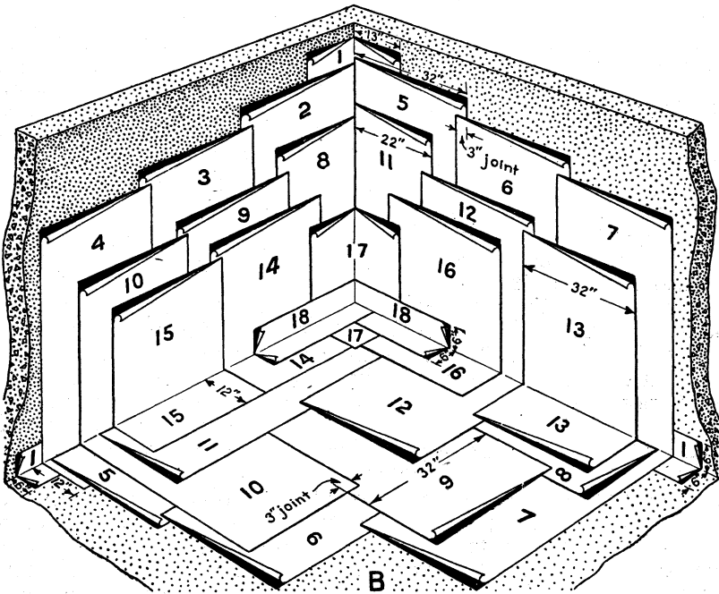
FIGURE 15.—Membrane waterproofing : A, Two layers of 36-inch felt, spaced 17 inches, overlapped 19 inches, jointed 2 inches; numbers show order of applying sheets. B, three layers of 32-inch felt, jointed 3 inches; intermediate floor layer crosswise of bottom and upper layers; wall sheets overlapped 22 inches, spaced 10 inches
