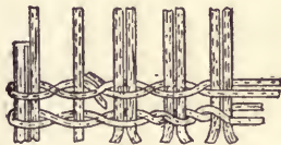
Fig. 93.—Working Pair of Rods on Fetch-rods.
