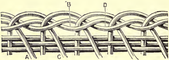
Fig. 32.—Rope Edge: Second Stage.
