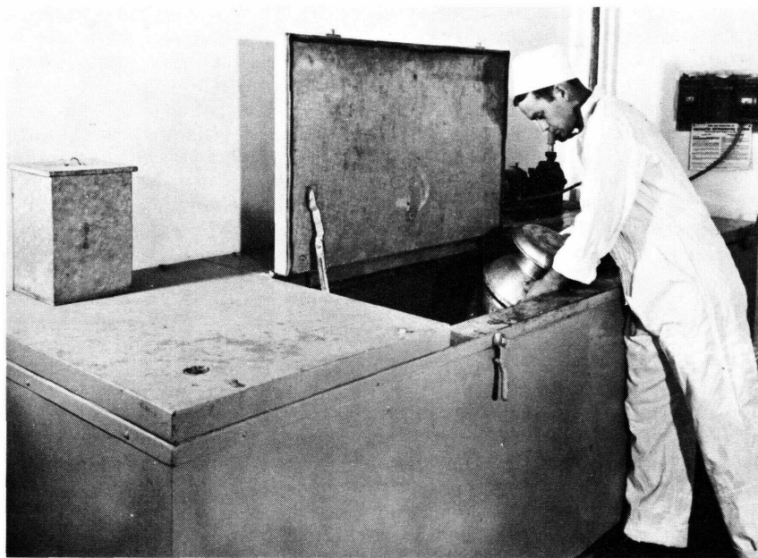
FIGURE 14.—A mechanically refrigerated storage box for cans of milk.
