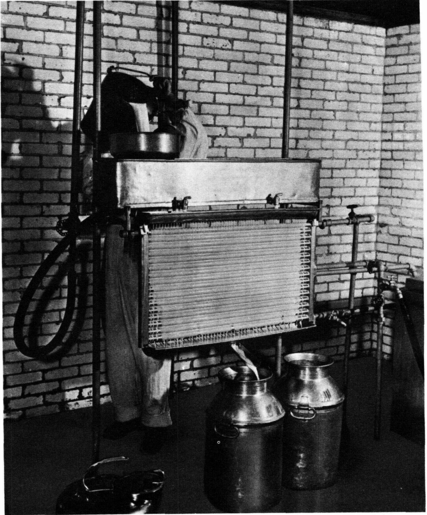
FIGURE 13.—Cooling milk with a surface cooler. Here the milk is strained as it enters the cooler supply tank. Cold water for the cooler is piped from the can storage tank at the right.
