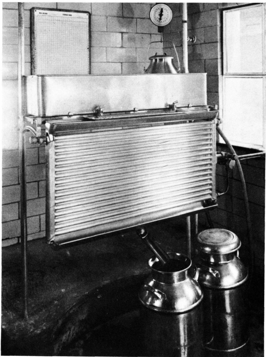
FIGURE 7.—A well-arranged milk handling room. A scale and weight chart are in the rear. Strainer is in upper trough of cooler.
