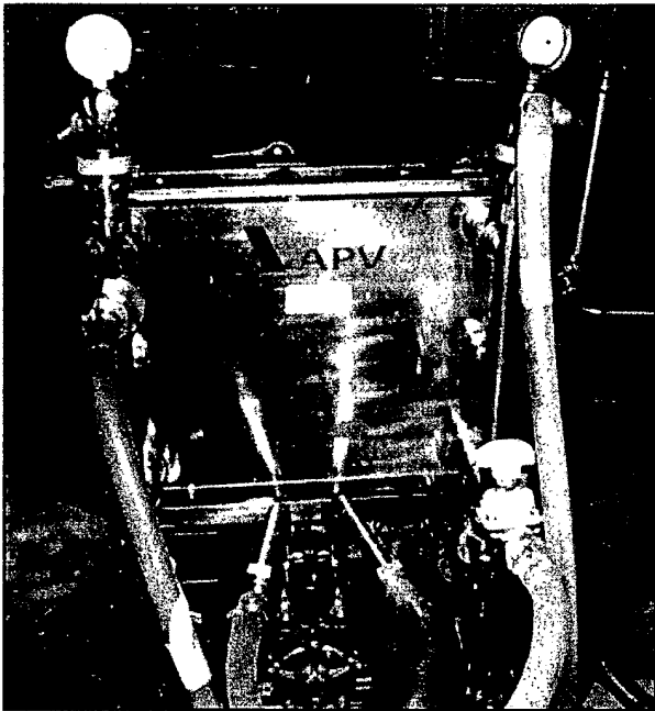
Figure 5. Plate filter press.
