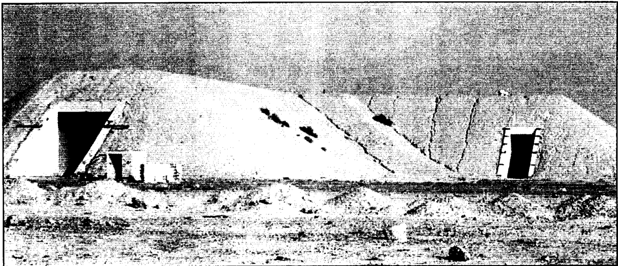
Figure 12. Typical side view of a cruciform shaped bunker.
