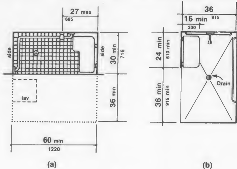
Fig. 57 Roll-in Shower with Folding Seat
