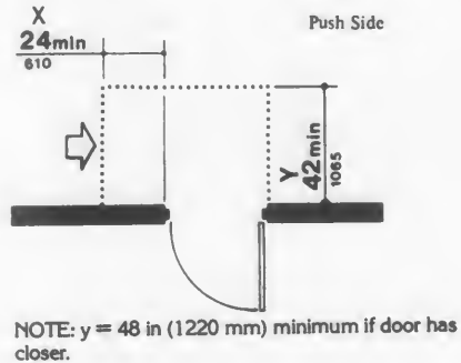
(c) Latch Side Approaches — Swinging Doors
