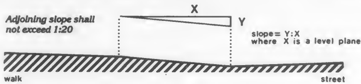
Fig. 11 Measurement of Curb Ramp Slopes
