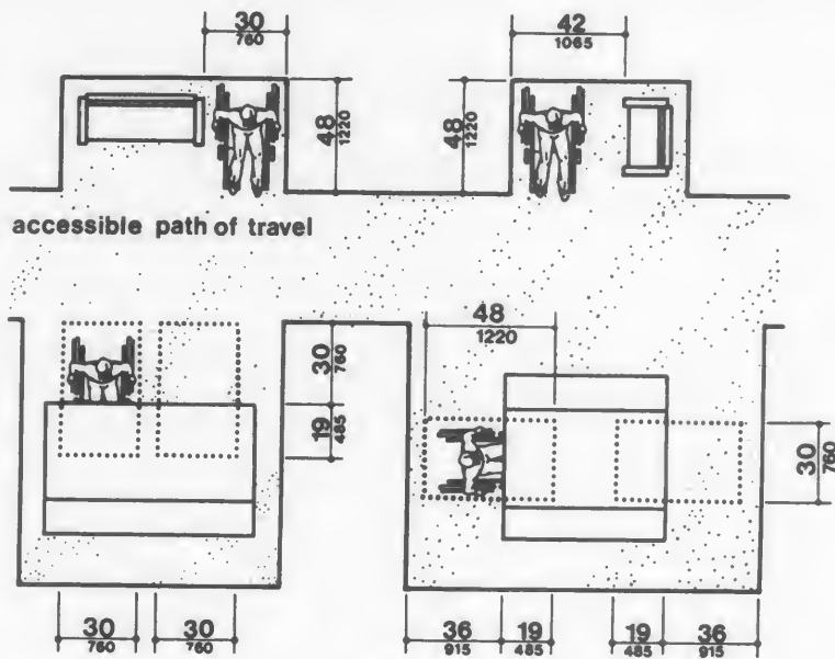
Fig. 45 Minimum Clearances for Seating and Tables
