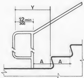
(c) Extension at Bottom of Run
