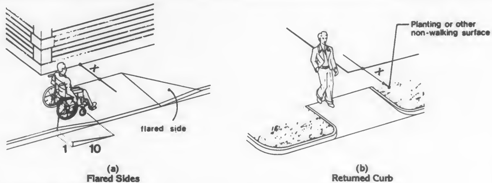
Fig. 12 Sides of Curb Ramps
