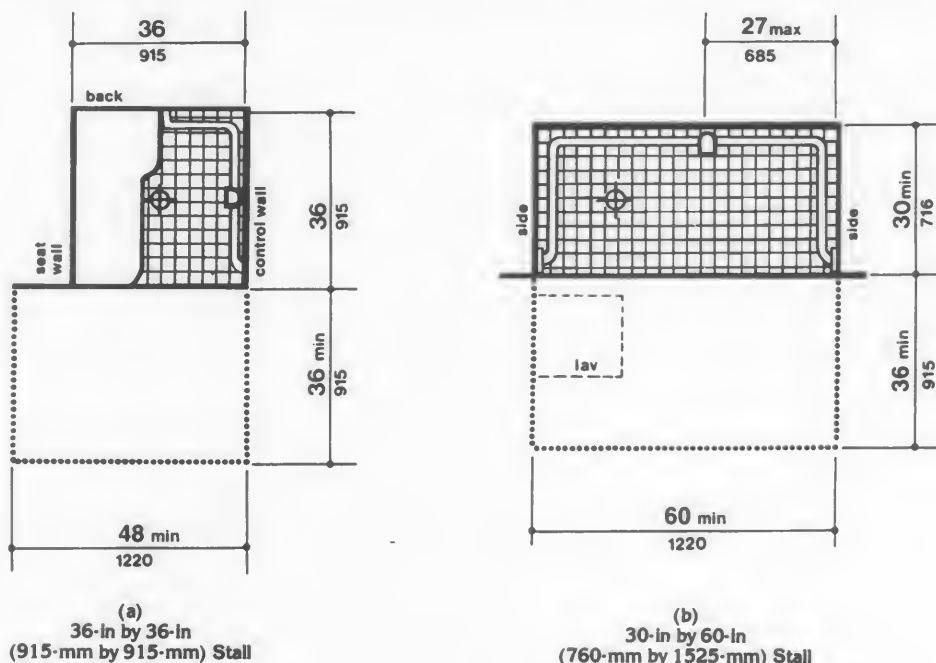
Fig. 35 Shower Size and Clearances
