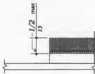
Fig. 8 (f) Carpet Pile Thickness
