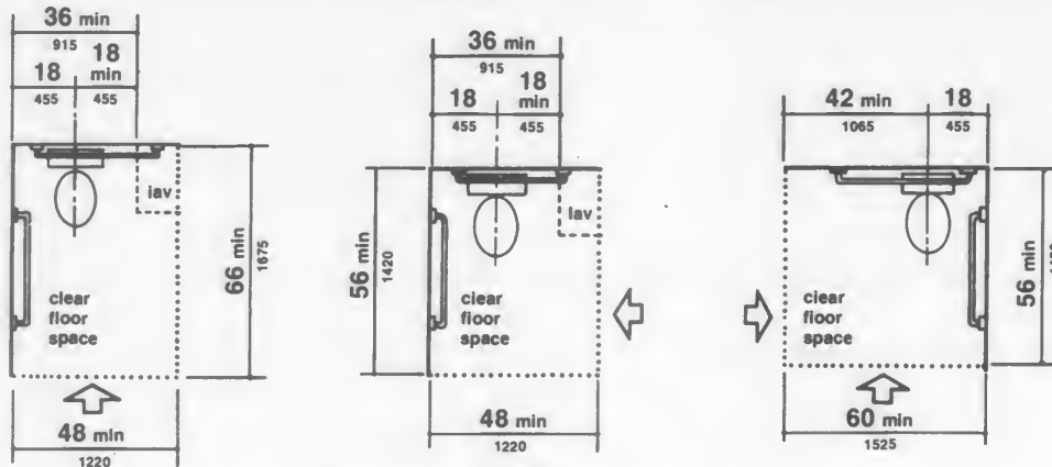
Fig. 28 Clear Floor Space at Water Closets
