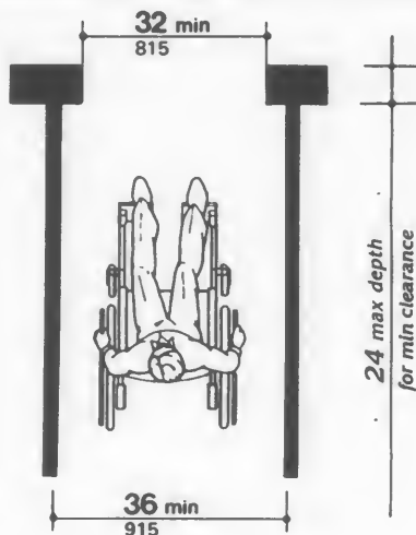
Fig. 1 Minimum Clear Width for Single Wheelchair
