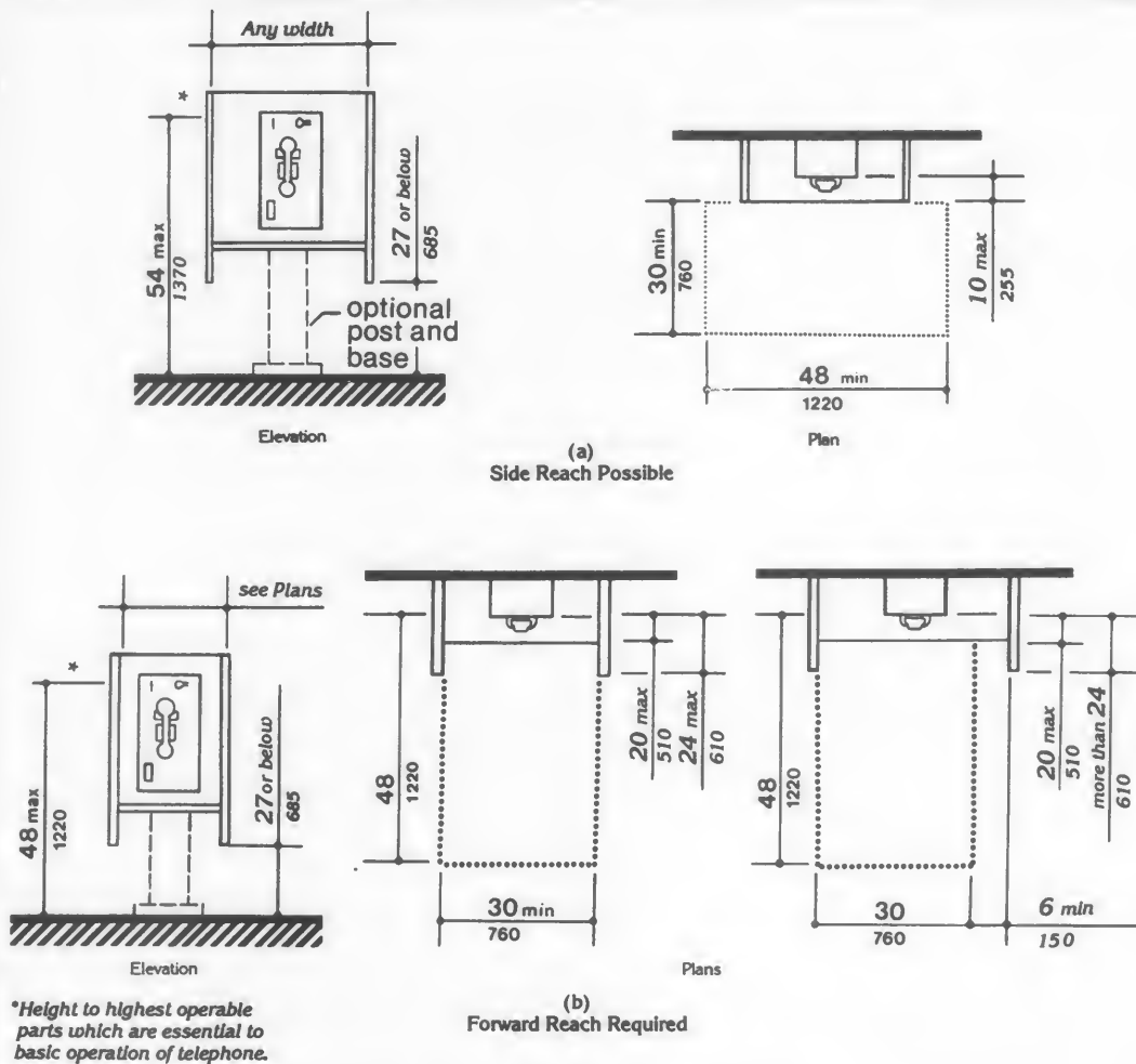
Fig. 44 Mounting Heights and Clearances for Telephones
