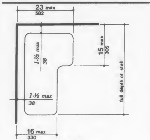
Fig. 36 Shower Seat Design
