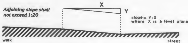
Fig. 11 Measurement of Curb Ramp Slopes
