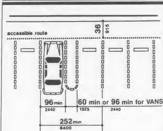
Fig. 9 Dimensions of Parking Spaces
