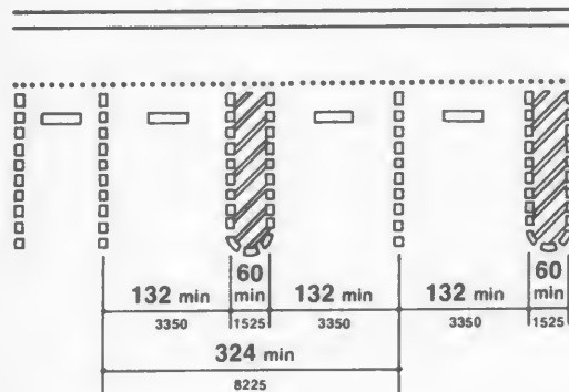
(b) Universal Parking Space Design
