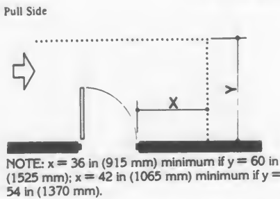
(a) Front Approaches — Swinging Doors
