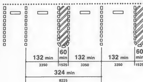
(b) Universal Parking Space Design
