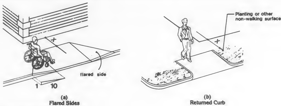
Fig. 12 Sides of Curb Ramps
