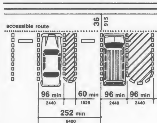
(a) Van Accessible Space at End Row
