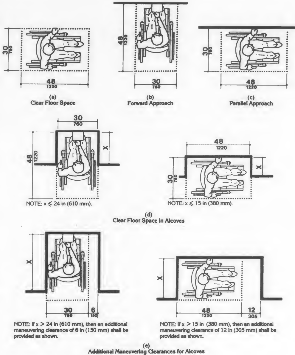
Fig. 4 Minimum Clear Floor Space for Wheelchairs
