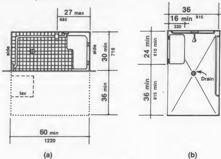
Fig. 57 Roll-in Shower with Folding Seat
