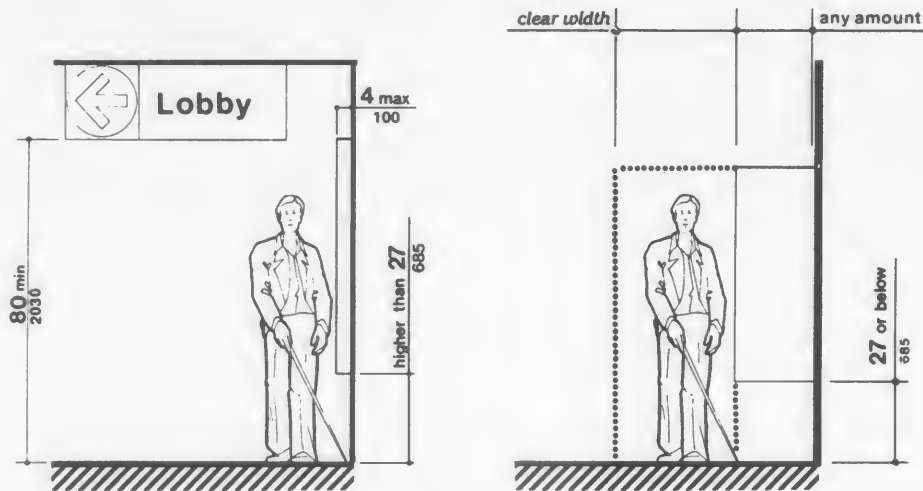
Fig. 8 (a) Walking Parallel to a Wall
