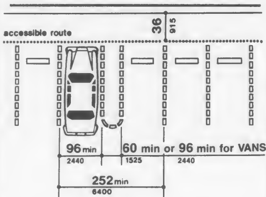
Fig. 9 Dimensions of Parking Spaces
