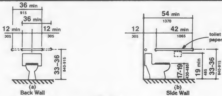
Fig. 29 Grab Bars at Water Closets
