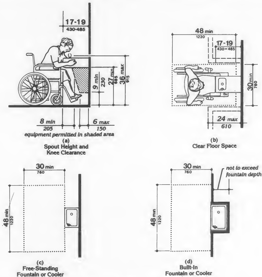
Fig. 27 Drinking Fountains and Water Coolers
