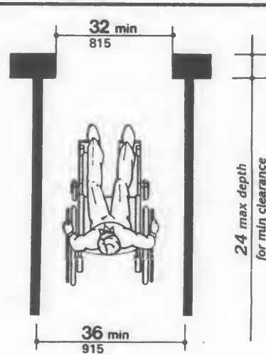
Fig. 1 Minimum Clear Width for Single Wheelchair
