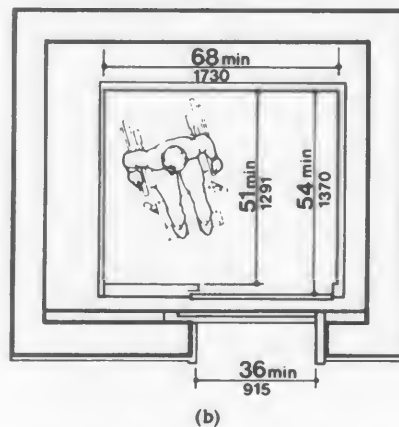
Fig. 22 Minimum Dimensions of Elevator Cars
