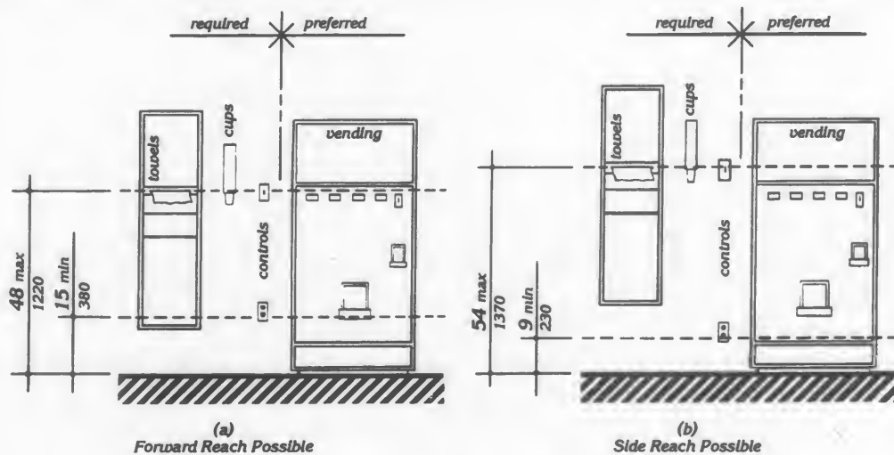
Fig. A8 Control Reach Limitations
