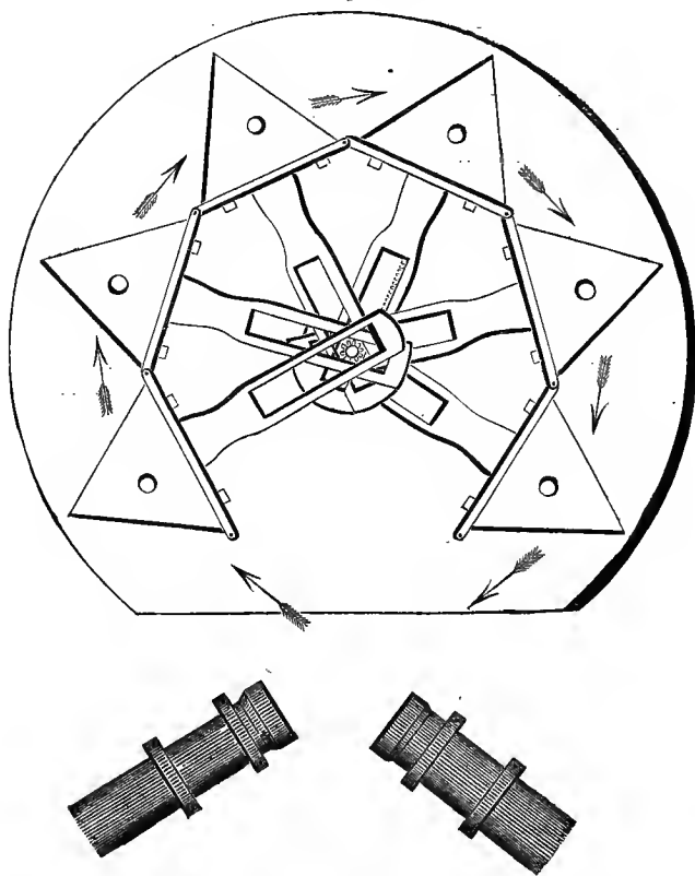
FIG. 10.—Rutherford's Automatic Spectroscope.
