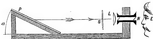
FIG. 11.—Simple Polarizing Apparatus.
