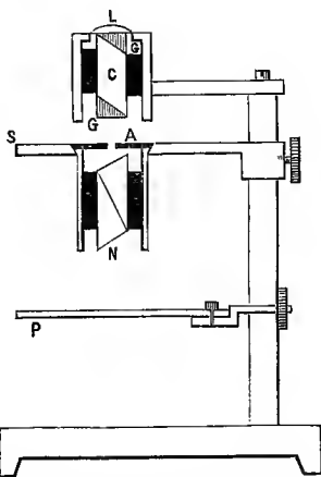
FIG. 65.—The Schistoscope, for the production of Complementary Colours. (Brücke)
