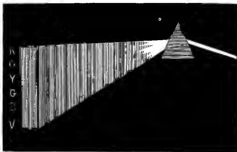
FIG. 1.—Prismatic Spectrum.
