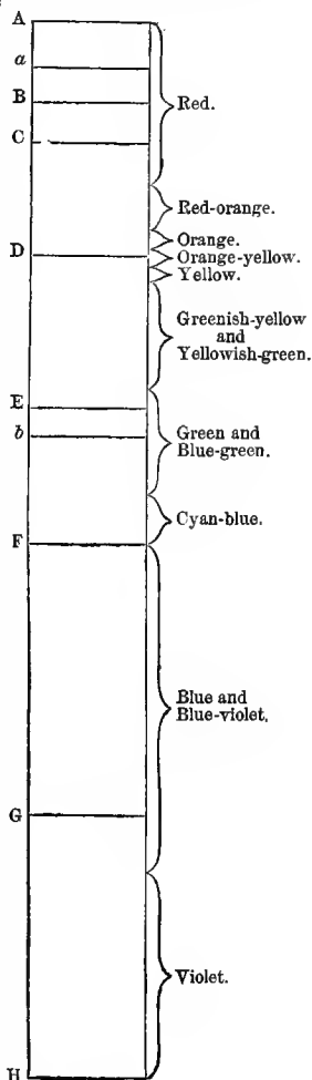
Fig. 46.—Prismatic Spectrum.
