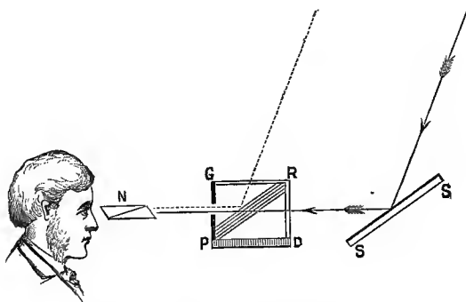
FIG. 57.—The Dichroöscope as arranged for use.
