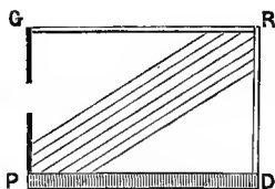
FIG. 56.—The Dichroöscope shown in section.
