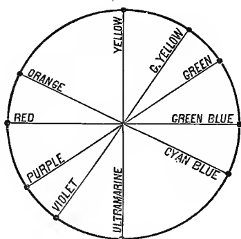
FIG. 118.—Chromatic Circle.
