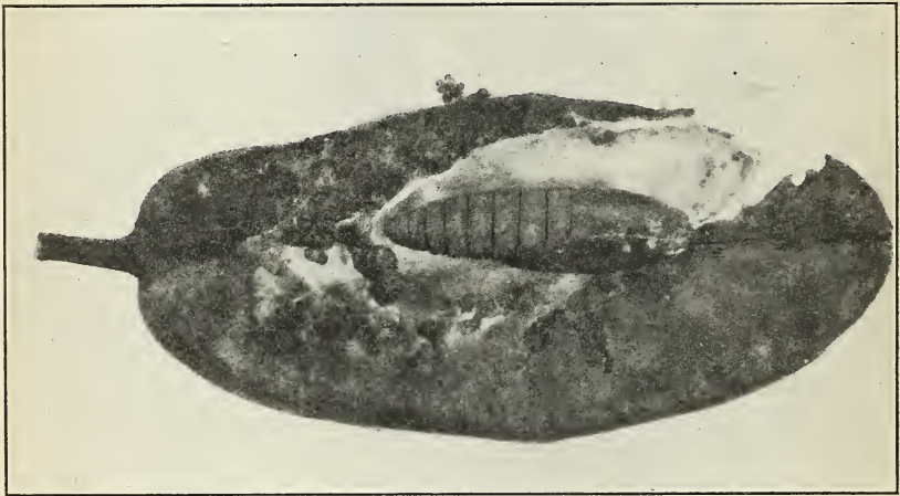
FIG. 8.—The blackhead fireworm: View of pupa and interior of cocoon. Enlarged about 7.5 times.
