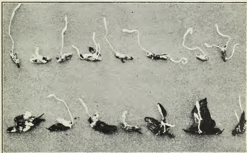
FIG. 11.—Fungous disease, a species of Spicaria , growing from the blackhead fireworm pupæ in their cocoons. Slightly enlarged.
