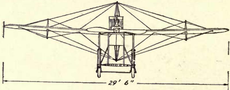
SIDE ELEVATION, PLAN AND FRONT ELEVATION OF THE TELLIER MONOPLANE
