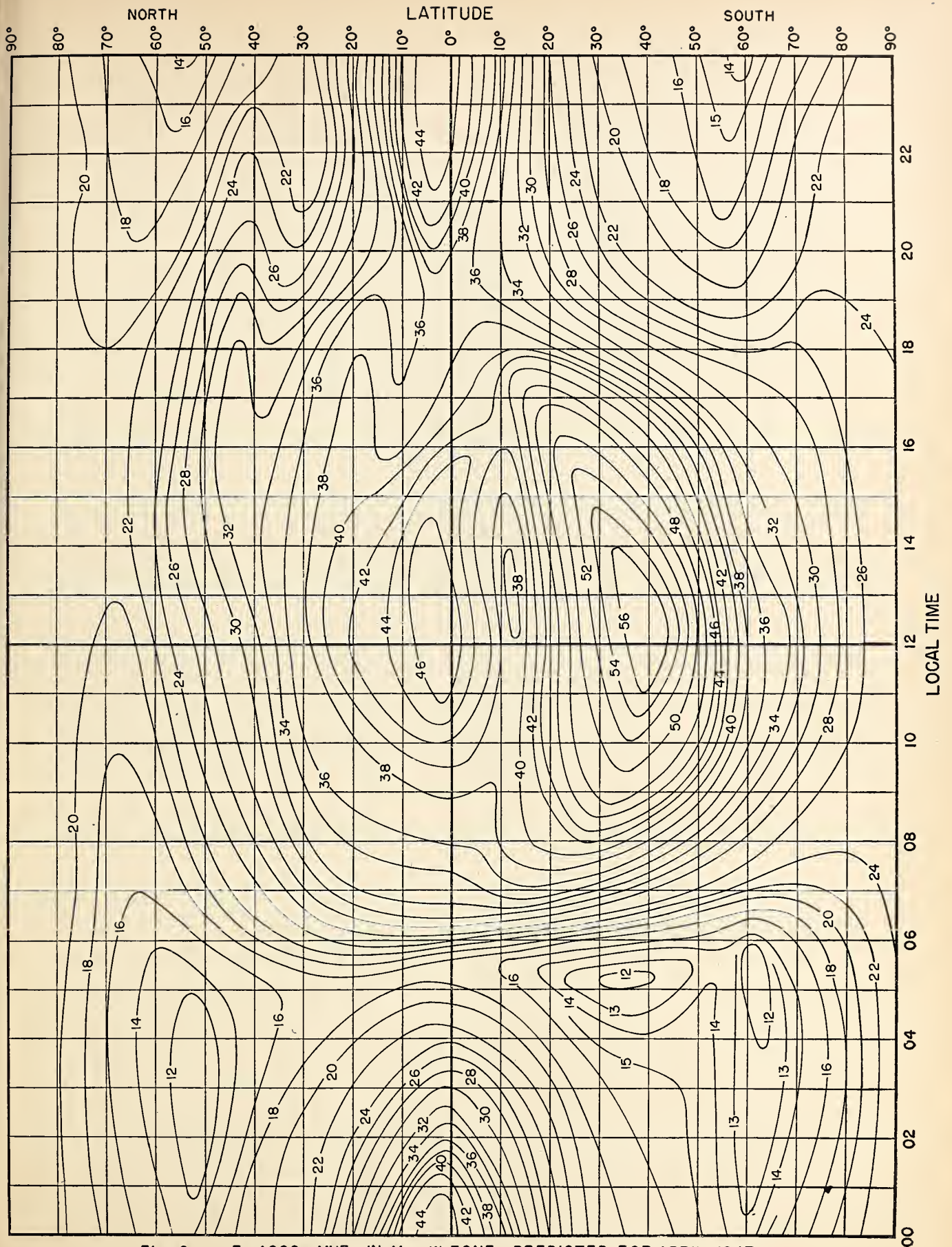
Fig. 6. F_2 4000-MUF, IN Mc, W ZONE, PREDICTED FOR APRIL 1947
