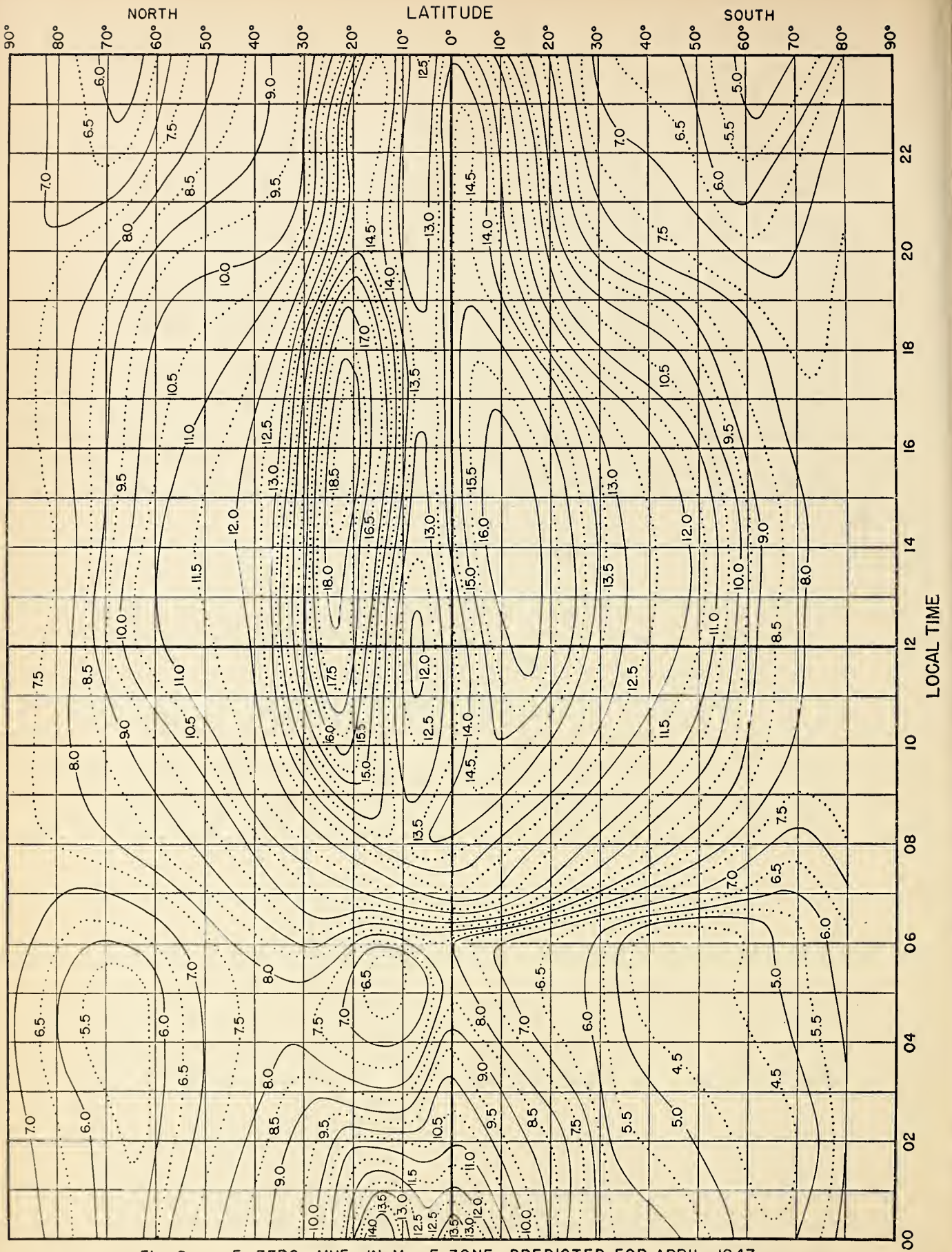
Fig. 9. F 2 ZERO - MUF, IN Mc, E ZONE, PREDICTED FOR APRIL 1947
