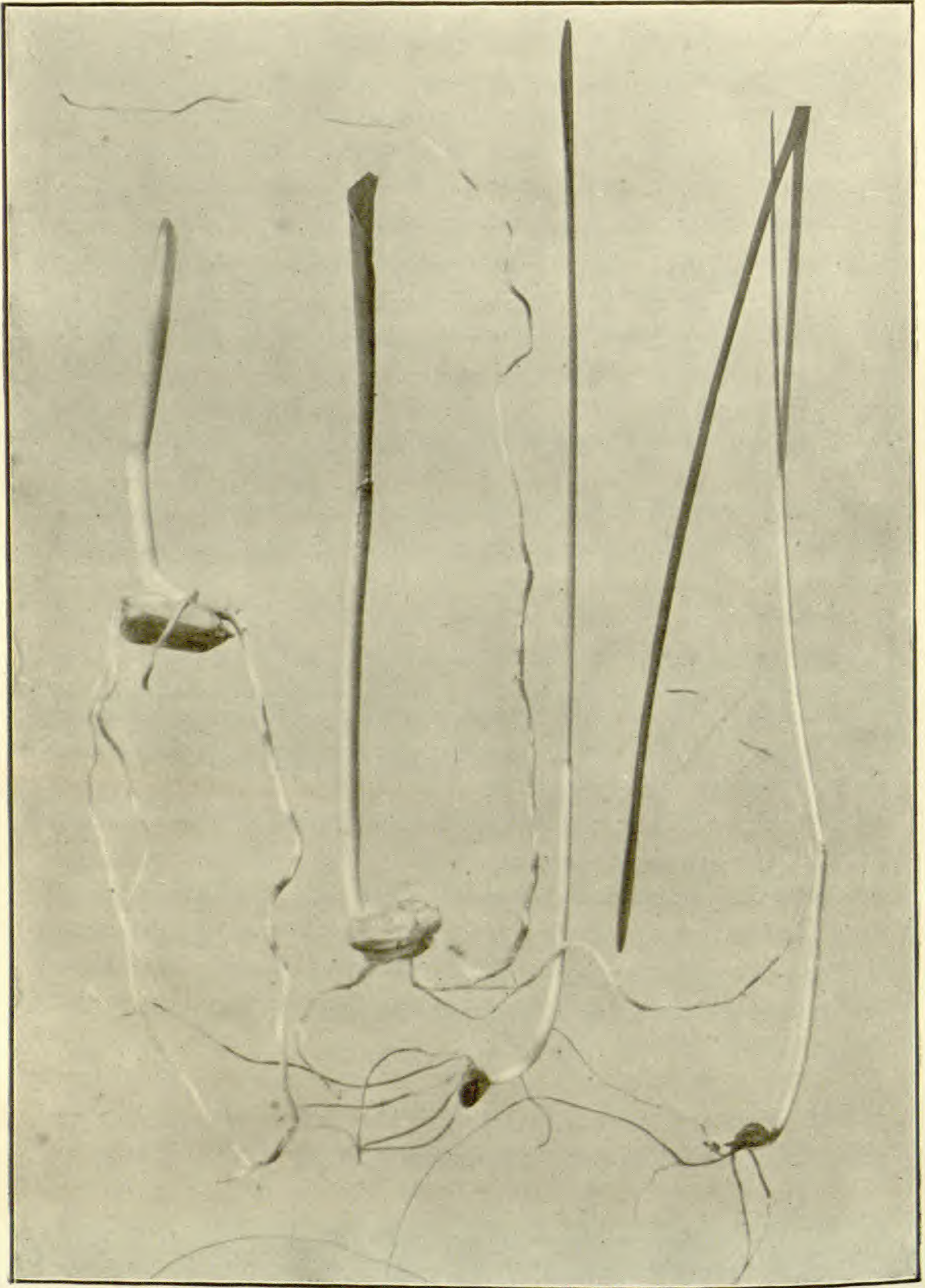
FIG. 4.—Corn and wheat seedlings. The larger one in each case is normal, while the smaller ones were from seeds treated eight months with gas from 0.333^{\text{gm}} KCN per cubic foot.
