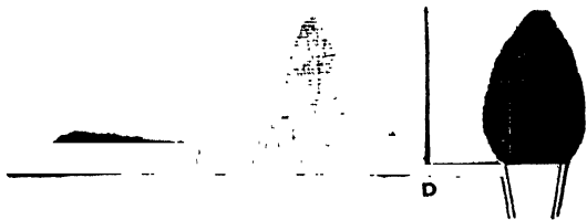
Flame of carbonic oxide burning in oxygen at 60 mm. pressure, with spectrum showing maxima. The continuous spectrum at the bottom is given by the red-hot top of the glass jet.
