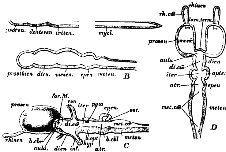
FIG. 2.—Diagrams showing three chief stages in the development of the nervous system. A, the neuron is divided into myelon and encephalon, the latter being again divided into the three primary vesicles. protencephalon , deuterencephalon , and tritencephalon . Similarly, the neurocaele , or general cavity of the neuron, is divided into myelocaele and encephalocaele , and the latter, again, into proso-caeles , and trito-caeles . B, the brain now consists of five encephalomereres, the prosthio- , dia- , meso- , epi- , and meta-encephala , containing respectively the prosthio- , dia- , meso- , epi- , and meta-caeles . C, D, the brain has assumed its permanent form, and is shown in C in vertical, in D in horizontal section. The prosthioencephalon has sent out paired prosencephala , a small unpaired portion, the basocerebrum ( b.cbr. ), being left, the latter being bounded in front by the lamina terminalis ( lam. term. ). Each prosencephalon has further given rise to a rhinencephalon . Similarly, the prosthio-caele now consists of unpaired aulu and of paired proso and rhino-caeles ( prae. cae. , rh. cae. ), the former communicating with the aulu by the foramina of Monro , or portae ( for. M. ). The diacaele is continued above into the conarium ( con ), below into the infundibulum ( inf ) with the hypophysis ( hyp ). The mesencephalon consists of an unpaired ventral basiopticus ( b. opt. ), and of paired opticocephala : its cavity of a median iter , and of paired optico-caeles , which communicate with the iter by the pyla . The epencephalon is divided into a dorsal portion, the cerebellum, or epencephalon proper, and a ventral division, the basio-cerebellum ( b. cbl. ), containing a cavity, the atrium ( atr. ), which communicates with the epicaele proper, or cavity of the cerebellum, by the ostium ( ost. ). The metencephalon and metacaele ( met. cae. ) have undergone but little alteration.
