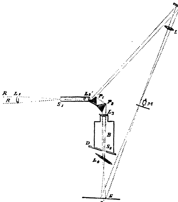
FIG. 1.—Colour Photometer.
