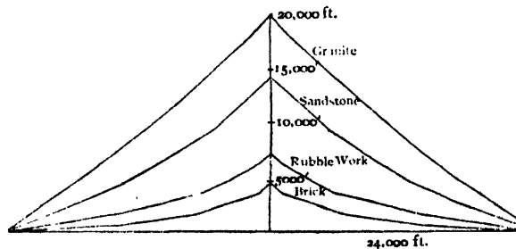
FIG. 2.—Theoretical Mountains.
